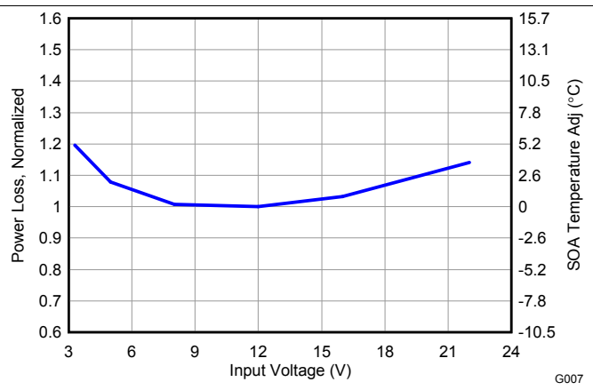
Figure 7. Normalized Power Loss vs Input Voltage
