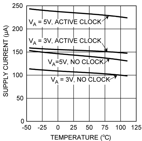
5-26. Supply Current vs Temperature
