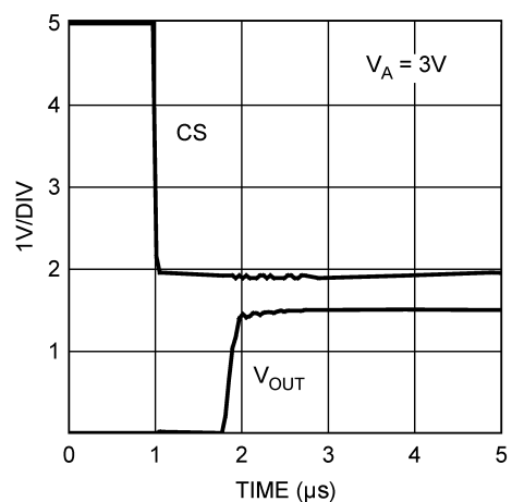
5-29. 3V Wake-Up Time
