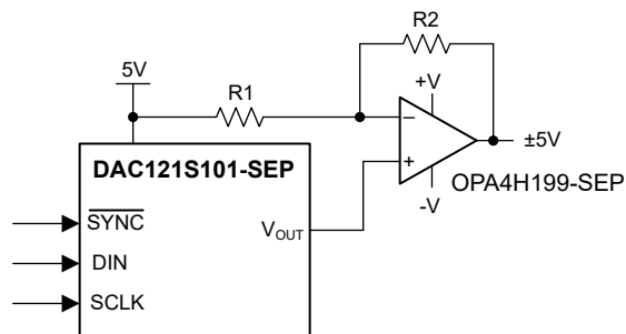
図 7-1. Bipolar Operation
