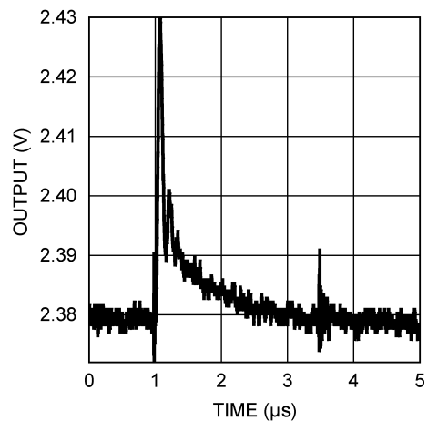
5-27. 5V Glitch Response
