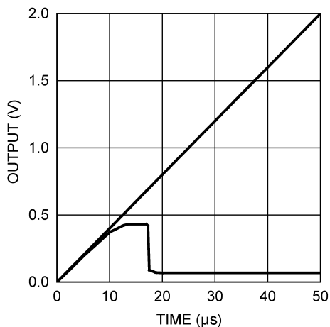
5-28. Power-On Reset
