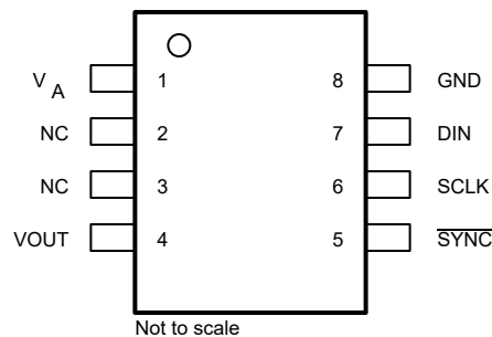
図 4-1. DAC121S101-SEP DGK Package, 8-Pin VSSOP (Top View)
