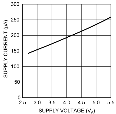
5-25. Supply Current vs Supply Voltage
