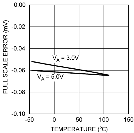
5-24. Full-Scale Error vs Temperature
