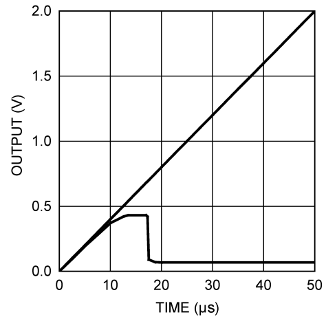
Figure 27. Power-On Reset
