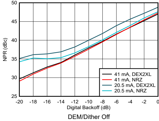
FIG 6-195. Noise Power Ratio vs Digital Backoff: 1 st Nyquist Zone
