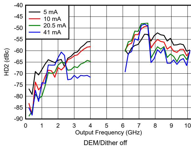
Figure 6-143. HD2 vs Frequency and Output Current in DES2X Modes
