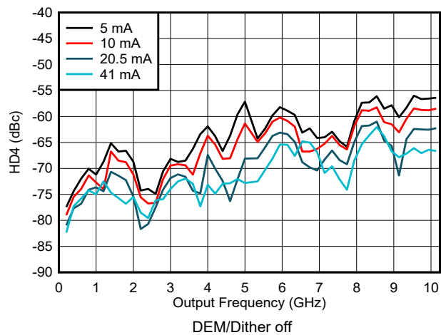
Figure 6-173. HD4 vs Frequency and Output Current in NRZ/RF Modes
