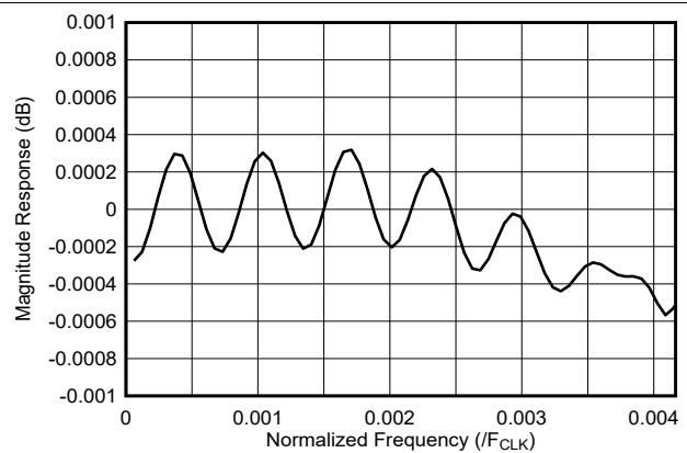
7-37. 96x Interpolation Filter Passband Response
