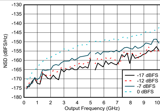
FIG 6-66. NSD vs Output Frequency and Digital Amplitude
