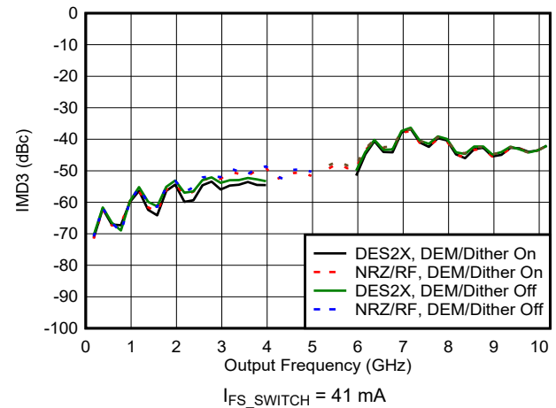
図 6-92. IMD3 vs Frequency and Mode
