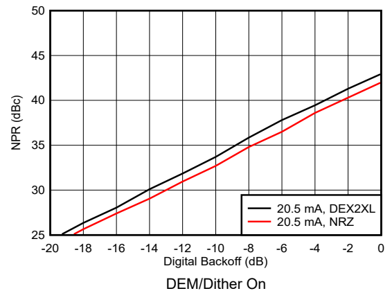
FIG 6-198. Noise Power Ratio vs Digital Backoff: 2 nd Nyquist Zone
