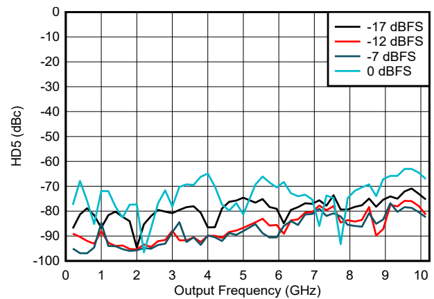
FIG 6-184. HD5 vs Frequency and Digital Amplitude in NRZ/RF Modes
