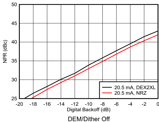
FIG 6-197. Noise Power Ratio vs Digital Backoff: 2 nd Nyquist Zone
