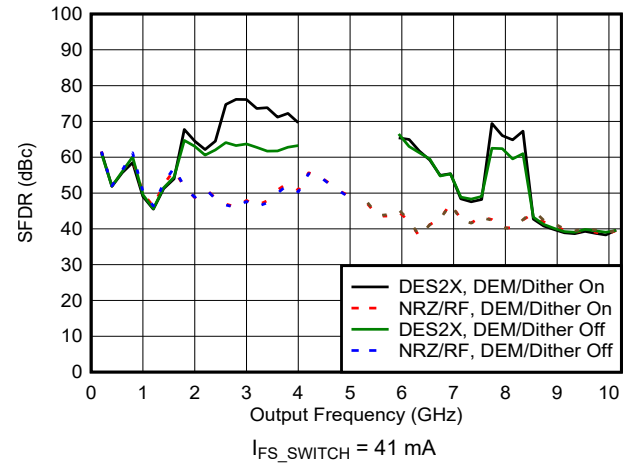
図 6-90. SFDR vs Frequency and Mode
