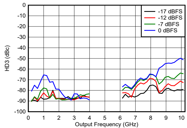
FIG 6-166. HD3 vs Frequency and Digital Amplitude in DES2X Modes
