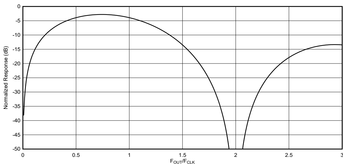
図 7-8. RF Mode Output Frequency Response
