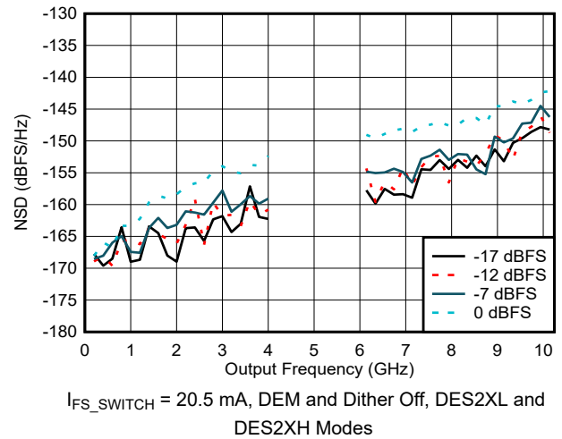
Figure 6-71. NSD vs Output Frequency and Digital Amplitude
