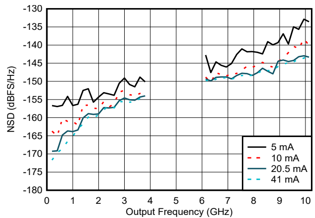
FIG 6-63. NSD vs Output Frequency and Output Current
