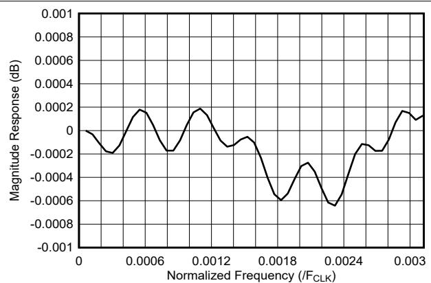
7-39. 128x Interpolation Filter Passband Response
