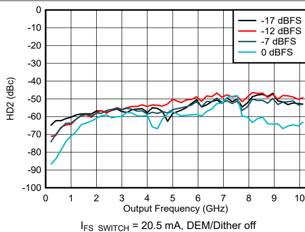
Figure 6-145. HD2 vs Frequency and Digital Amplitude in NRZ/RF Modes
