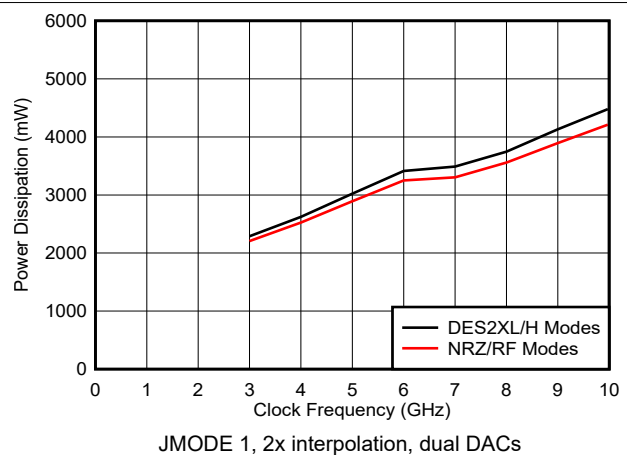
6-214. Power Dissipation vs Clock Frequency and DAC Mode
