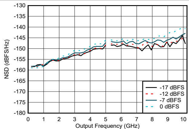
FIG 6-65. NSD vs Output Frequency and Digital Amplitude
