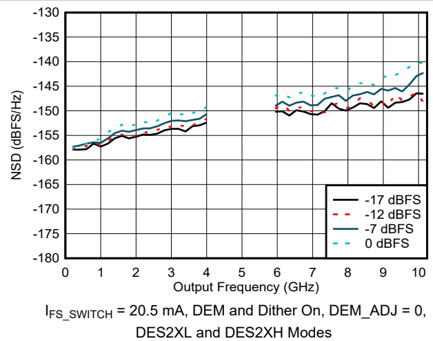
Figure 6-73. NSD vs Output Frequency and Digital Amplitude
