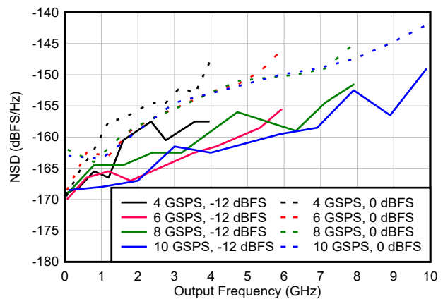
Figure 6-77. NSD vs Output Frequency and Sample Rate
