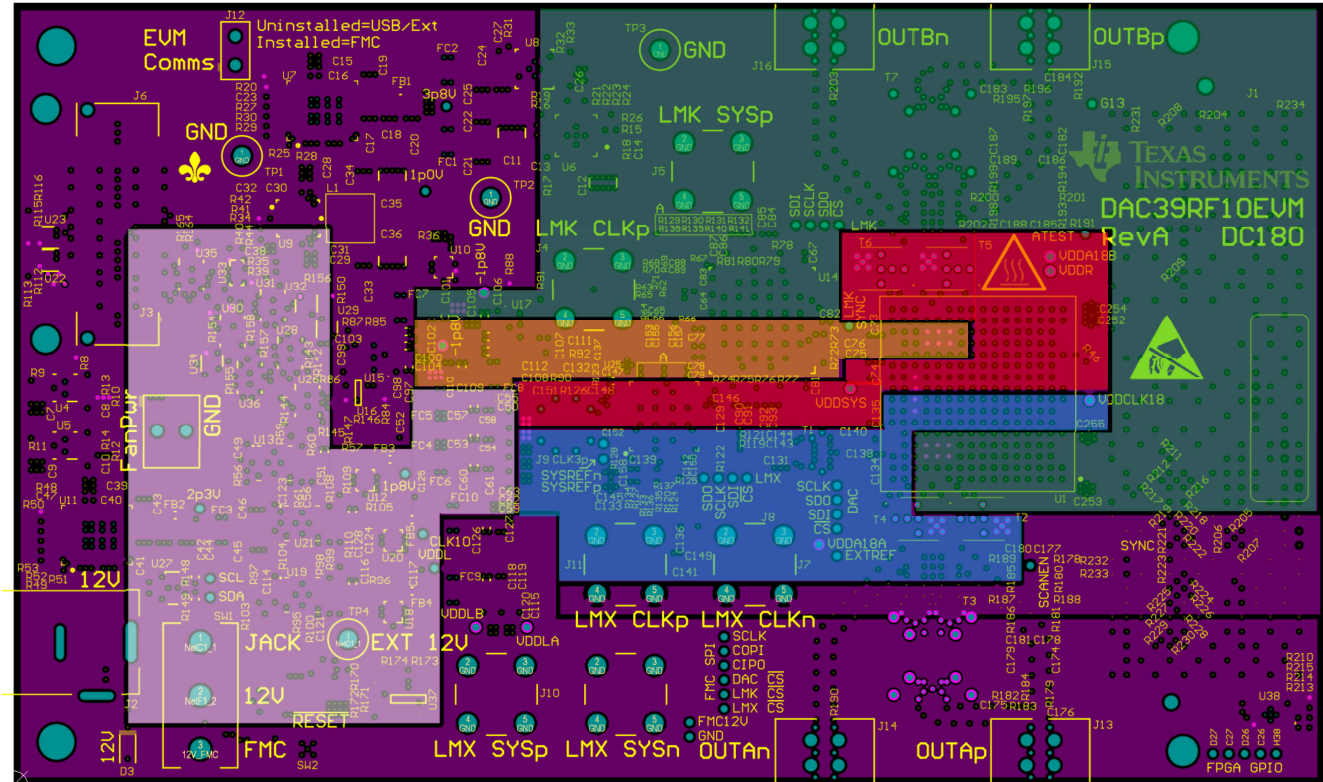
Layer12 / PWR3 DAC VDDA18A = RED DAC VDDA18B = ORANGE DAC VDDDB = YELLOW DAC VEExA = GREEN DAC VEExB = BLUE VDDIO = WHITE
