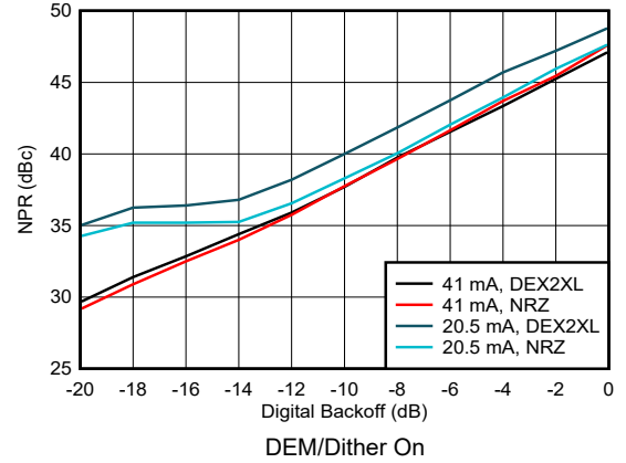
FIG 6-196. Noise Power Ratio vs Digital Backoff: 1 st Nyquist Zone
