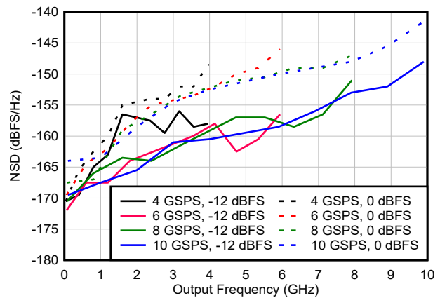
Figure 6-75. NSD vs Output Frequency and Digital Amplitude
