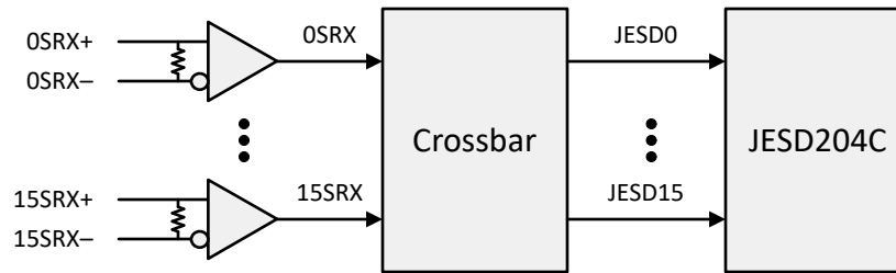
FIG 7-53. Crossbar Block Diagram
