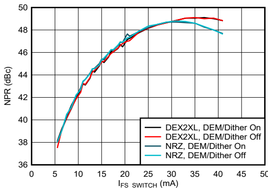
FIG 6-199. Noise Power Ratio vs Output Current: 1 st Nyquist Zone
