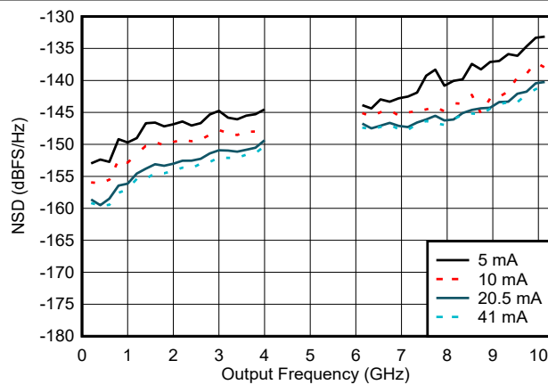
FIG 6-62. NSD vs Output Frequency and Output Current
