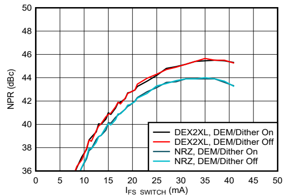
FIG 6-200. Noise Power Ratio vs Output Current: 2 nd Nyquist Zone
