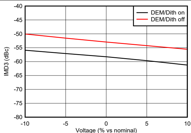
図 6-139. IMD3 vs Voltage in RF Mode at 7247 MHz
