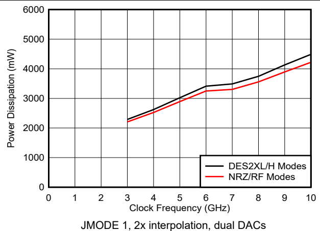
6-214. Power Dissipation vs Clock Frequency and DAC Mode
