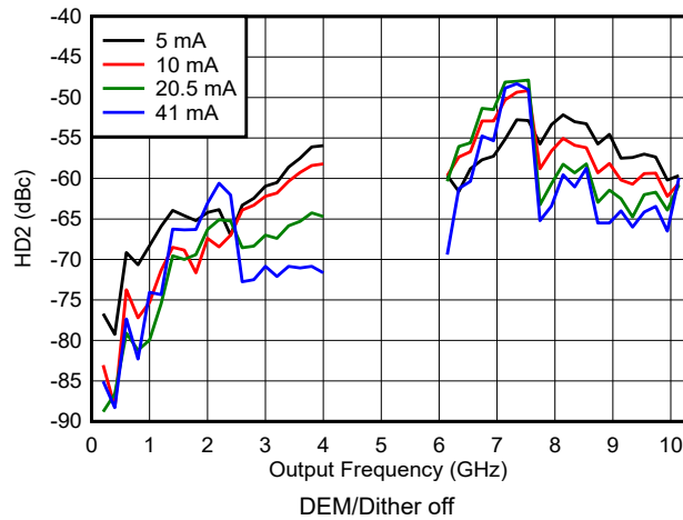
图 6-143. HD2 vs Frequency and Output Current in DES2X Modes
