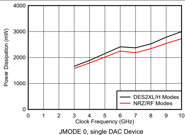
6-213. Power Dissipation vs Clock Frequency and DAC Mode
