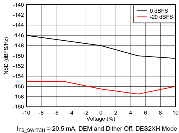
図 6-88. NSD vs Supply Voltage
