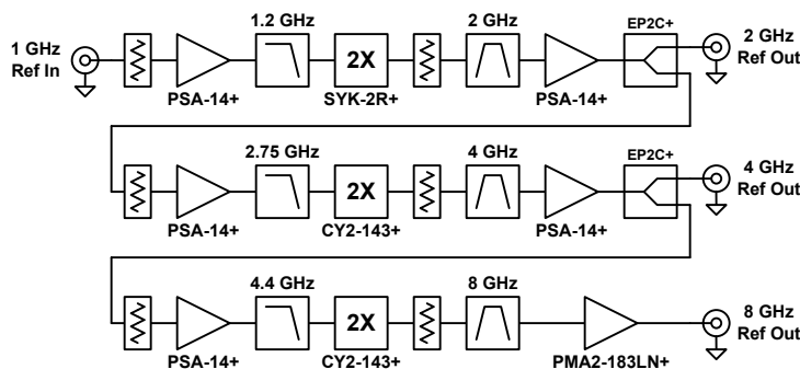
Figure 8-11. Reference Multiplier Chain
