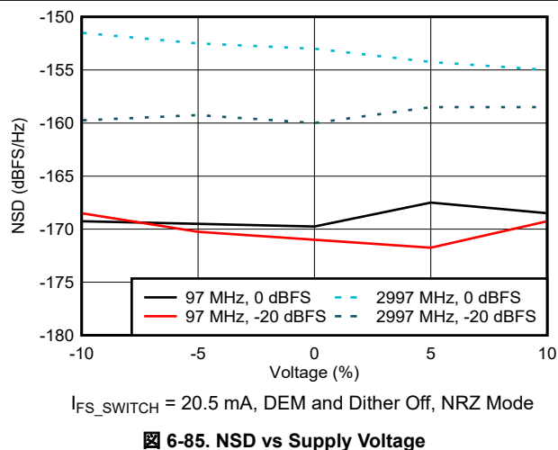
図 6-85. NSD vs Supply Voltage
