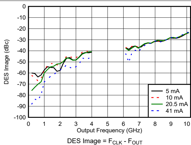
FIG 6-193. DES Image vs Frequency and Output Current in DES2X Modes
