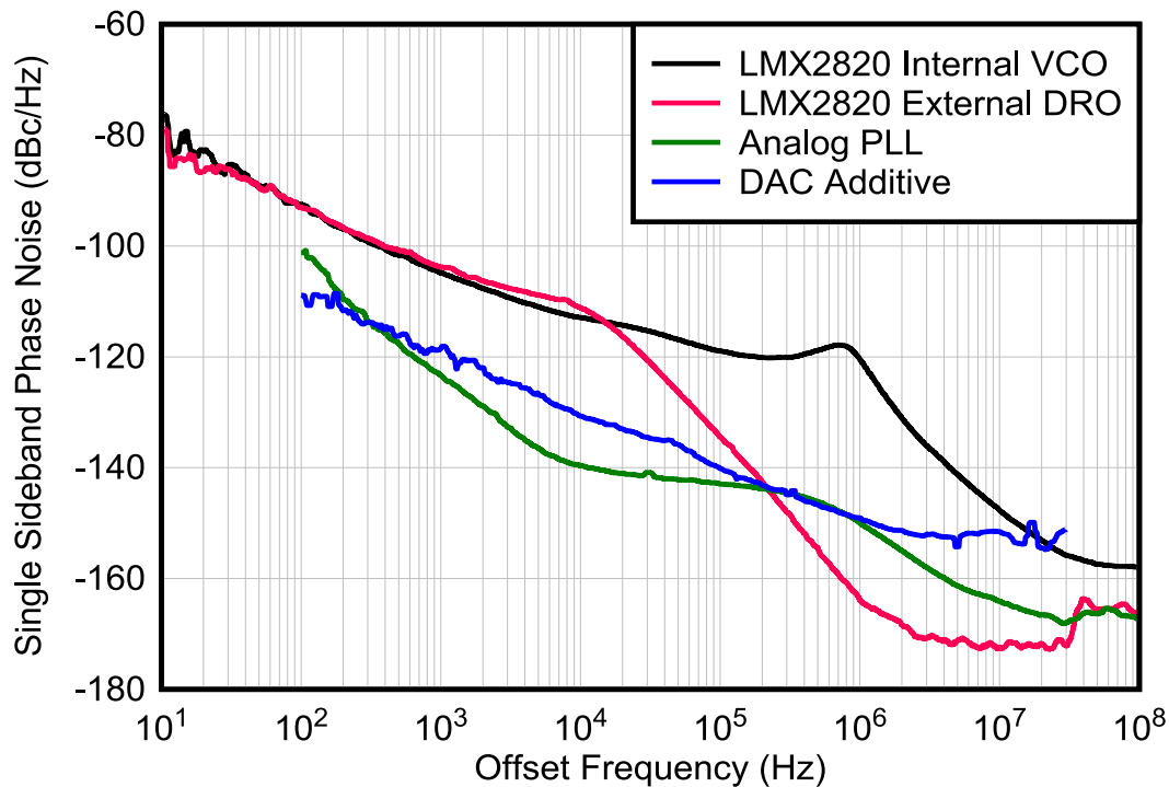
図 8-7. Phase Noise of DAC Clock Examples with the Device Additive Phase Noise
