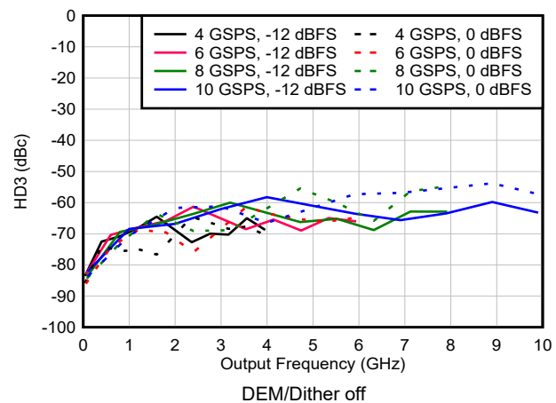
FIG 6-170. HD3 vs Frequency and Sample Rate in NRZ/RF Modes
