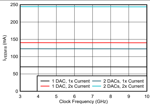
図 6-218. VEEM18 Current vs Clock Frequency and DAC Mode
