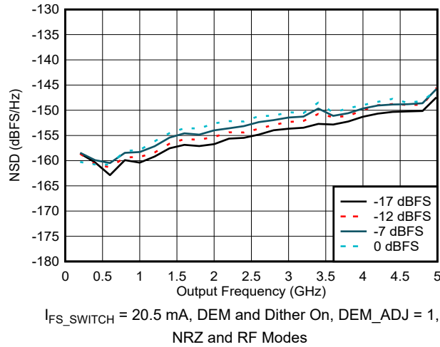
FIG 6-68. NSD vs Output Frequency and Digital Amplitude
