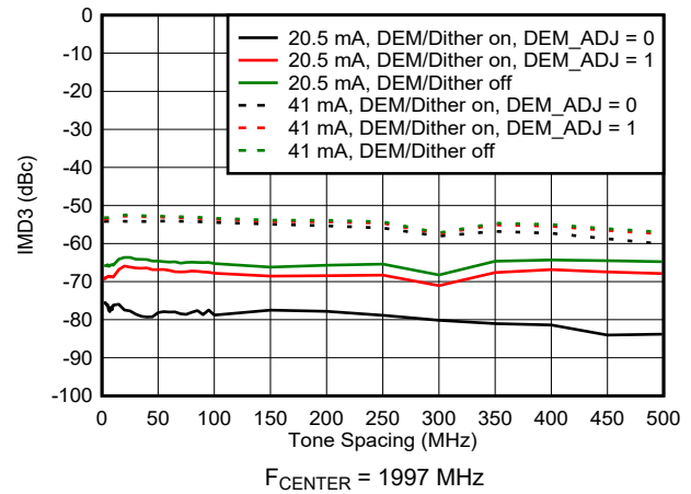
6-126. IMD3 vs Tone Spacing in DES2XL Mode
