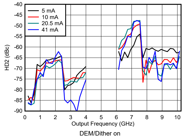
图 6-144. HD2 vs Frequency and Output Current in DES2X Modes
