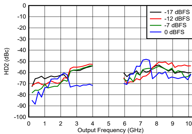
FIG 6-149. HD2 vs Frequency and Digital Amplitude in DES2X Modes
