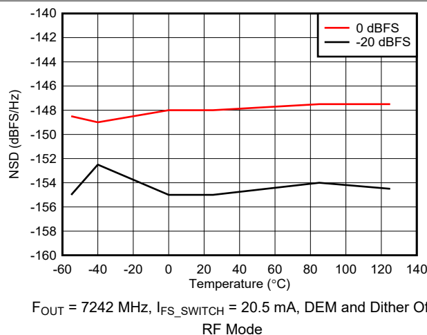
図 6-82. NSD vs Temperature
