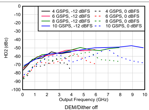
図 6-154. HD2 vs Frequency and Sample Rate in NRZ/RF Modes
