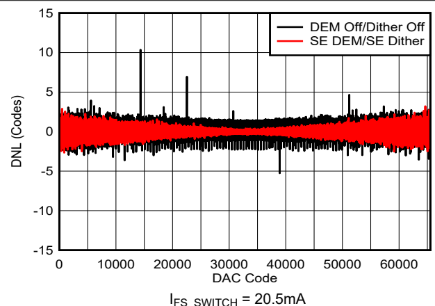
図 6-11. DNL vs DAC Code: 20.5mA
