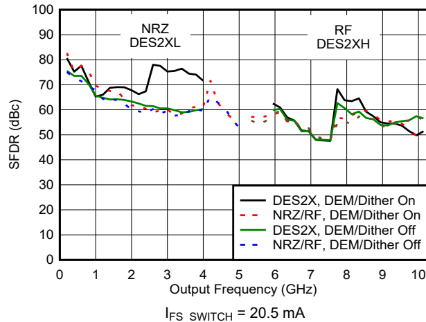
図 6-89. SFDR vs Frequency and Mode
