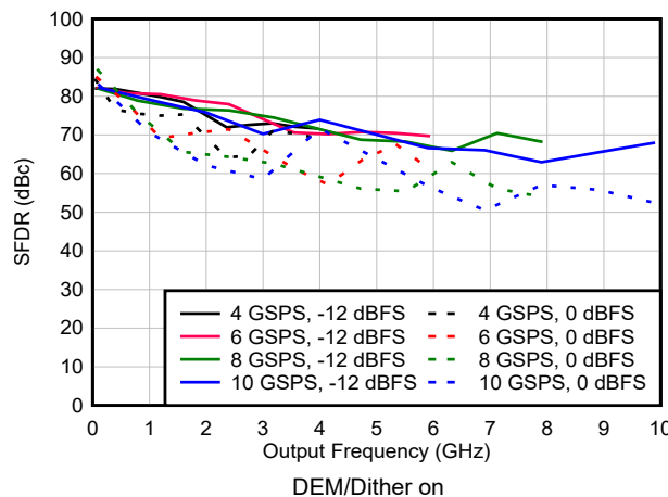
6-109. SFDR vs Frequency and Sample Rate in NRZ/RF Modes
