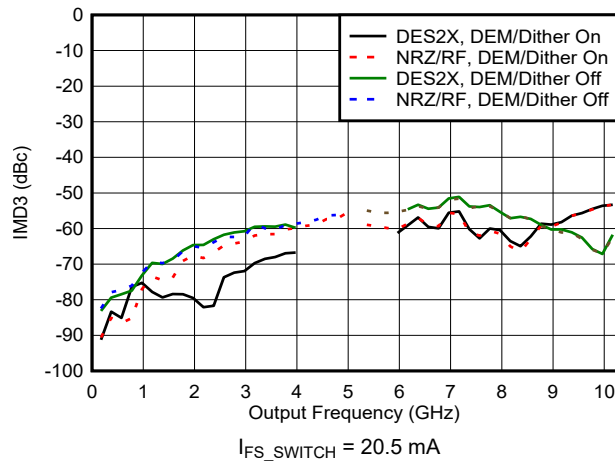
図 6-91. IMD3 vs Frequency and Mode
