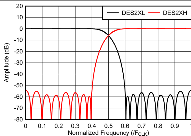
図 7-48. DES Interpolator Frequency Response
