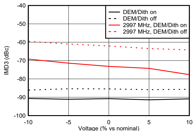
図 6-137. IMD3 vs Voltage in NRZ Mode
