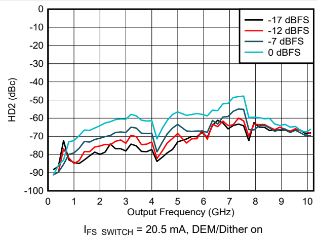
图 6-146. HD2 vs Frequency and Digital Amplitude in NRZ/RF Modes
