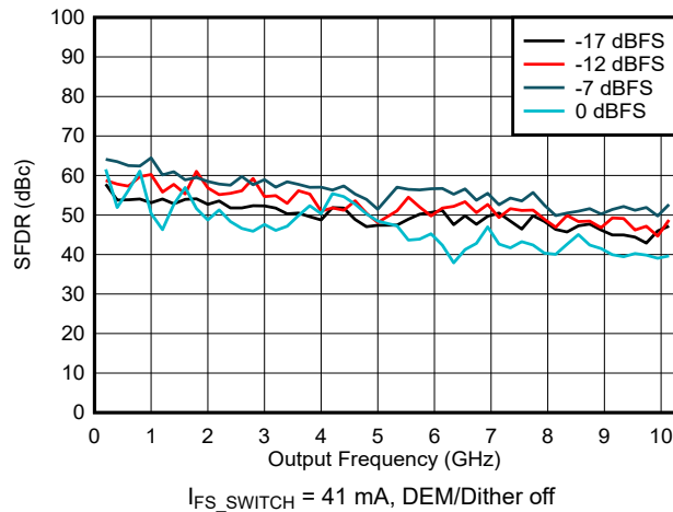
Figure 6-103. SFDR vs Frequency and Digital Amplitude in NRZ/RF Modes
