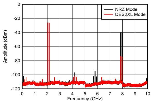
图 6-46. Dual Tone, f_{\text{OUT}} = 2097\text{ MHz} , 0 dBFS
