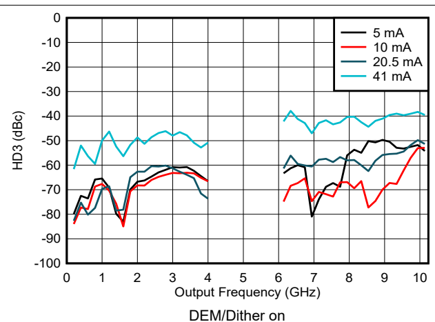
図 6-158. HD3 vs Frequency and Output Current in NRZ/RF Modes
