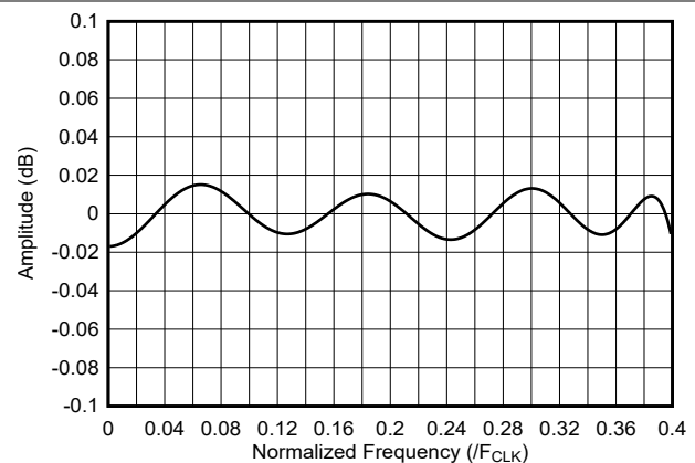
図 7-49. DES Interpolator Frequency Response (Passband)
