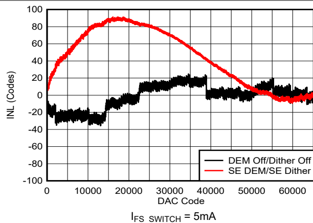
图 6-14. INL vs DAC Code: 5mA
