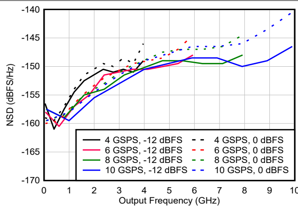
Figure 6-76. NSD vs Output Frequency and Digital Amplitude
