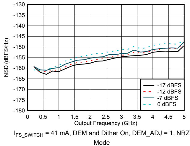
FIG 6-70. NSD vs Output Frequency and Digital Amplitude
