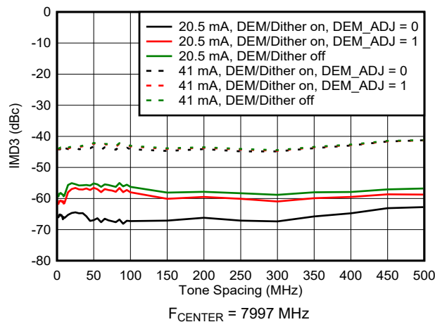
6-127. IMD3 vs Tone Spacing in RF Mode
