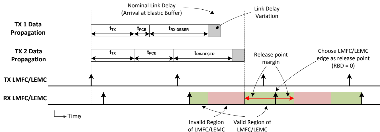
图 7-54. LMFC Valid Region Definition for Elastic Buffer Release Point Selection
