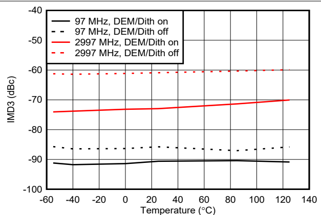
图 6-134. IMD3 vs Temperature in DES2XL Mode
