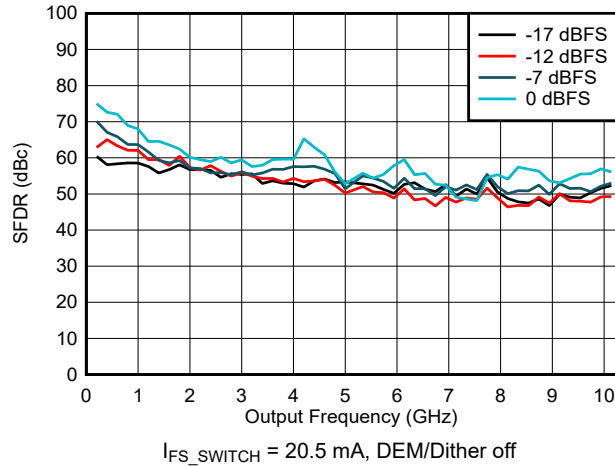
Figure 6-101. SFDR vs Frequency and Digital Amplitude in NRZ/RF Modes
