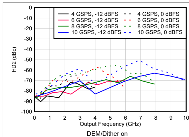
図 6-153. HD2 vs Frequency and Sample Rate in NRZ/RF Modes
