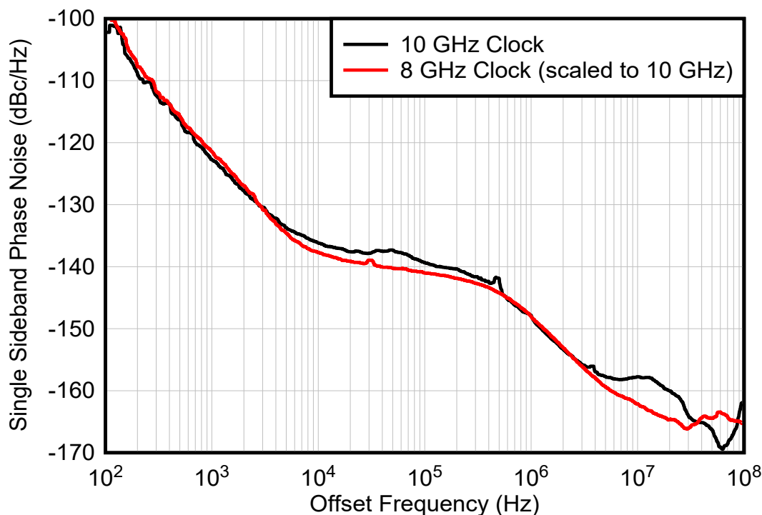
図 8-13. 8 GHz and 10 GHz Clock Phase Noise
