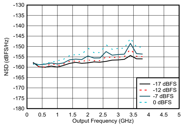
Figure 6-75. NSD vs Output Frequency and Digital Amplitude
