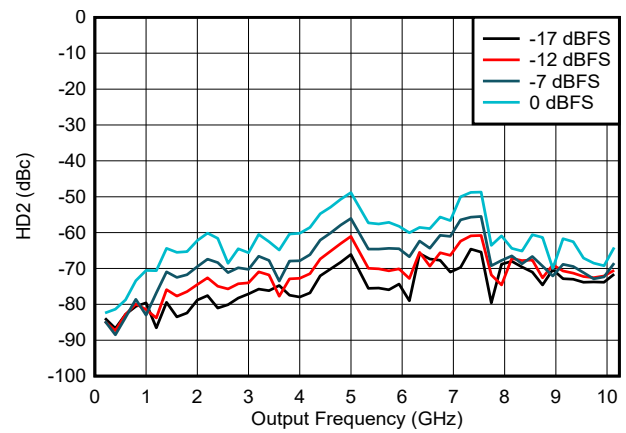
FIG 6-148. HD2 vs Frequency and Digital Amplitude in NRZ/RF Modes
