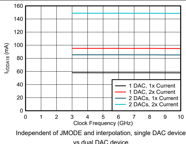
6-216. VDDA18 Current vs Clock Frequency and DAC Mode
