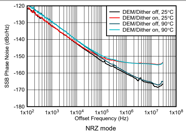
图 6-204. Phase Noise vs Offset Frequency at 1 GHz
