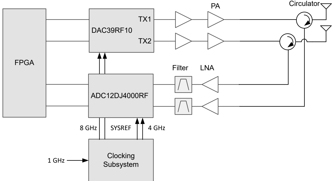
図 8-6. Two Channel Radar Transceiver using DAC39RF10 and ADC12DJ4000RF
