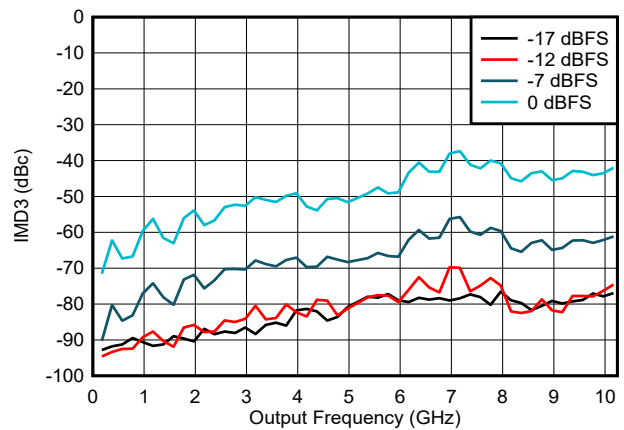
FIG 6-118. IMD3 vs Frequency and Digital Amplitude in NRZ/RF Modes
