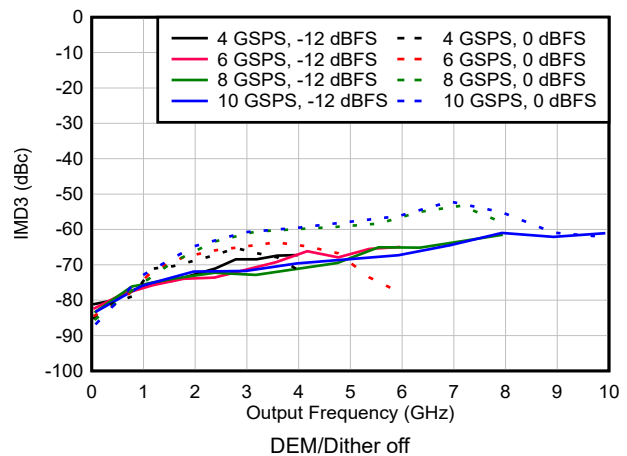
图 6-132. IMD3 vs Frequency and Sample Rate in DES2X Modes
