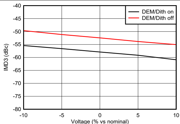
図 6-140. IMD3 vs Voltage in DES2XH Mode at 7247 MHz
