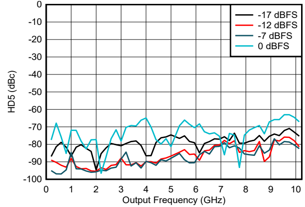
Figure 6-184. HD5 vs Frequency and Digital Amplitude in NRZ/RF Modes
