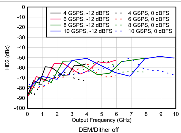
図 6-156. HD2 vs Frequency and Sample Rate in DES2X Modes
