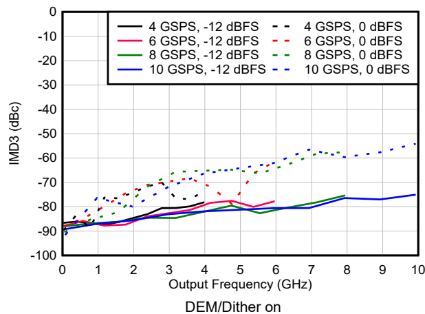
图 6-131. IMD3 vs Frequency and Sample Rate in DES2X Modes
