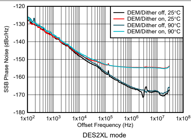
图 6-205. Phase Noise vs Offset Frequency at 1 GHz
