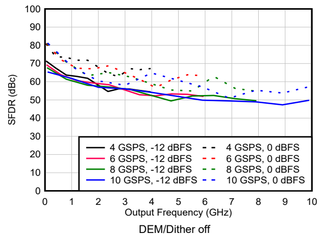
6-110. SFDR vs Frequency and Sample Rate in NRZ/RF Modes
