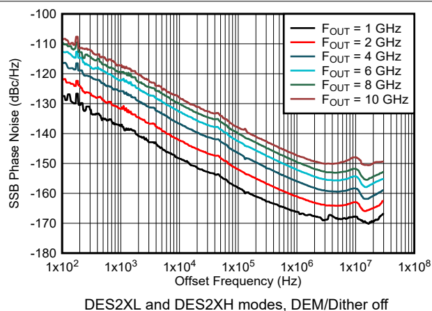
图 6-203. Phase Noise vs Offset Frequency and Output Frequency
