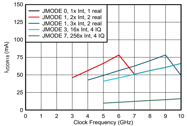
图 6-222. VDDR18 Current vs Clock Frequency and Mode
