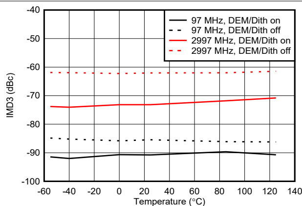
图 6-133. IMD3 vs Temperature in NRZ Mode
