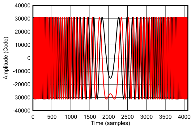
図 8-15. Complex Time Domain of NLFM Chirp (Red = real, Black = imag)
