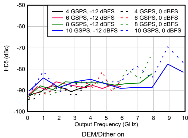
FIG 6-189. HD5 vs Frequency and Sample Rate in NRZ/RF Modes
