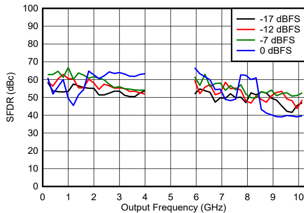
6-105. SFDR vs Frequency and Digital Amplitude in DES2X Modes
