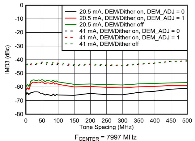
6-128. IMD3 vs Tone Spacing in DES2XH Mode
