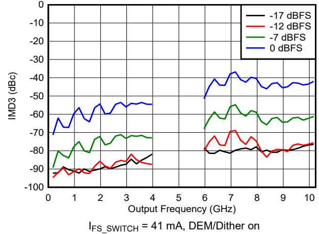
6-124. IMD3 vs Frequency and Digital Amplitude in DES2X Modes
