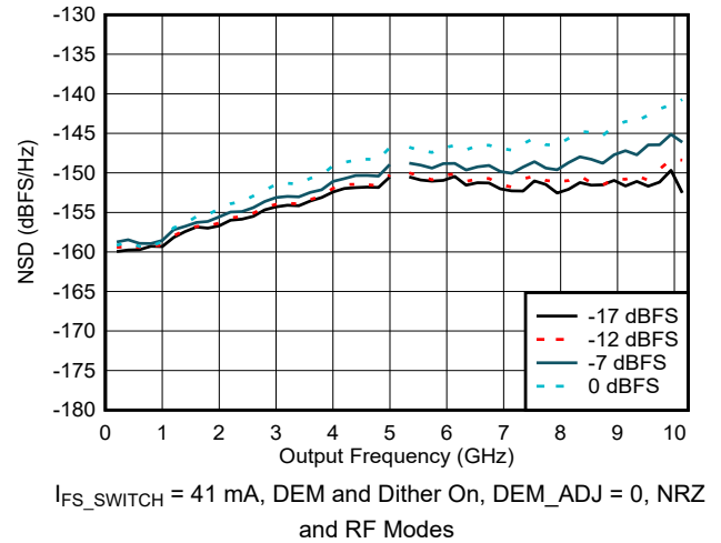
FIG 6-69. NSD vs Output Frequency and Digital Amplitude
