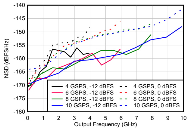
Figure 6-75. NSD vs Output Frequency and Digital Amplitude
