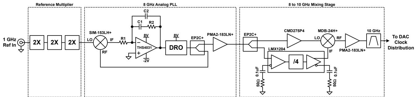
8-12. 10 GHz Clock Synthesizer
