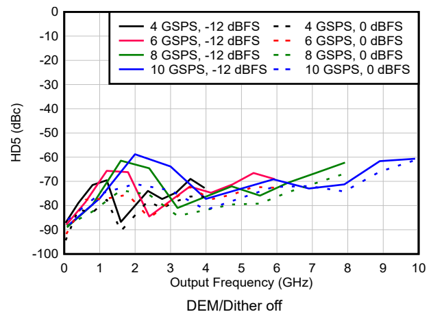
FIG 6-192. HD5 vs Frequency and Sample Rate in DES2X Modes
