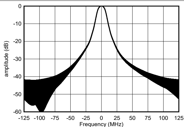
図 8-16. Digital Spectrum for NLFM Chirp
