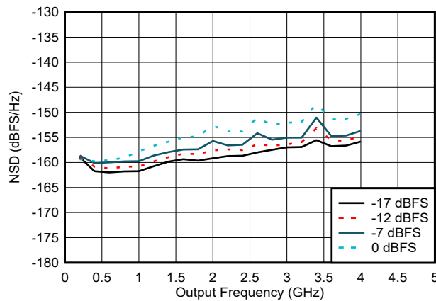
Figure 6-74. NSD vs Output Frequency and Digital Amplitude
