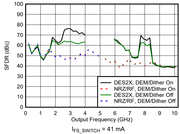
図 6-90. SFDR vs Frequency and Mode
