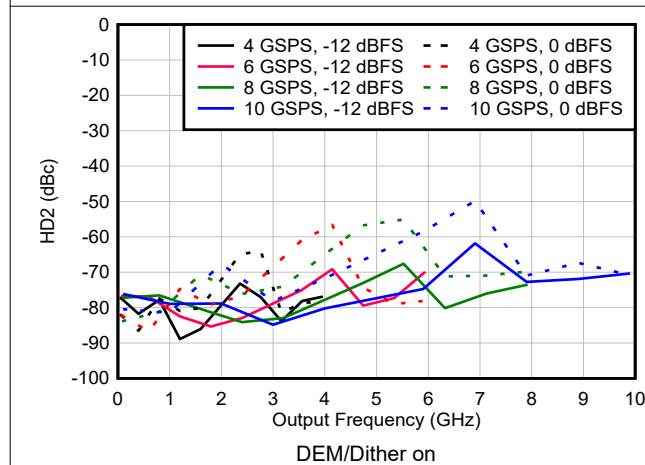
図 6-155. HD2 vs Frequency and Sample Rate in DES2X Modes
