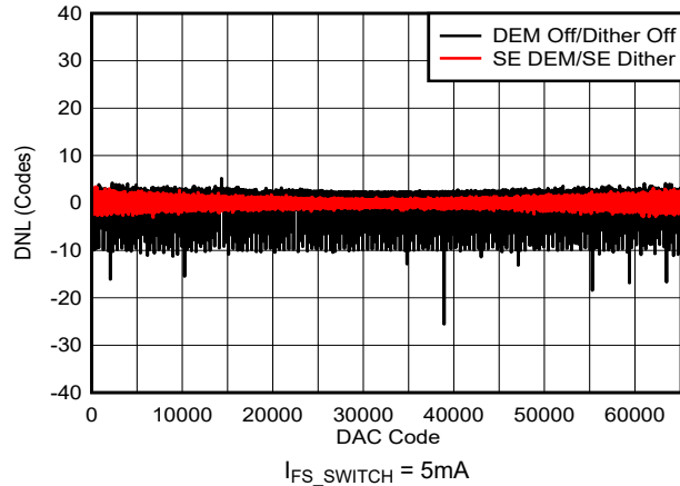
图 6-12. DNL vs DAC Code: 5mA
