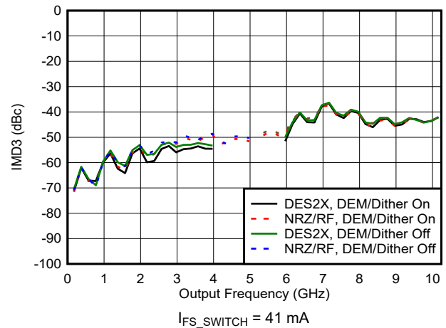
図 6-92. IMD3 vs Frequency and Mode
