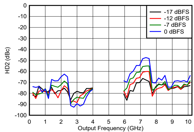
FIG 6-150. HD2 vs Frequency and Digital Amplitude in DES2X Modes
