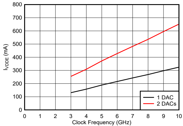
图 6-221. VDDE Current vs Clock Frequency
