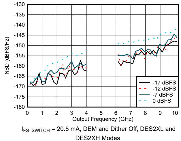
FIG 6-71. NSD vs Output Frequency and Digital Amplitude
