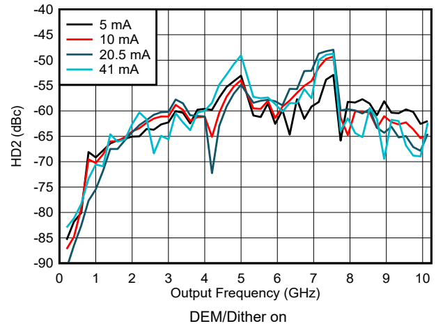
图 6-142. HD2 vs Frequency and Output Current in NRZ/RF Modes
