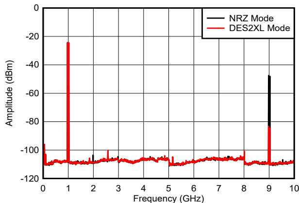
图 6-43. Dual Tone, f_{\text{OUT}} = 997\text{ MHz} , 0 dBFS
