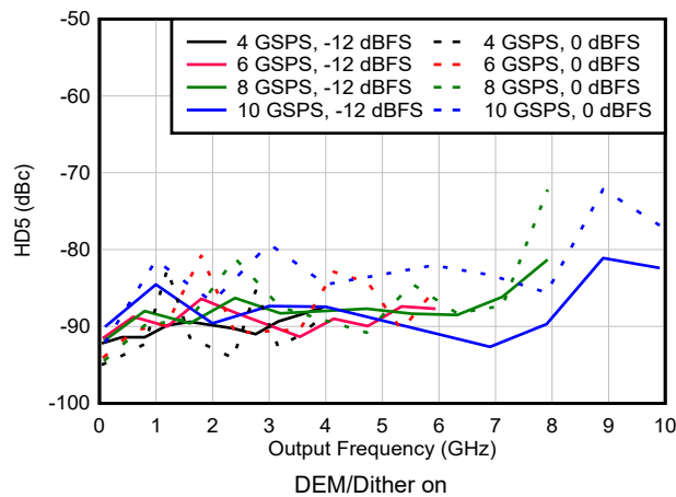
FIG 6-191. HD5 vs Frequency and Sample Rate in DES2X Modes
