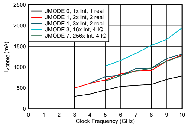
图 6-224. VDDDIG Current vs Clock Frequency and Digital Mode
