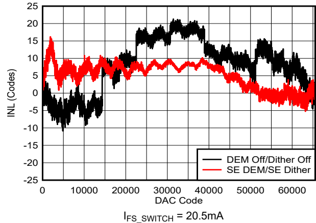
图 6-13. INL vs DAC Code: 20.5mA
