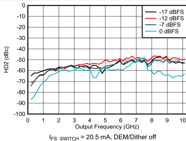
图 6-145. HD2 vs Frequency and Digital Amplitude in NRZ/RF Modes
