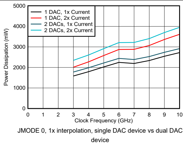
6-215. Power Dissipation vs Clock Frequency and DAC Mode
