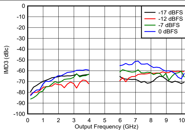
FIG 6-119. IMD3 vs Frequency and Digital Amplitude in NRZ/RF Modes
