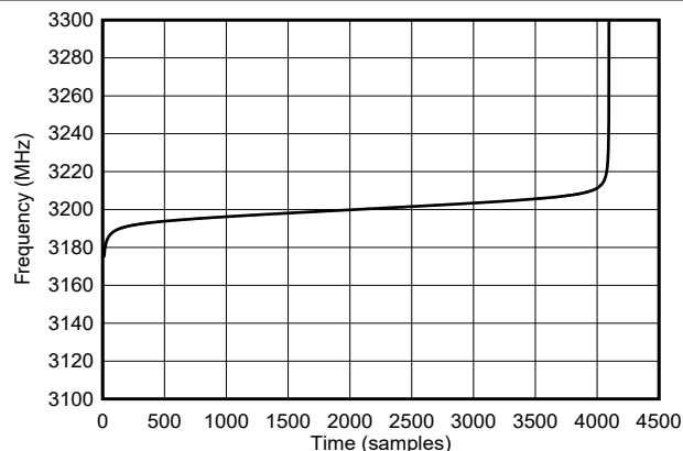
図 8-14. NLFM Frequency Ramp
