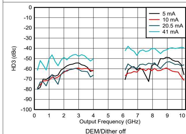
図 6-157. HD3 vs Frequency and Output Current in NRZ/RF Modes
