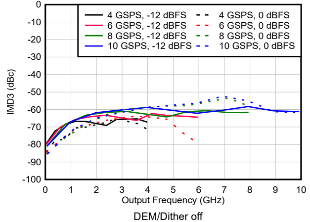
图 6-130. IMD3 vs Frequency and Sample Rate in NRZ/RF Modes
