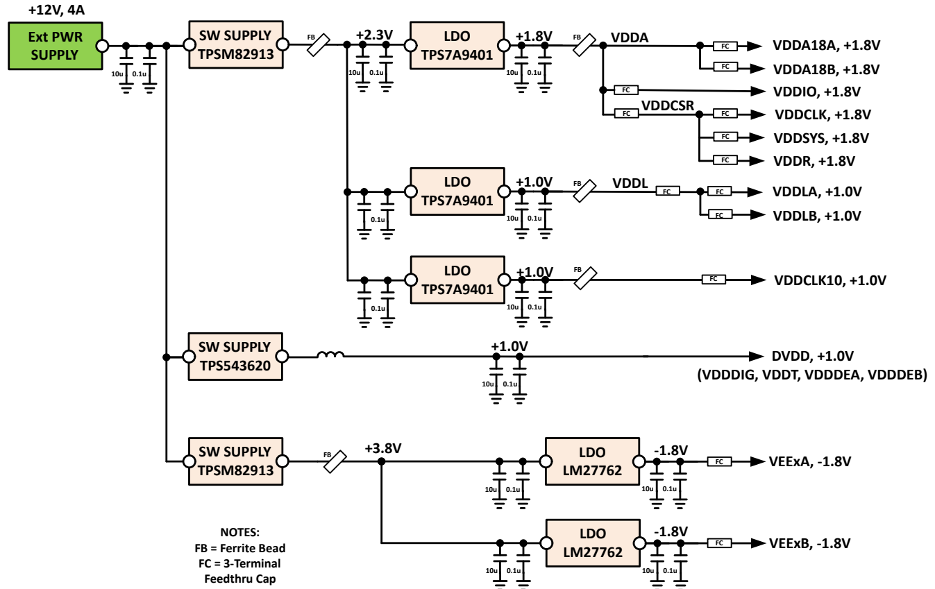
8-23. Recommended Power Supply Block Diagram
