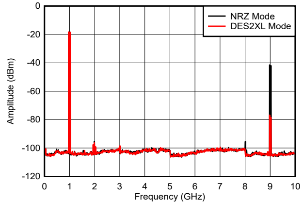
图 6-44. Dual Tone, f_{\text{OUT}} = 997\text{ MHz} , -6 dBFS
