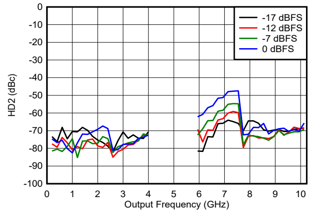
FIG 6-148. HD2 vs Frequency and Digital Amplitude in NRZ/RF Modes
