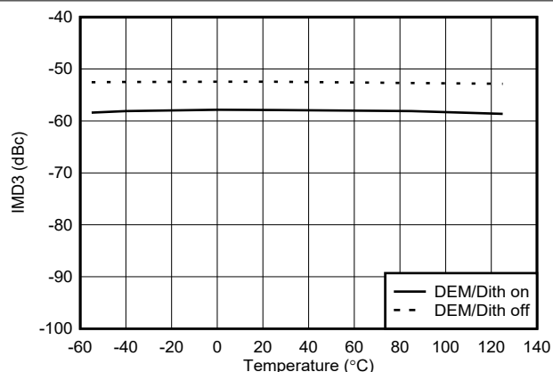
図 6-136. IMD3 vs Temperature in DES2XH Mode at 7247 MHz
