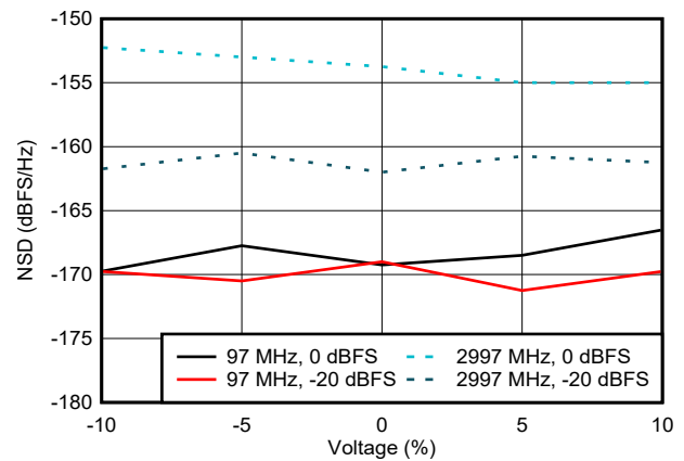
図 6-87. NSD vs Supply Voltage
