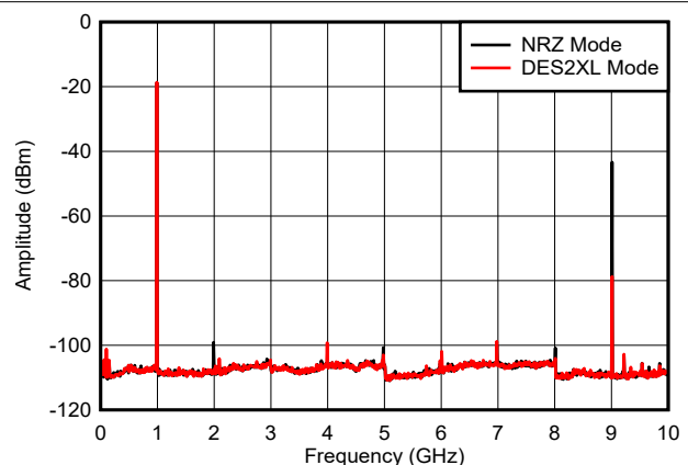
✎ 6-22. f_{\text{OUT}} = 997\text{ MHz} , 0 dBFS
