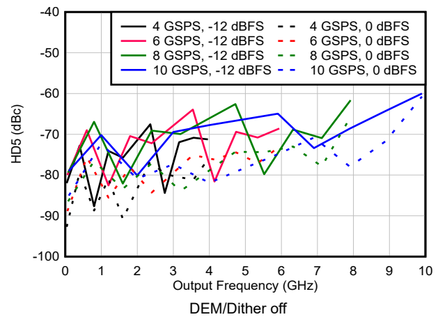
FIG 6-190. HD5 vs Frequency and Sample Rate in NRZ/RF Modes
