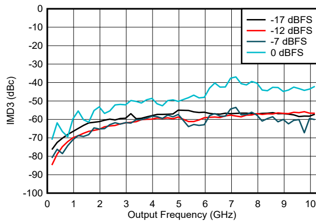
FIG 6-117. IMD3 vs Frequency and Digital Amplitude in NRZ/RF Modes
