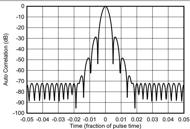
図 8-17. Auto-correlation of NLFM Chirp
