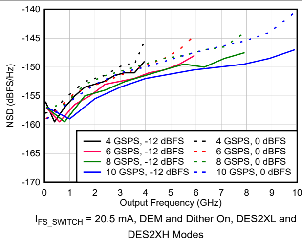
図 6-80. NSD vs Output Frequency and Sample Rate
