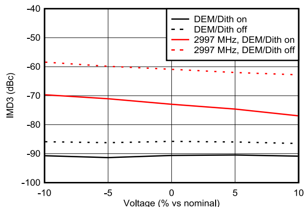
図 6-138. IMD3 vs Voltage in DES2XL Mode
