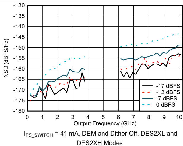
FIG 6-72. NSD vs Output Frequency and Digital Amplitude
