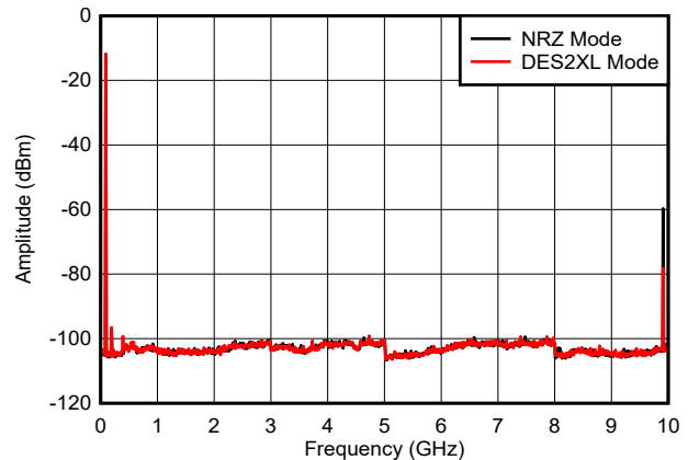
✎ 6-20. f_{\text{OUT}} = 97\text{ MHz} , -6 dBFS
