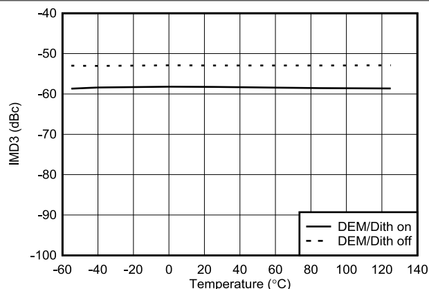
図 6-135. IMD3 vs Temperature in RF Mode at 7247 MHz
