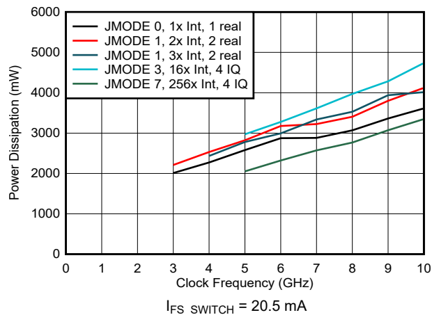
6-211. Power Dissipation vs Clock Frequency and Digital Mode
