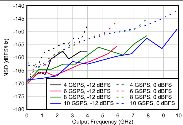
Figure 6-77. NSD vs Output Frequency and Sample Rate
