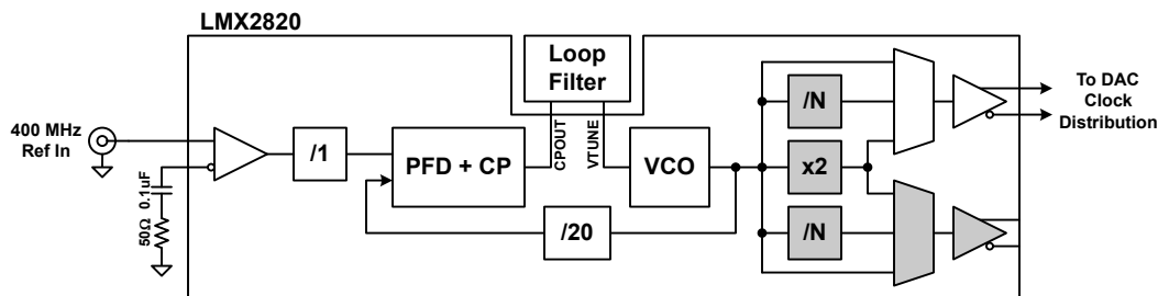
図 8-8. LMX2820 with Internal VCO
