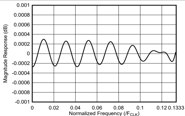
7-17. 3x Interpolation Filter Passband Response
