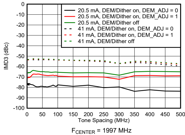
6-125. IMD3 vs Tone Spacing in NRZ Mode
