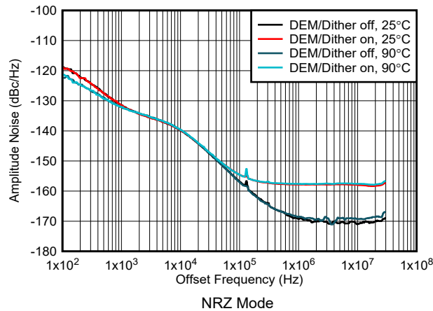
Figure 6-209. Amplitude Noise vs Offset Frequency and Temperature at 1 GHz
