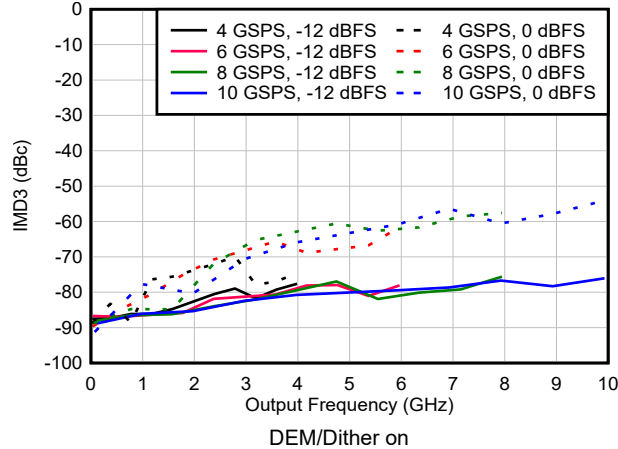
图 6-129. IMD3 vs Frequency and Sample Rate in NRZ/RF Modes
