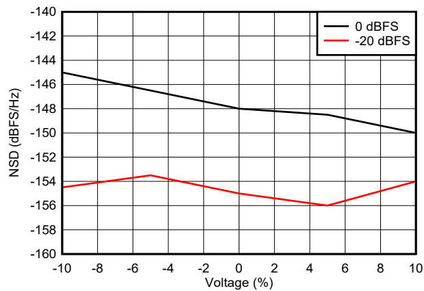
図 6-86. NSD vs Supply Voltage
