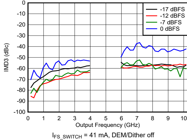
6-123. IMD3 vs Frequency and Digital Amplitude in DES2X Modes
