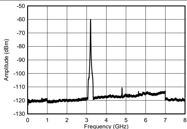
図 8-18. NLFM Chirp Output Spectra across 0 - 8 GHz
