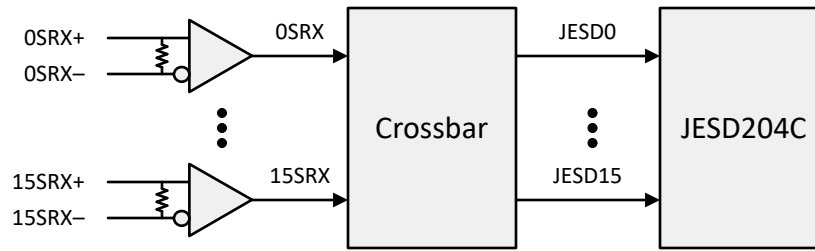
FIG 7-53. Crossbar Block Diagram
