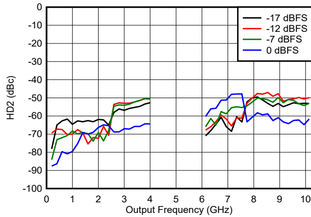
FIG 6-147. HD2 vs Frequency and Digital Amplitude in NRZ/RF Modes
