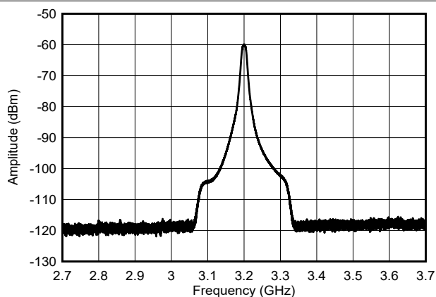
図 8-19. NLFM Chirp Output Spectra across 1 GHz
