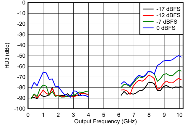
FIG 6-166. HD3 vs Frequency and Digital Amplitude in DES2X Modes
