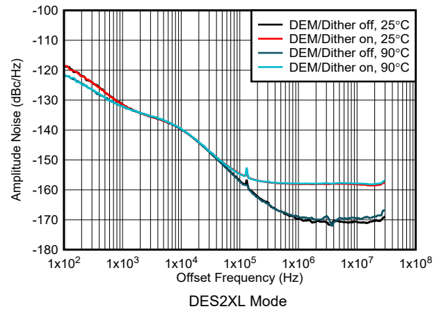
Figure 6-210. Amplitude Noise vs Offset Frequency and Temperature at 1 GHz
