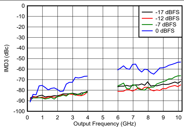
FIG 6-120. IMD3 vs Frequency and Digital Amplitude in NRZ/RF Modes
