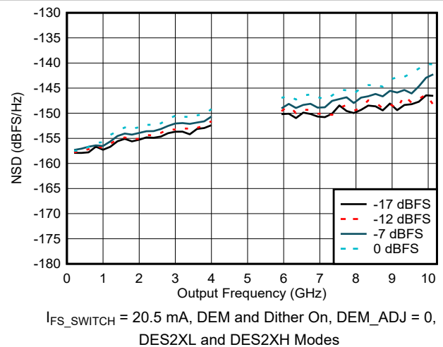
FIG 6-73. NSD vs Output Frequency and Digital Amplitude
