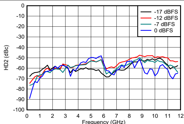
FIG 6-140. HD2 vs Frequency and Digital Amplitude in NRZ/RF Modes
