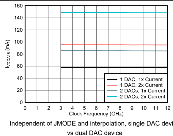
FIG 6-208. VDDA18 Current vs Clock Frequency and DAC Mode
