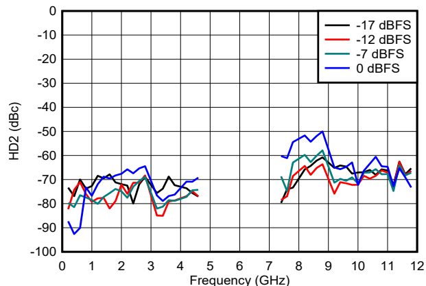
FIG 6-141. HD2 vs Frequency and Digital Amplitude in NRZ/RF Modes
