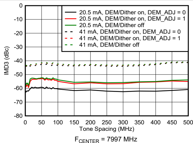
図 6-120. IMD3 vs Tone Spacing in RF Mode
