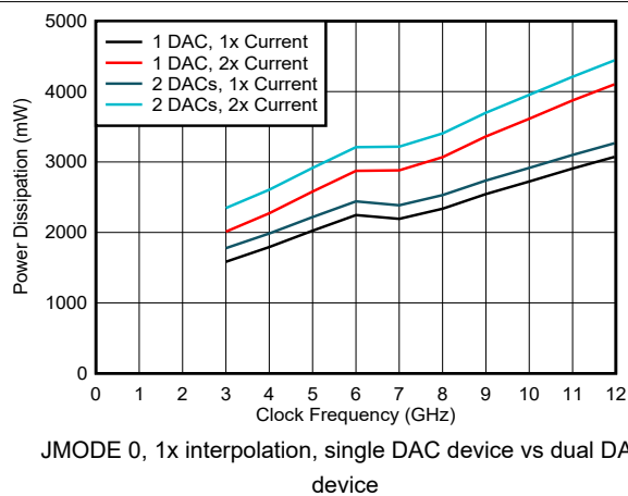
FIG 6-207. Power Dissipation vs Clock Frequency and DAC Mode
