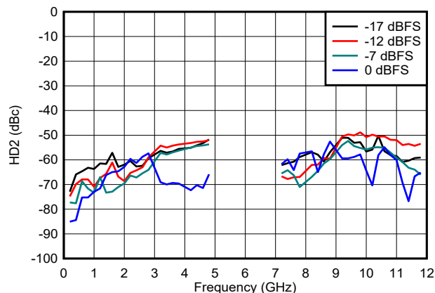
FIG 6-142. HD2 vs Frequency and Digital Amplitude in DES2X Modes
