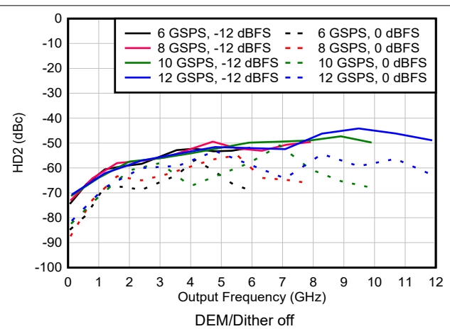
図 6-147. HD2 vs Frequency and Sample Rate in NRZ/RF Modes
