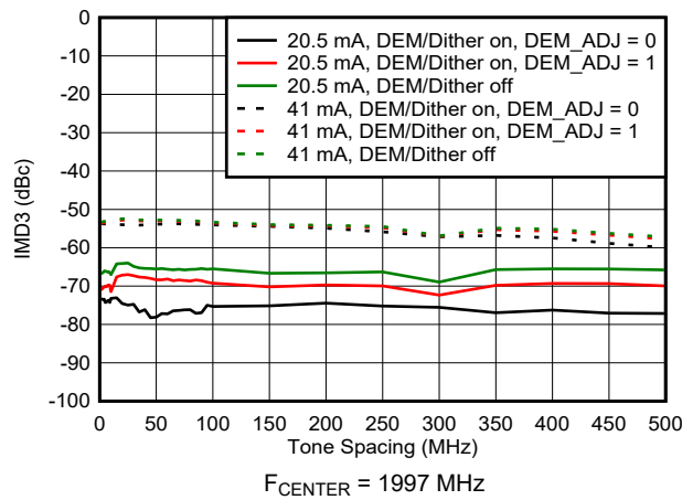
図 6-118. IMD3 vs Tone Spacing in NRZ Mode
