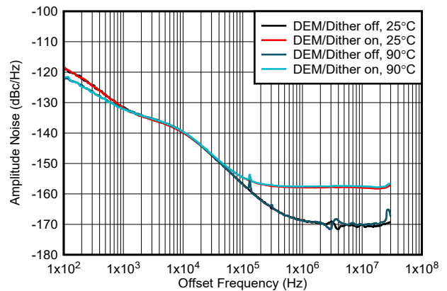
Figure 6-202. Amplitude Noise vs Offset Frequency and Temperature at 1 GHz
