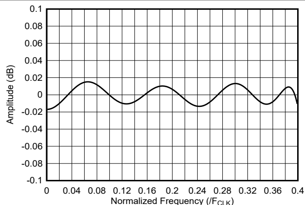
7-49. DES Interpolator Frequency Response (Passband)
