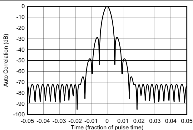
図 8-16. Auto-correlation of NLFM Chirp
