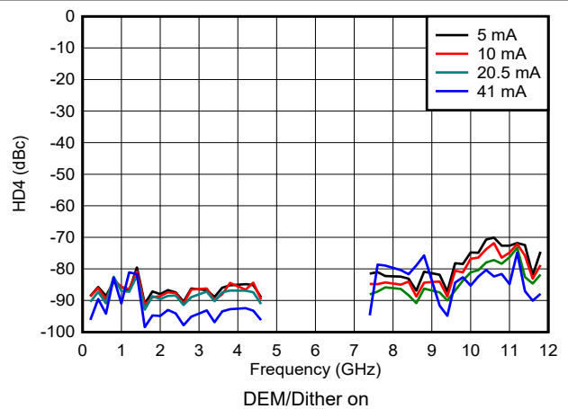
図 6-169. HD4 vs Frequency and Output Current in DES2X Modes
