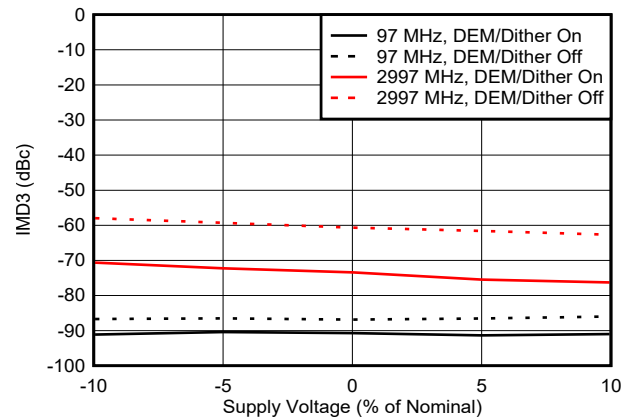
Figure 6-131. IMD3 vs Voltage in DES2XL Mode
