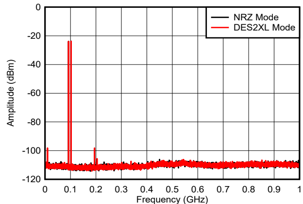
6-40. Dual Tone, f_{\text{OUT}} = 97\text{ MHz} , -6 dBFS (0 - 1 GHz)
