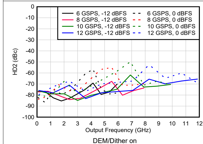
図 6-148. HD2 vs Frequency and Sample Rate in DES2X Modes
