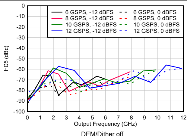
図 6-185. HD5 vs Frequency and Sample Rate in DES2X Modes
