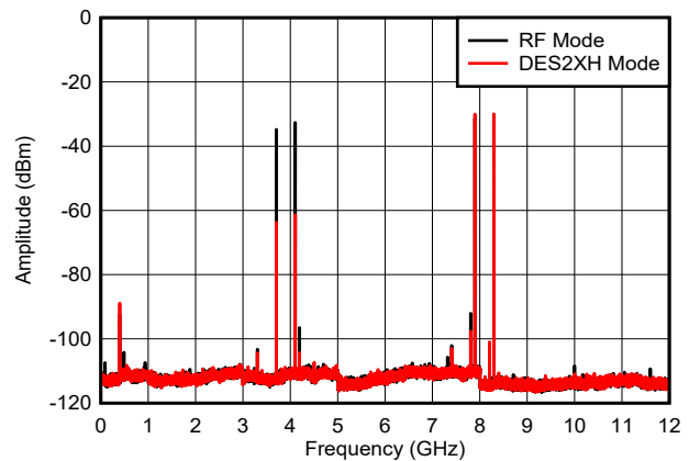
Figure 6-52. Dual Tone, f_{\text{OUT}} = 8097\text{ MHz} , 0 dBFS
