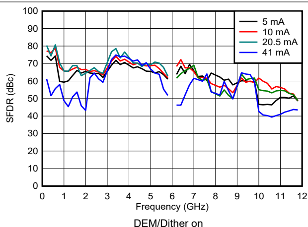
Figure 6-93. SFDR vs Frequency and Output Current in DES2X Modes
