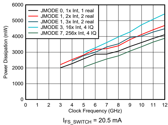
FIG 6-203. Power Dissipation vs Clock Frequency and Digital Mode
