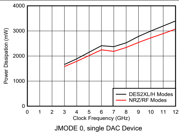
FIG 6-205. Power Dissipation vs Clock Frequency and DAC Mode
