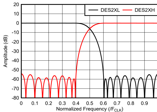
Figure 8-1. DES Interpolator Frequency Response
