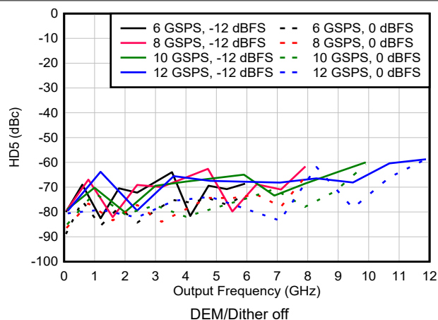
図 6-183. HD5 vs Frequency and Sample Rate in NRZ/RF Modes
