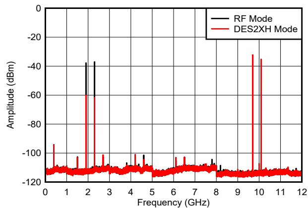
✎ 6-55. Dual Tone, f_{\text{OUT}} = 9897\text{ MHz} , 0 dBFS
