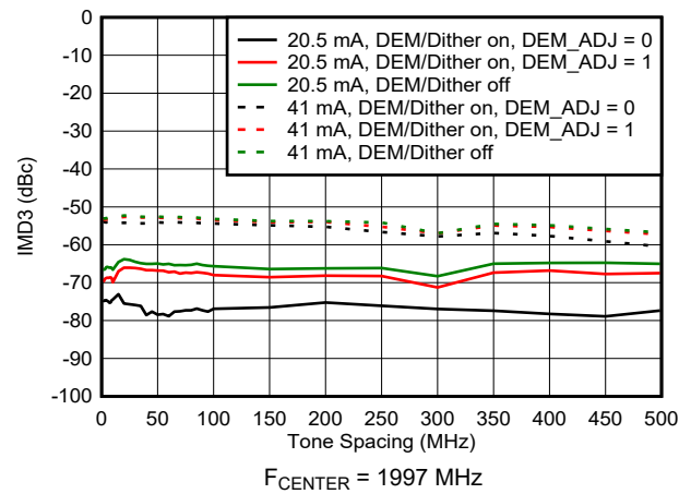
図 6-119. IMD3 vs Tone Spacing in DES2XL Mode
