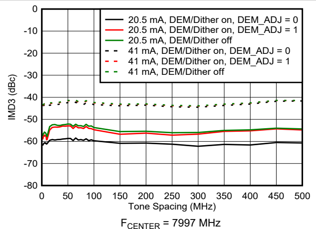
図 6-121. IMD3 vs Tone Spacing in DES2XH Mode
