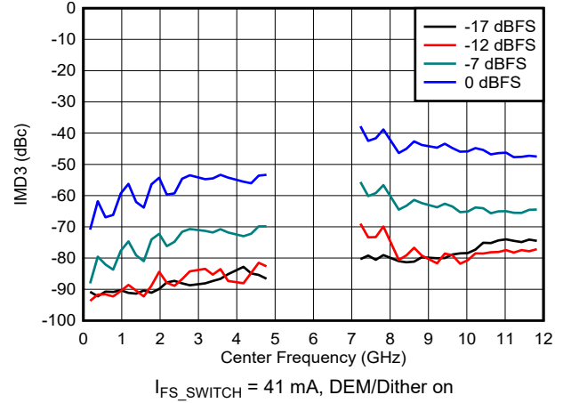
図 6-117. IMD3 vs Frequency and Digital Amplitude in DES2X Modes
