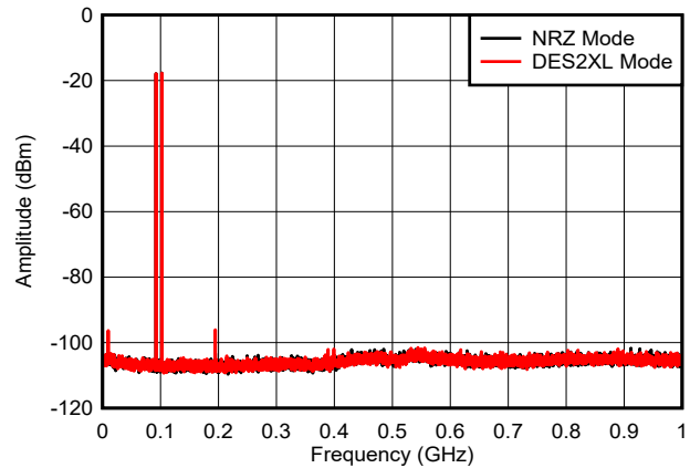
6-38. Dual Tone, f_{\text{OUT}} = 97\text{ MHz} , 0 dBFS (0 - 1 GHz)
