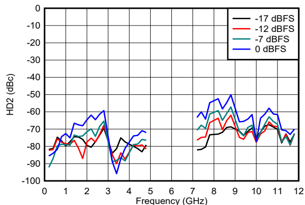
FIG 6-143. HD2 vs Frequency and Digital Amplitude in DES2X Modes
