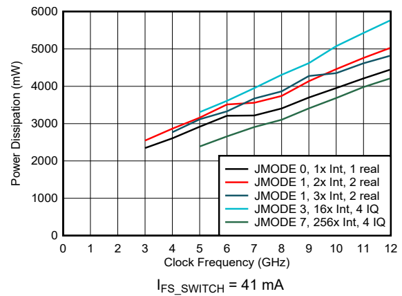
FIG 6-204. Power Dissipation vs Clock Frequency and Digital Mode
