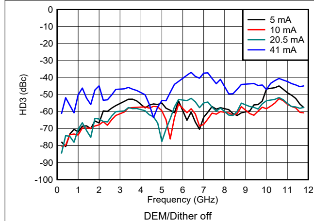
図 6-150. HD3 vs Frequency and Output Current in NRZ/RF Modes
