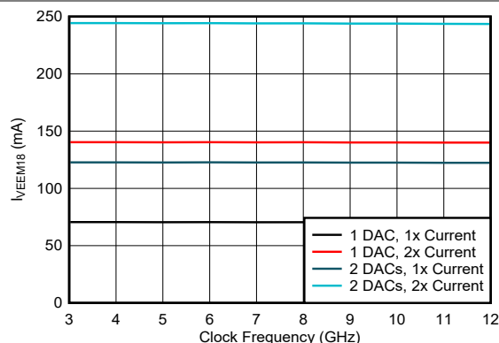
FIG 6-210. VEEM18 Current vs Clock Frequency and DAC Mode
