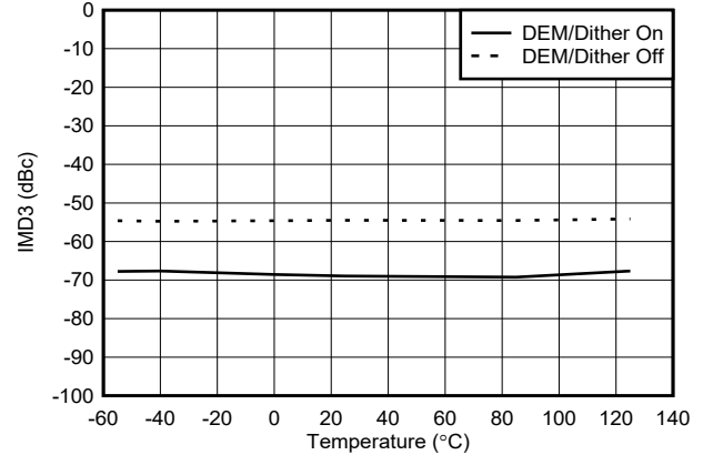
Figure 6-129. IMD3 vs Temperature in DES2XH Mode at 9002 MHz
