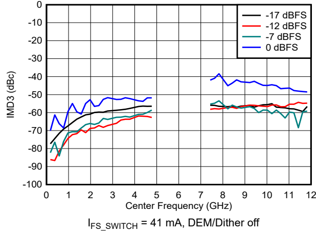
図 6-116. IMD3 vs Frequency and Digital Amplitude in DES2X Modes
