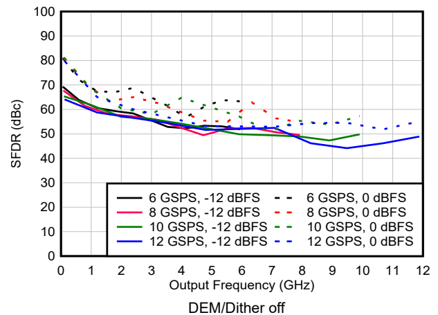
Figure 6-103. SFDR vs Frequency and Sample Rate in NRZ/RF Modes
