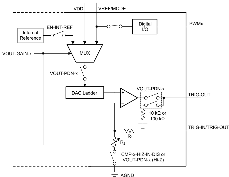
7-2. Voltage Reference Selection and Power-Down Logic
