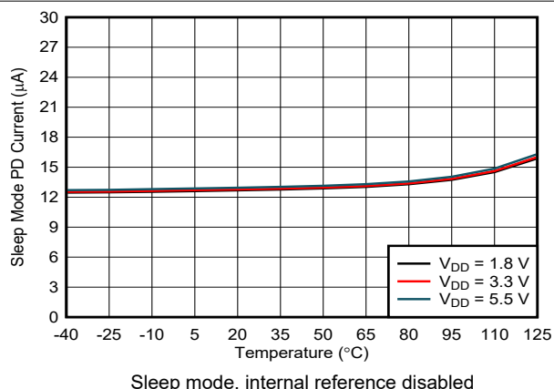
図 6-13. Power-Down Current vs Temperature
