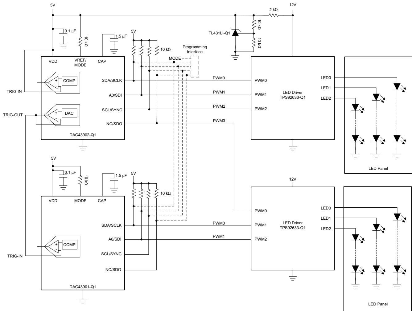
☒ 8-1. Sequential Turn Indicator
