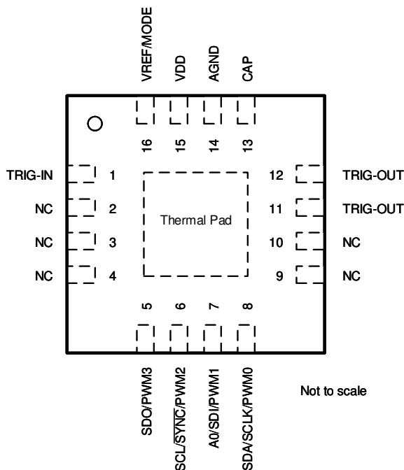
図 5-2. DAC43902-Q1: RTE Package, 16-pin WQFN (Top View)
