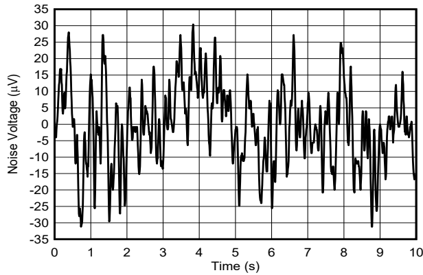
Internal reference, gain = 4x, f = 0.1 Hz to 10 Hz
