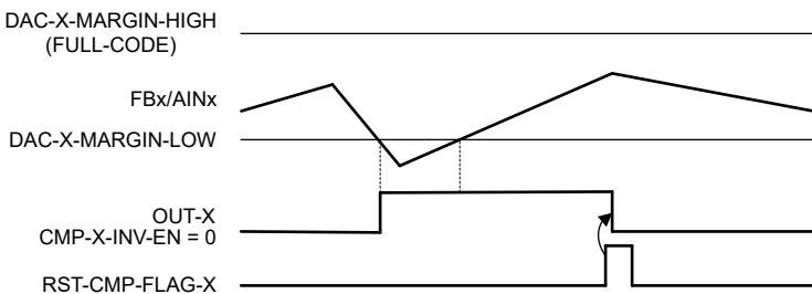
图 7-7. Latching Comparator With Active High Output
