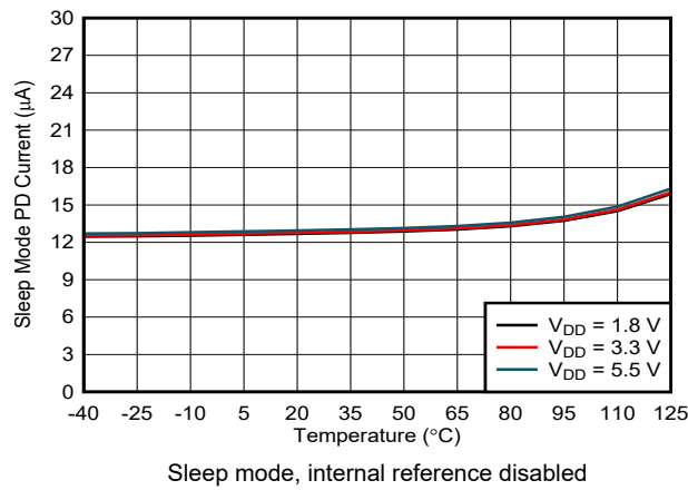
6-56. Power-Down Current vs Temperature
