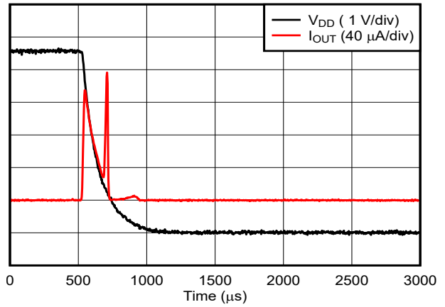
6-44. Current Output Setting Time, Falling Edge
