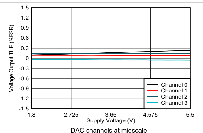
Figure 6-15. Voltage Output TUE vs Supply Voltage
