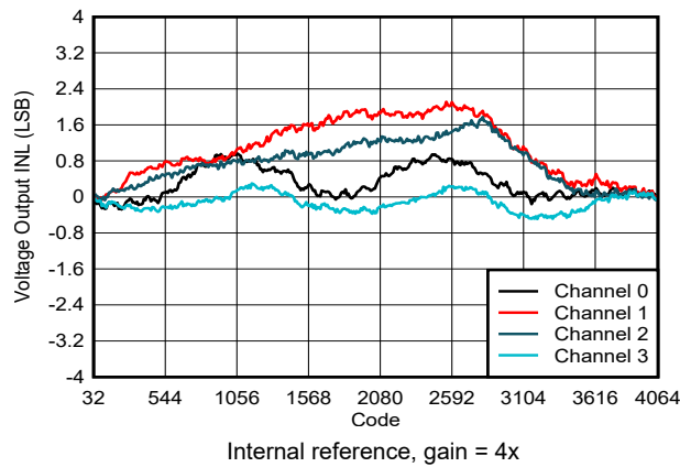
6-4. Voltage Output INL vs Digital Input Code
