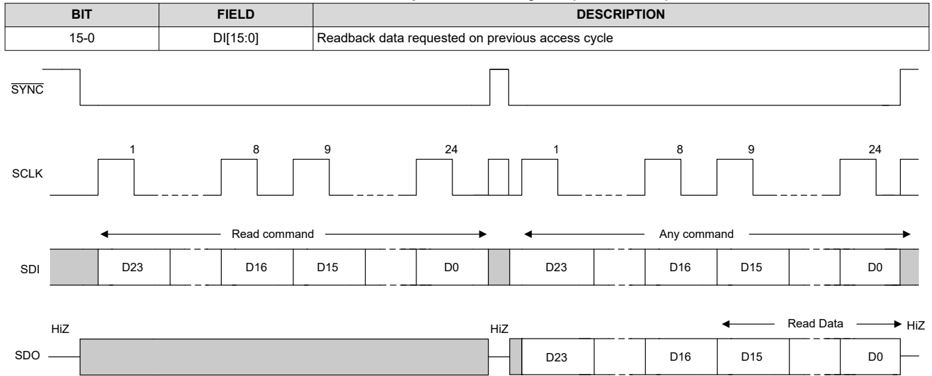
図 7-15. SPI Read Cycle
