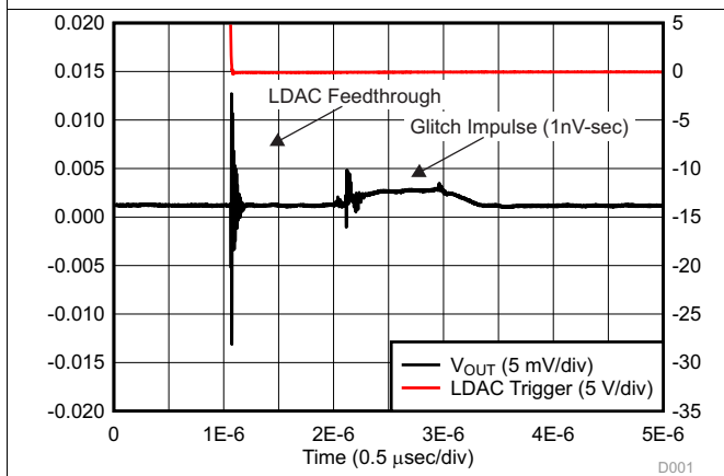
DAC code transition from 8000h to 7FFFh
