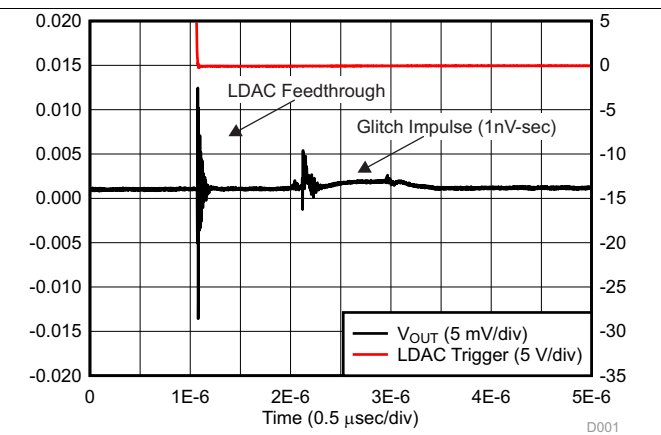
DAC code transition from 7FFFh to 8000h
