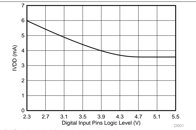
DAC unloaded, All channels to mid-scale
