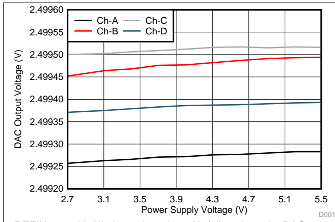
REFIN = 2.5 V, All channels active with full-scale code, DAC unloaded
