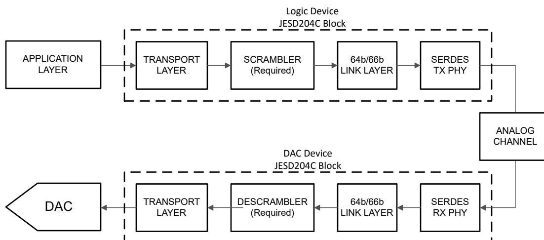
図 7-51. Simplified JESD204C Interface Diagram with 64b/66b Encoding
