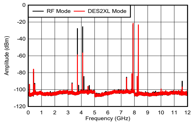
図 6-39. Dual Tone, f_{\text{OUT}} = 8097\text{MHz} , -6dBFS
