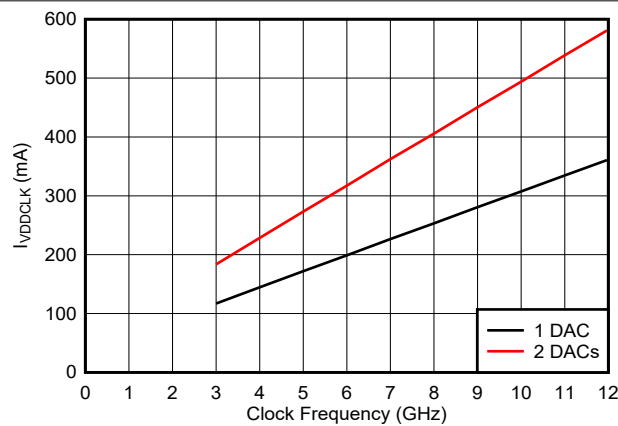
Independent of JMODE and Interpolation Figure 6-52. VDDCLK Current vs Clock Frequency
