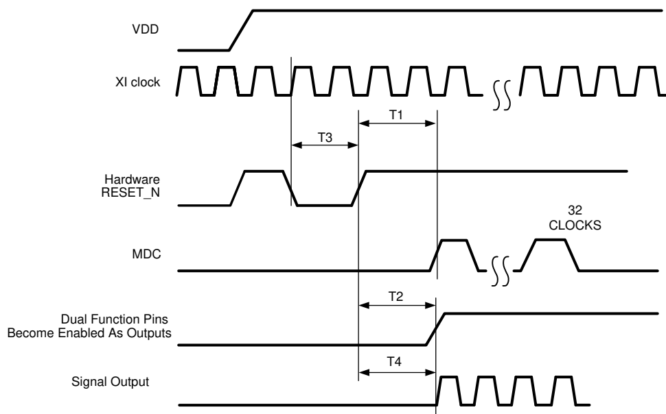
FIG 6-2. Reset Timing
