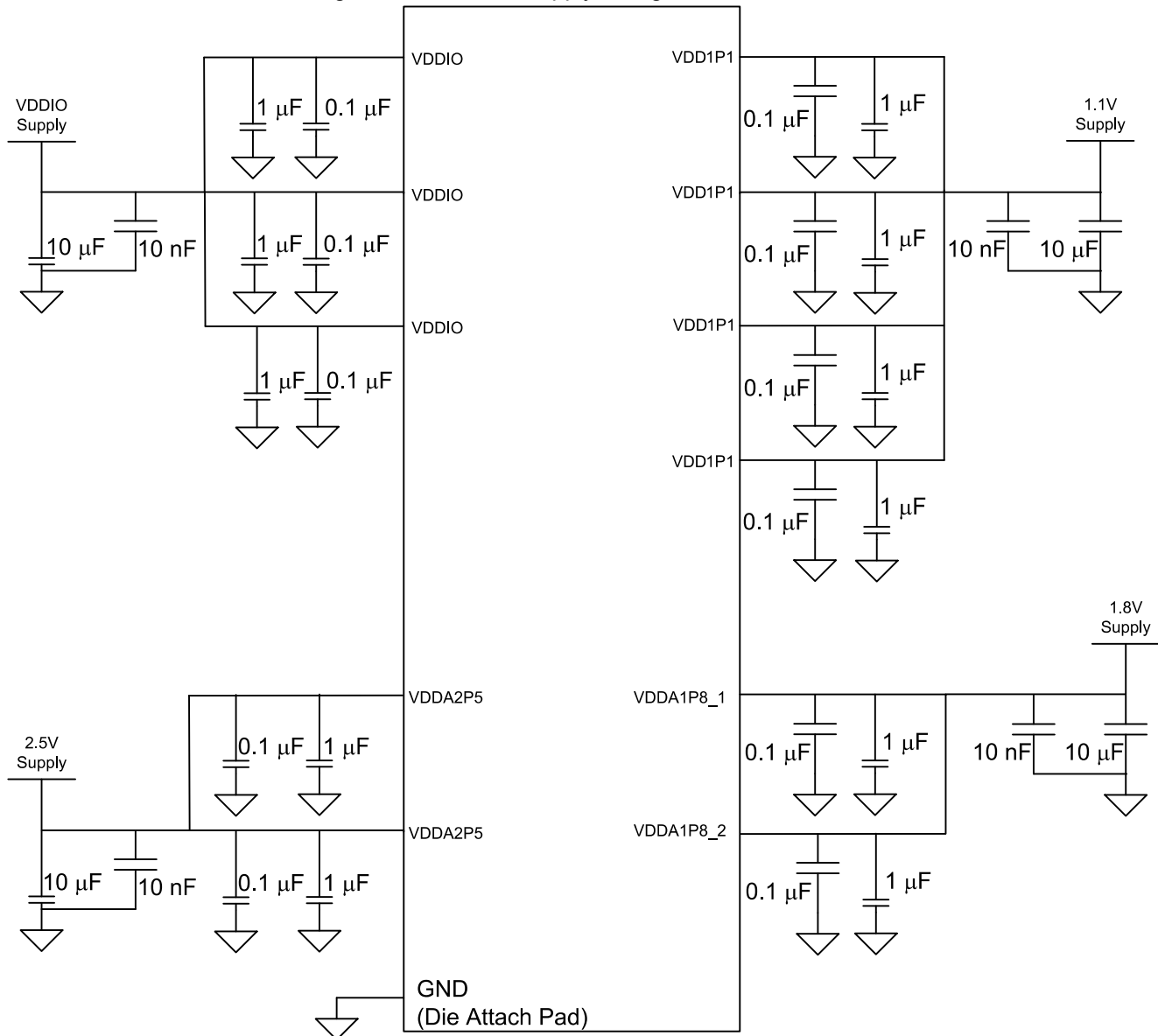
Figure 9-3. Three-Supply Configuration
