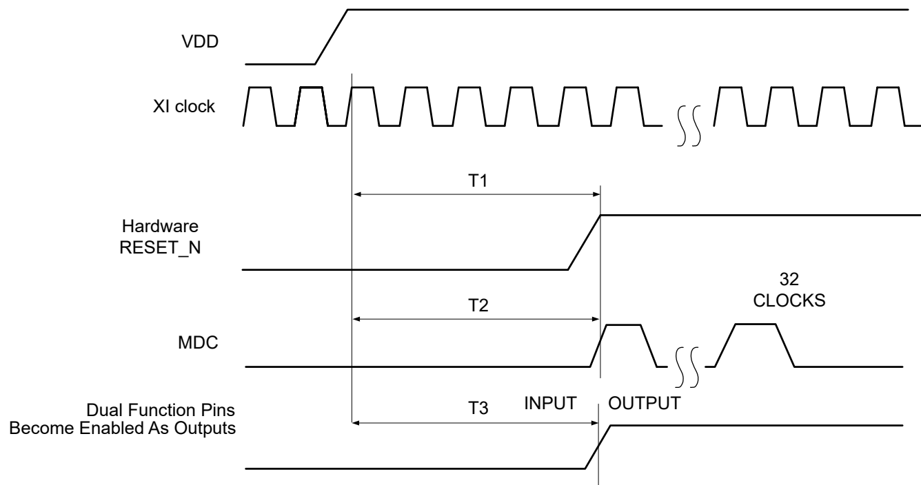
FIG 6-1. Power-Up Timing
