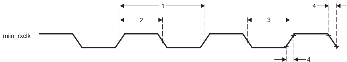
図 7-52. Clock Timing (GMAC Receive) - MII operation
