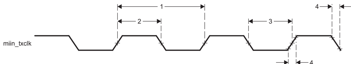
図 7-53. Clock Timing (GMAC Transmit) - MII operation
