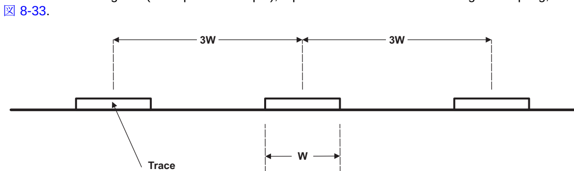
8-33. 3W Spacing Rule
