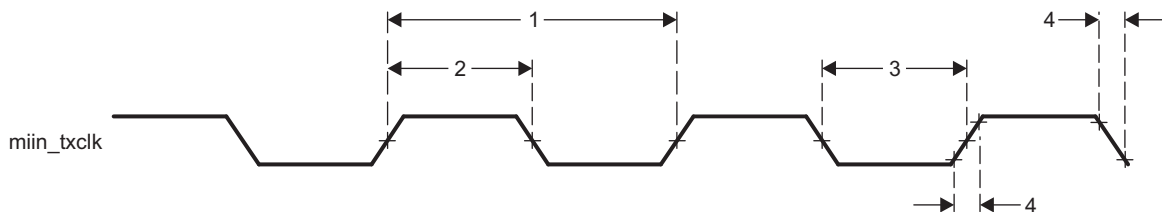
图 7-53. Clock Timing (GMAC Transmit) - MIIn operation
