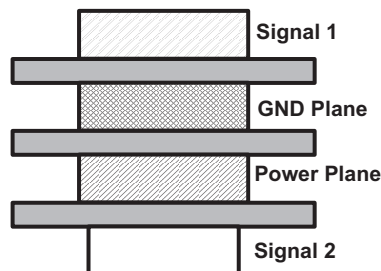
Figure 8-31. Four-Layer Board Stack-Up
