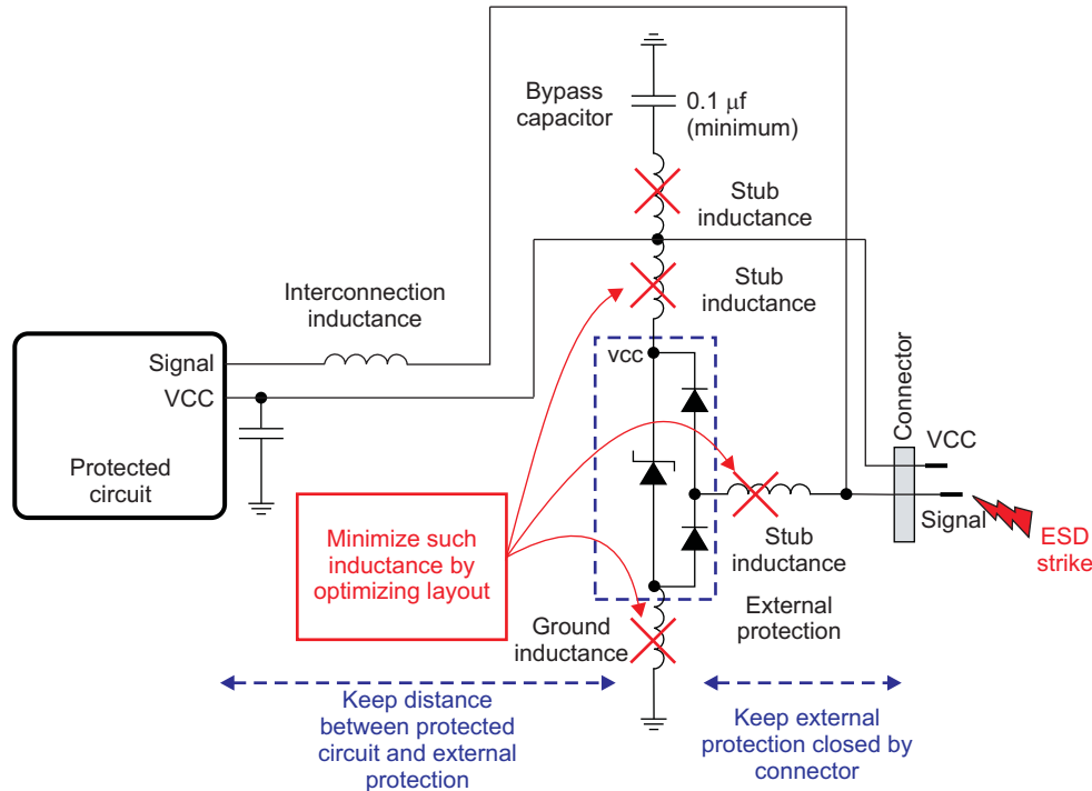
☒ 8-16. Placement Recommendation for an ESD External Protection
