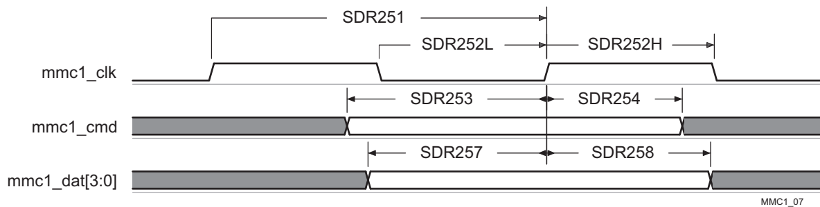
图 7-68. MMC/SD/SDIO in - High Speed SDR25 - Receiver Mode
