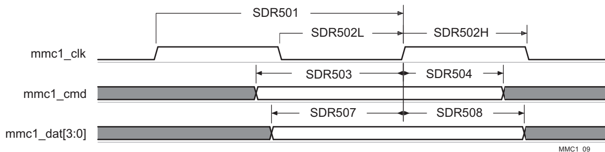
图 7-70. MMC/SD/SDIO in - High Speed SDR50 - Receiver Mode
