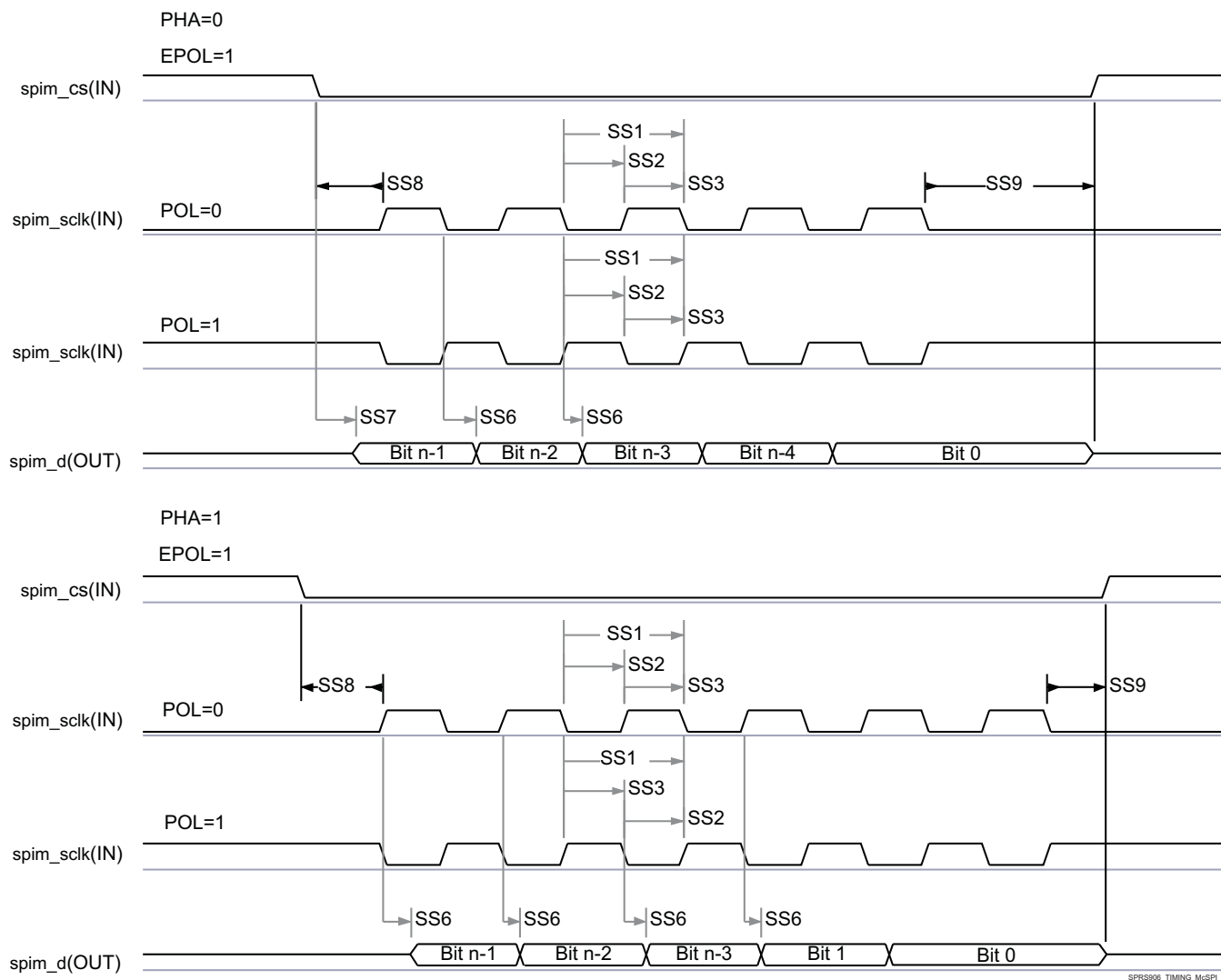
7-35. McSPI - Slave Mode Transmit
