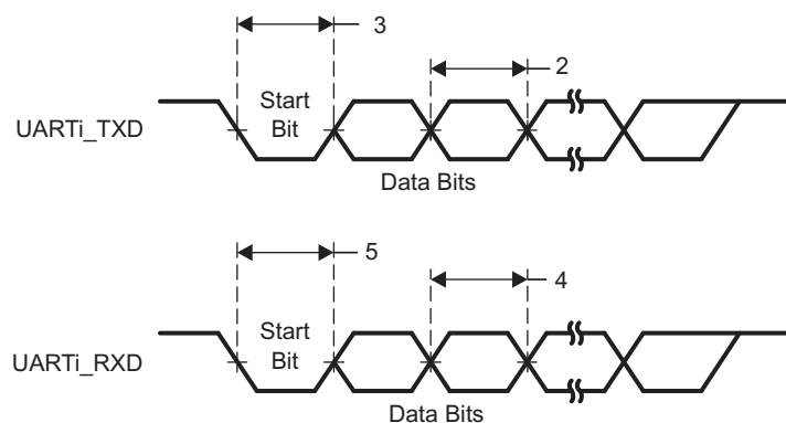
Figure 5-48. UART Timing
