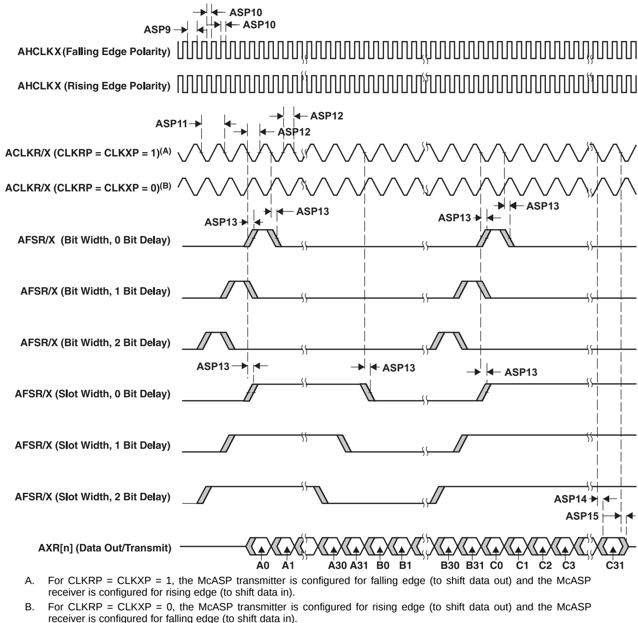
Figure 5-58. McASP Output Timing
