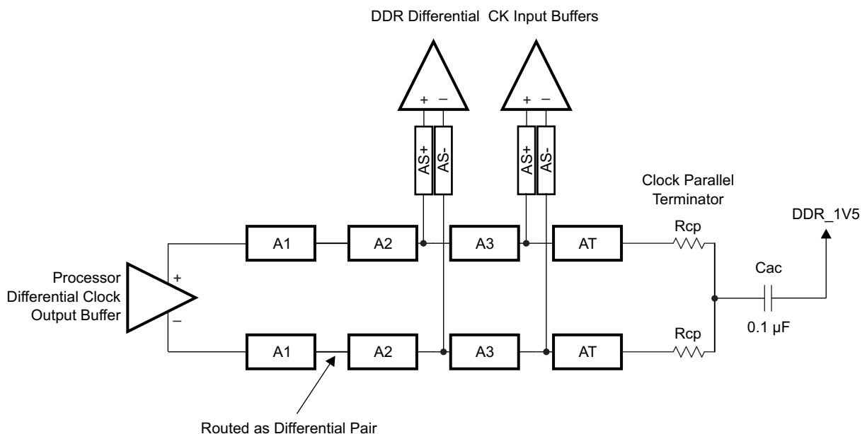
FIG 7-48. CK Topology for Two DDR3 Devices
