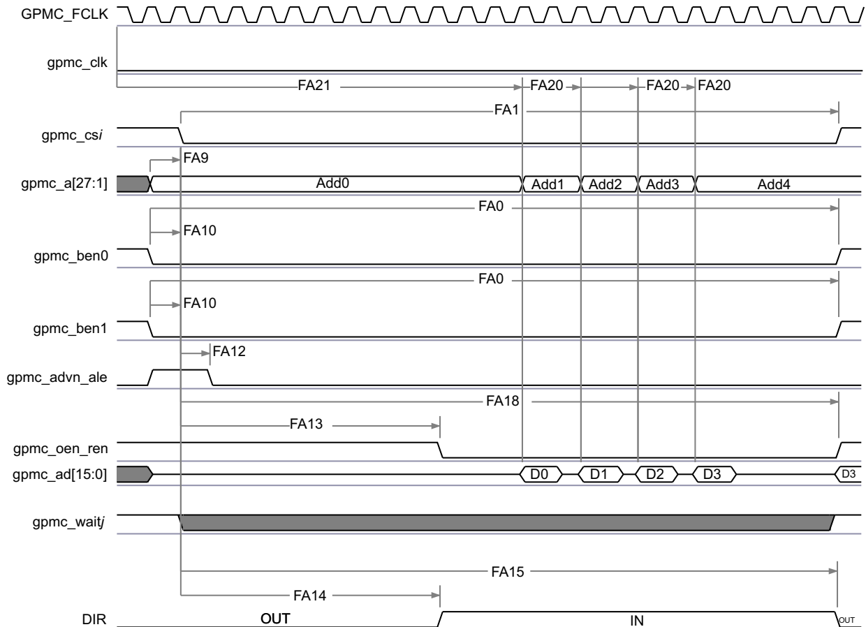
FIG 5-31. GPMC / NOR Flash - Asynchronous Read - Page Mode 4x16-bit Timing (1)(2)(3)(4)
