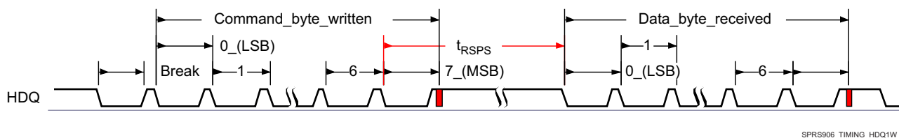
图 5-44. HDQ Communication Timing
