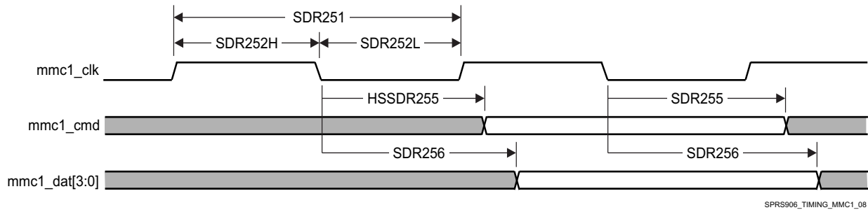
図 5-85. MMC/SD/SDIO in - High Speed SDR25 - Transmitter Mode
