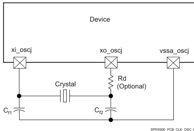
✎ 7-36. Grounding Scheme for High-Frequency Clock
