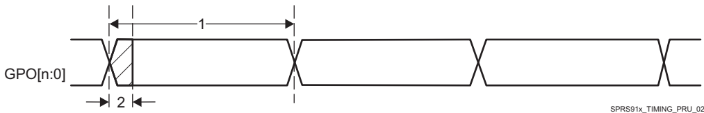
图 5-110. PRU-ICSS PRU Direct Output Timing
