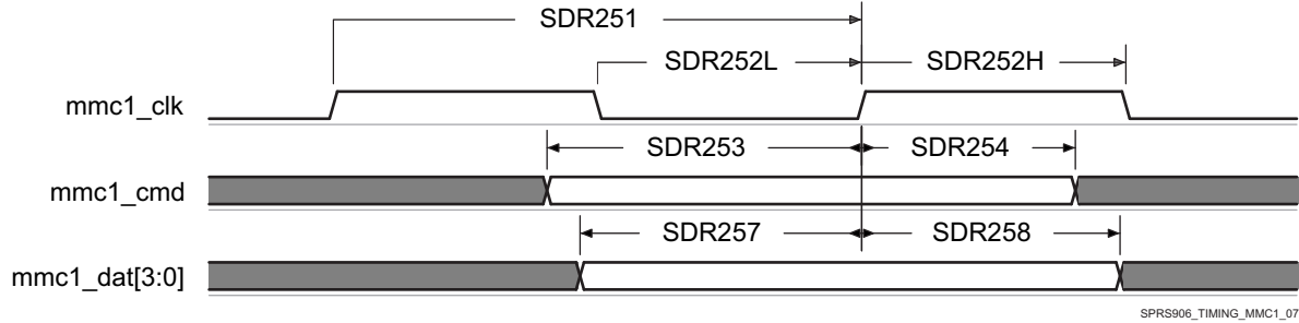
図 5-84. MMC/SD/SDIO in - High Speed SDR25 - Receiver Mode
