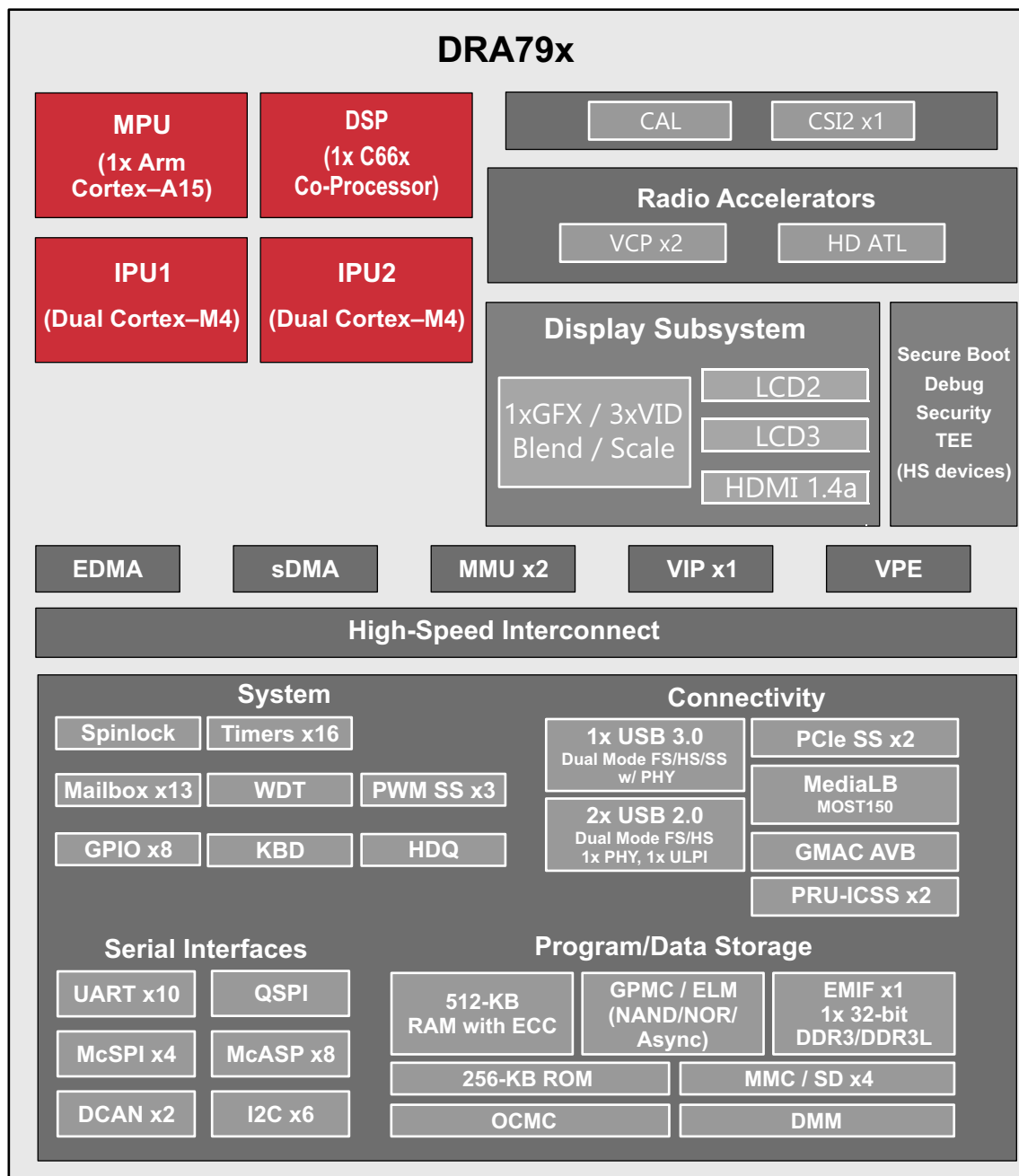
6-1. DRA79x Block Diagram
