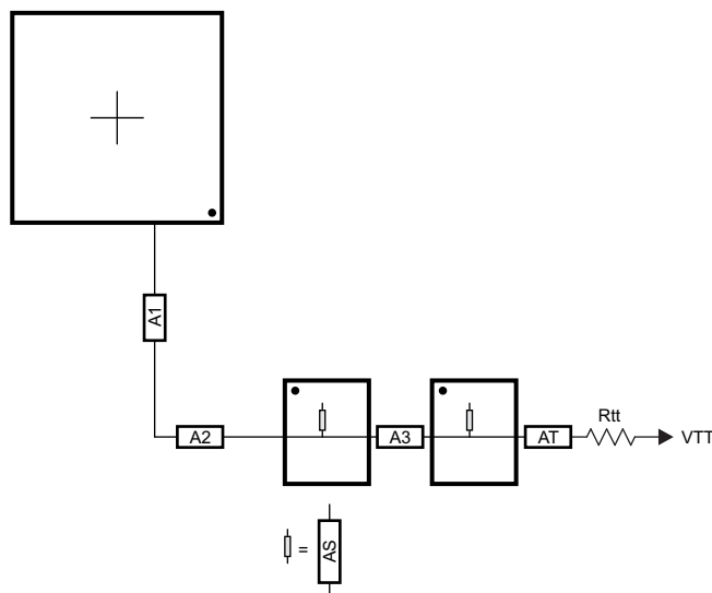
7-51. ADDR_CTRL Routing for Two Single-Side DDR3 Devices
