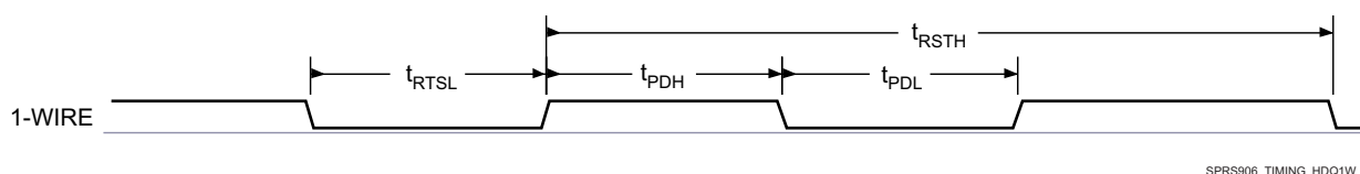
图 5-45. 1-Wire—Break (Reset)
