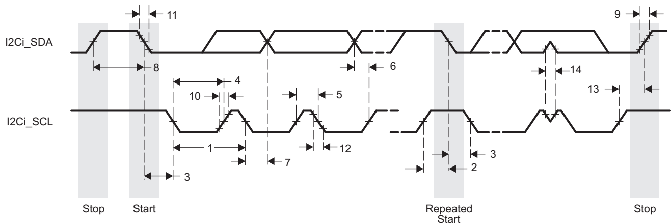
图 5-39. I2C Receive Timing
