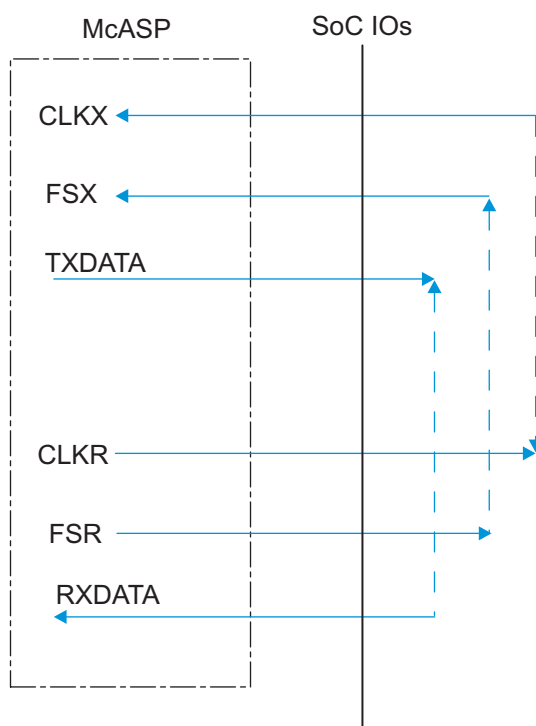
FIG 5-61. McASP1-8 CIOFIO – ASYNC Mode
