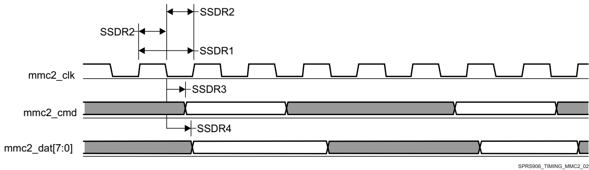
图 5-93. MMC/SD/SDIO in - Standard JC64 - Transmitter Mode
