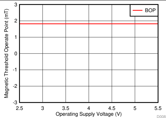
图 8. B_{OP} Threshold vs Supply Voltage (DRV5015A2, DRV5015A3)
