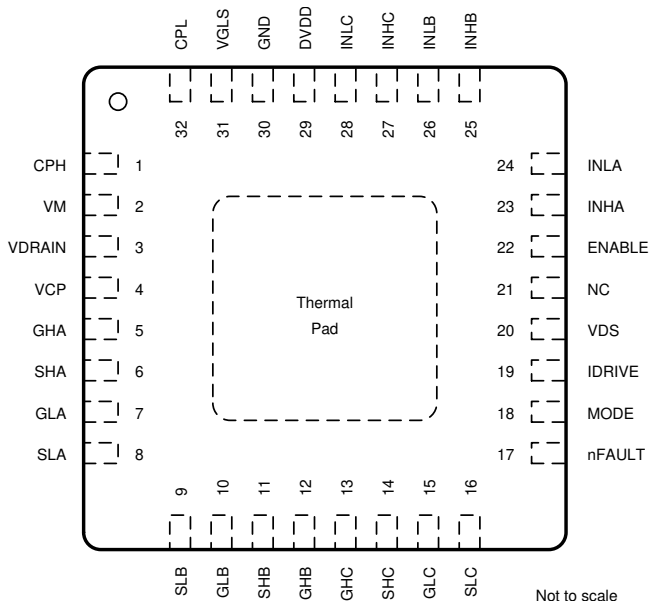
Pin Functions—32-Pin DRV8350 Devices
