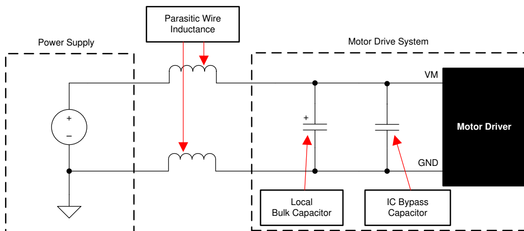
图 74. Motor Drive Supply Parasitics Example
