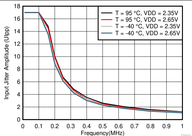
7-5. Typical Sinusoidal Input Jitter Tolerance for 30-dB Channel at 25.78125 Gbps
