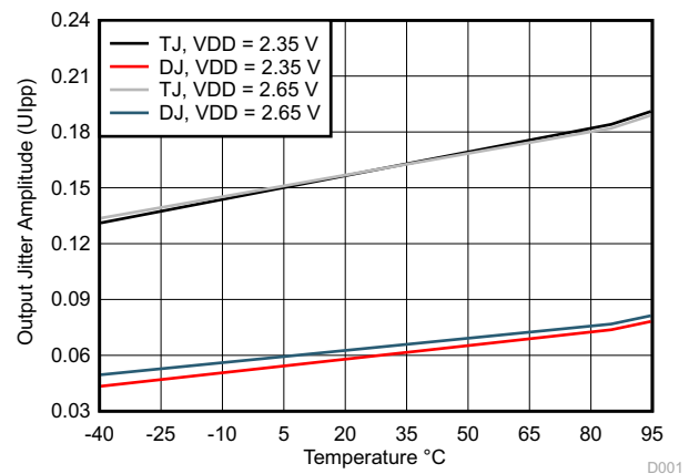
7-4. Typical Output Jitter vs Ambient Temperature at 25.78125 Gbps
