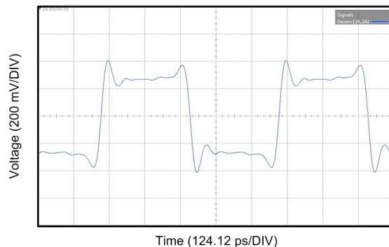
✕ 19. DS250DF810 FIR Transmit Equalization while Operating at 25.78125 Gbps
