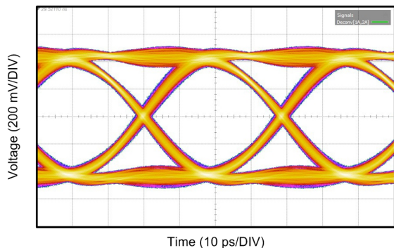
✕ 18. DS250DF810 Operating at 25.78125 Gbps
