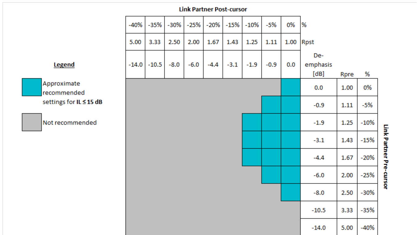
图 11. Guideline for link partner FIR settings when IL \leq 15 dB
