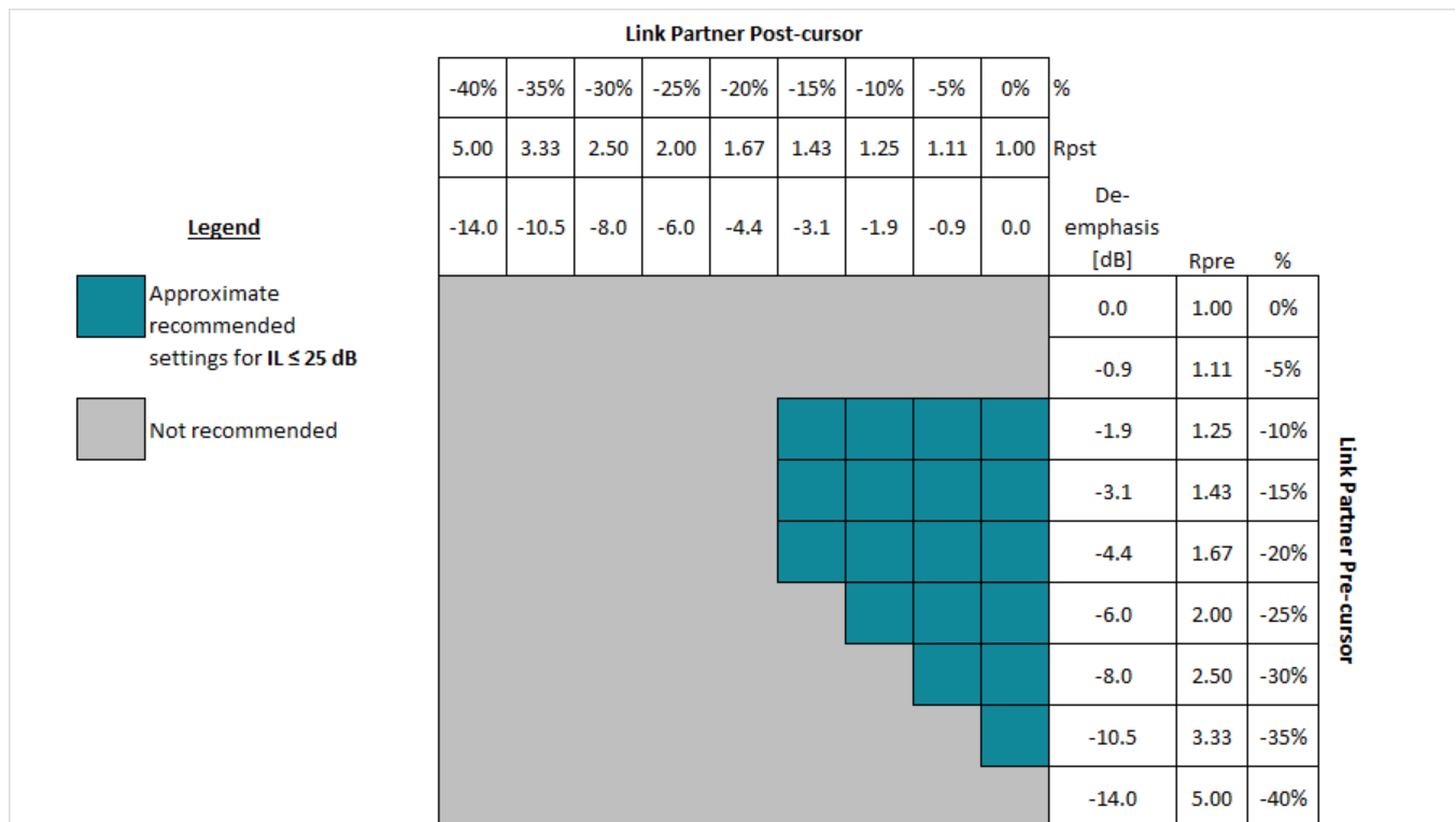
图 12. Guideline for link partner FIR settings when IL \leq 25 dB
