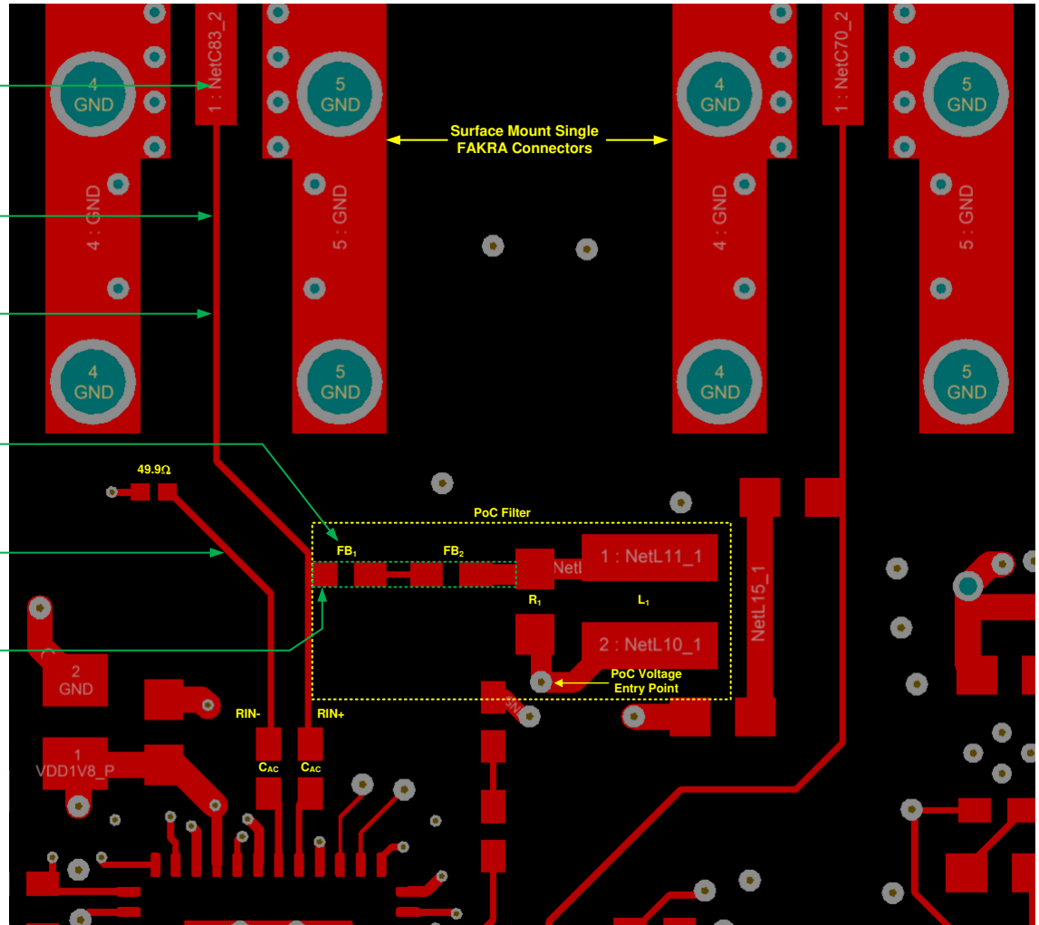
Figure 10-2. Example Routing of FPD-Link III Traces to a Single Mini-Fakra Connector and PoC Components
