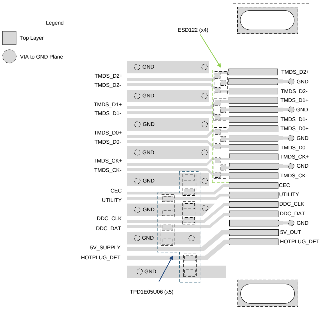
Figure 20. HDMI2_Layout
