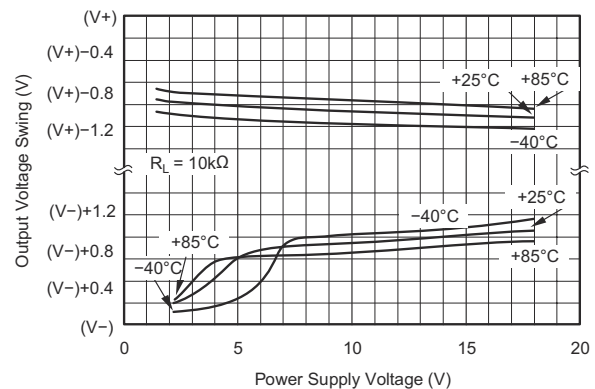
7-14. Output Voltage Swing vs Power Supply Voltage
