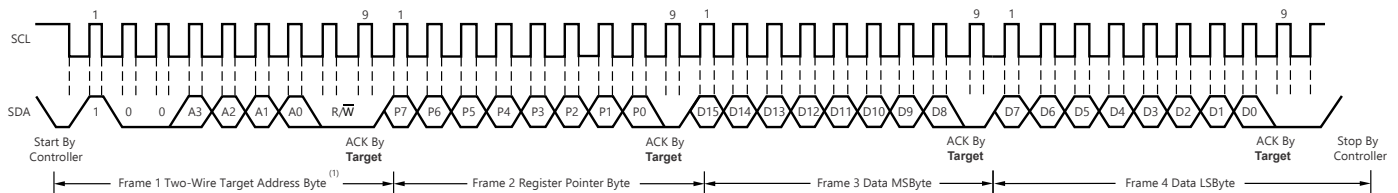
☒ 6-4. Timing Diagram for Write Word Format
