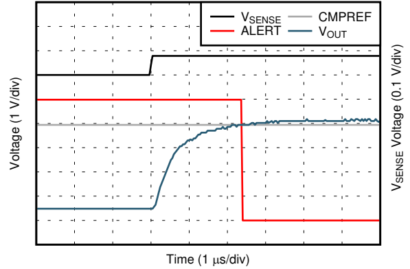
32. Brownout Recovery
