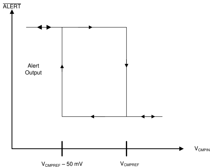
44. Typical Comparator Hysteresis
