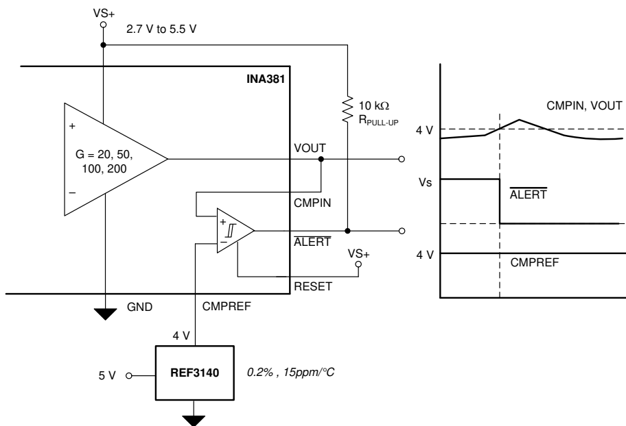
43. External Reference Voltage
