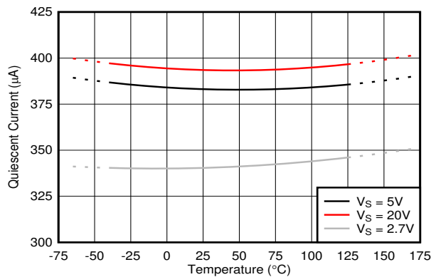
FIG 6-31. Quiescent Current vs. Temperature, INA290
