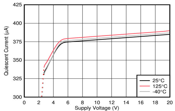
FIG 6-34. Quiescent Current vs. Supply Voltage, INA290
