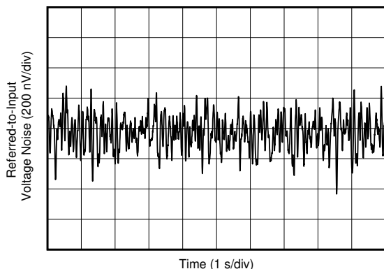
FIGURE 6-27. Input-Referred Noise
