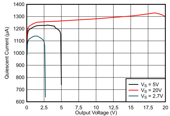
FIG 6-30. Quiescent Current vs. Output Voltage, INA4290
