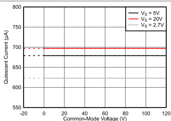
FIG 6-38. Quiescent Current vs. Common-Mode Voltage, INA2290
