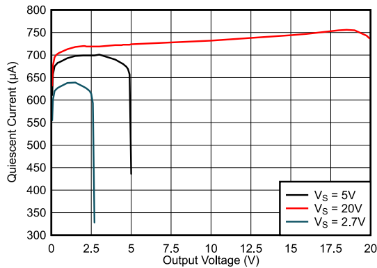
FIG 6-29. Quiescent Current vs. Output Voltage, INA290
