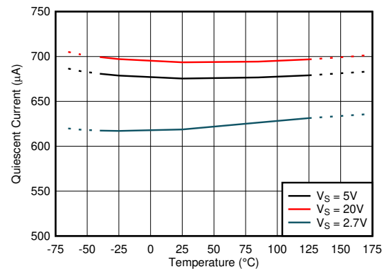
FIG 6-32. Quiescent Current vs. Temperature, INA4290
