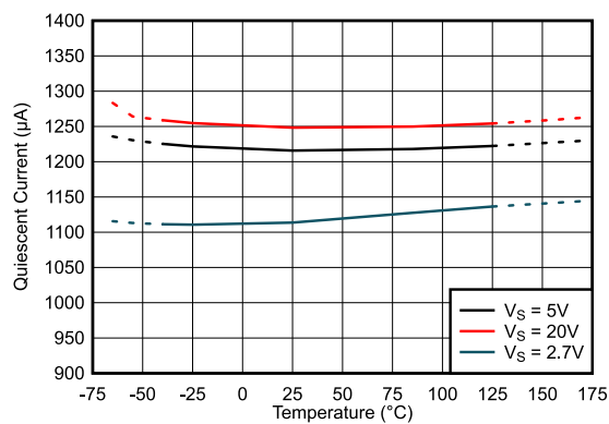
FIG 6-33. Quiescent Current vs. Temperature, INA290
