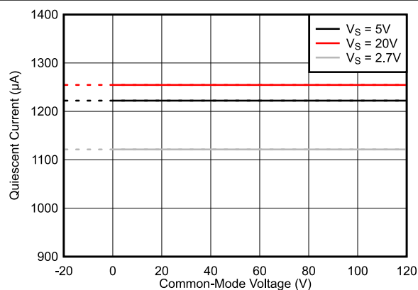
FIG 6-39. Quiescent Current vs. Common-Mode Voltage, INA2290
