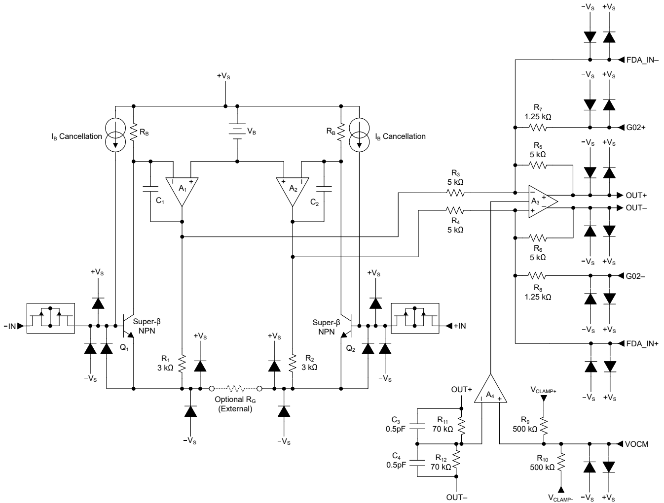
Figure 8-1. Detailed Schematic
