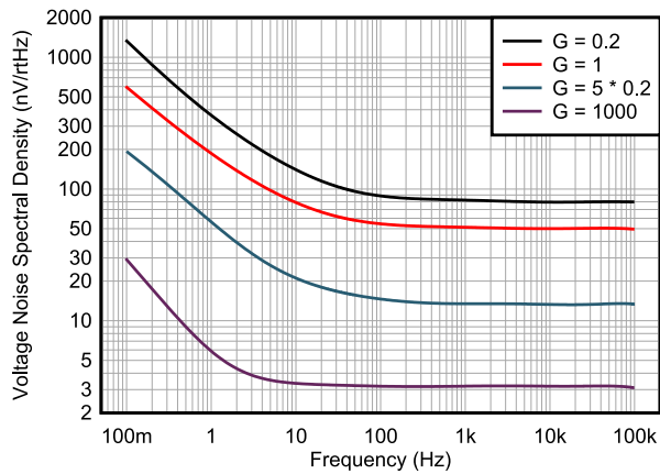
7-25. Voltage Noise Spectral Density vs Frequency (RTI)
