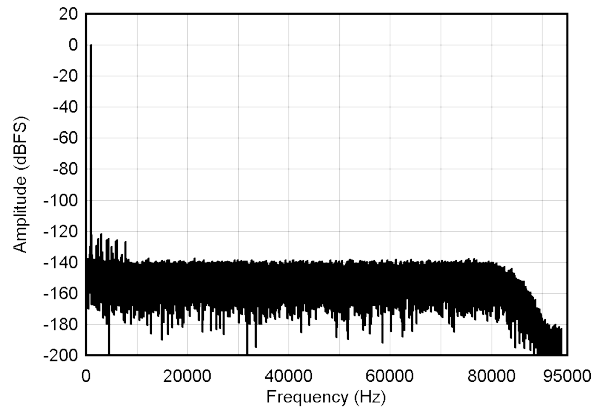
9-13. Noise Performance FFT Plots with Wideband Filter for G = 1 V/V
