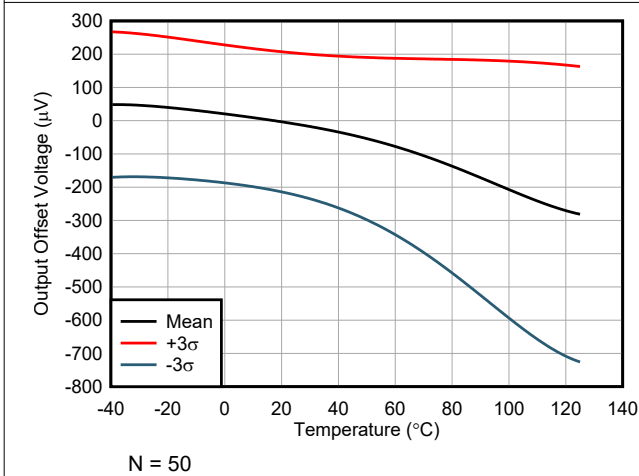
7-17. Input-Referred Output Offset Voltage vs Temperature
