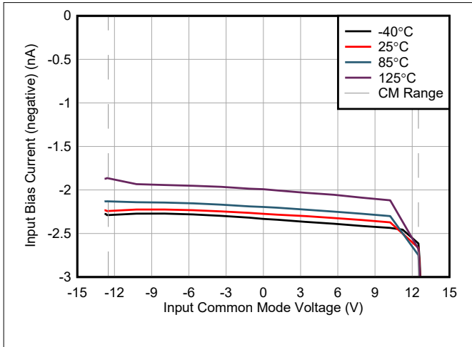
7-31. Negative Input Bias Current vs Common-Mode Voltage
