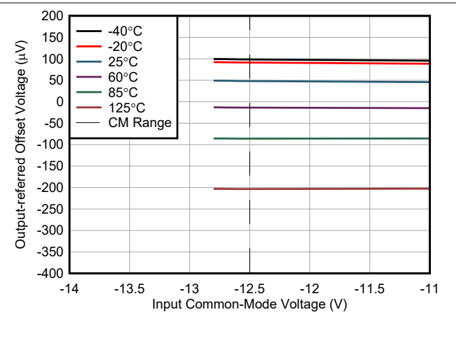
7-36. Offset Voltage vs Negative Common-Mode Voltage
