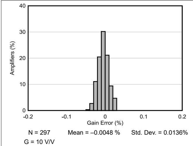
7-13. Typical Gain Error Distribution at G = 10 V/V
