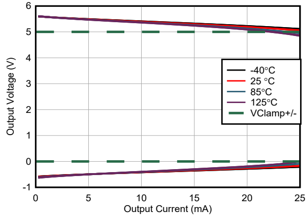
8-13. Output Voltage With Output Clamping Enabled
