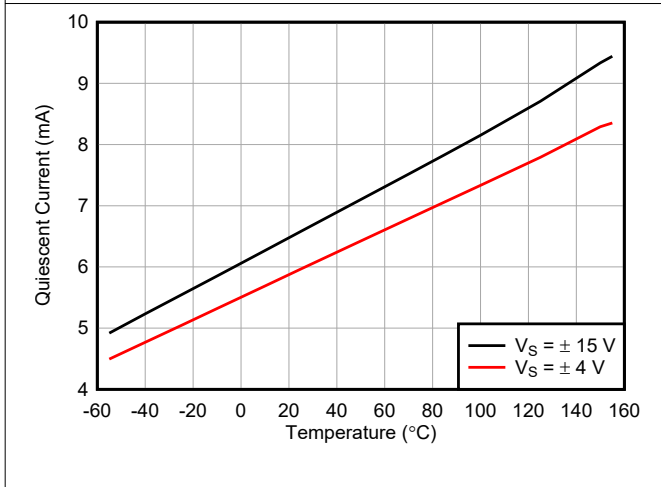
7-33. Quiescent Current vs Temperature
