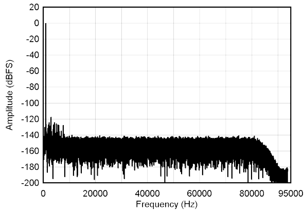
9-12. Noise Performance FFT Plots with Wideband Filter for G = 0.2 V/V
