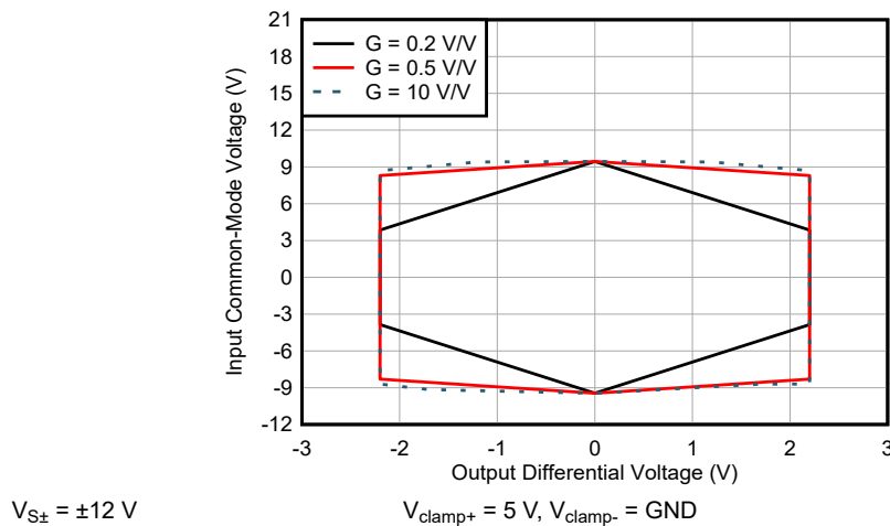
8-9. Input Common-Mode Voltage vs Output Voltage With Output Clamping
