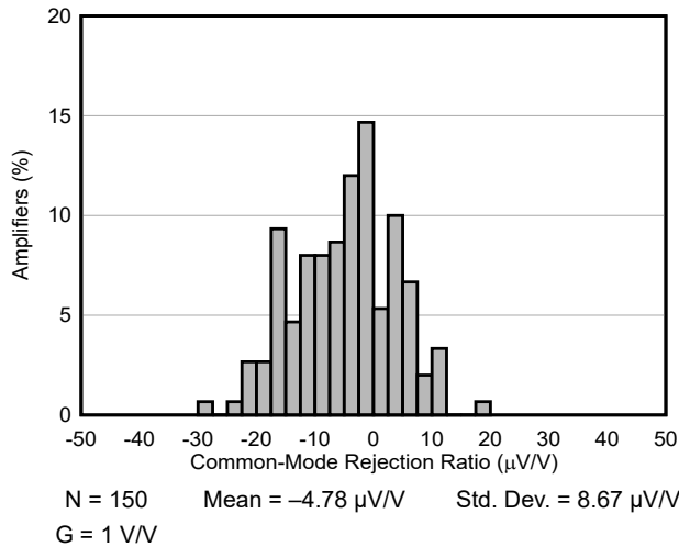
7-9. Typical CMRR Distribution at G = 1 V/V
