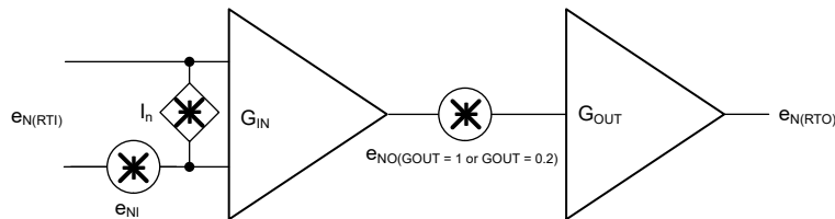
8-14. Simplified Noise Model for the INA851
