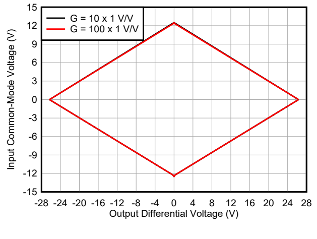
8-8. Input Common-Mode Voltage vs Output Voltage, High Gains
