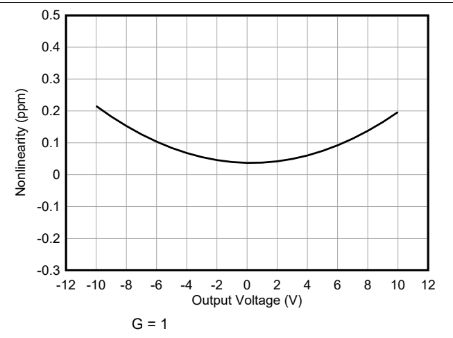
7-34. Gain Nonlinearity, G = 1
