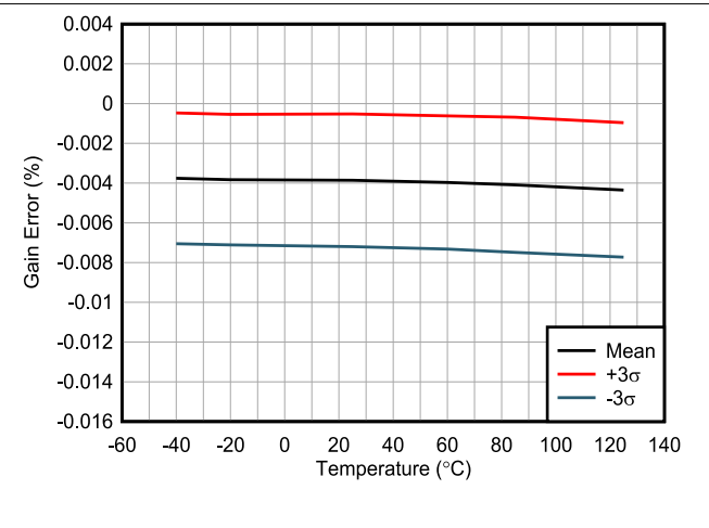
7-32. Gain Error vs Temperature
