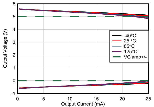
7-38. Positive Output Voltage Swing vs Output Current
