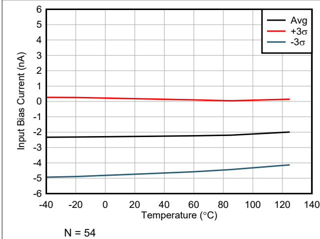
7-15. Input Bias Current vs Temperature
