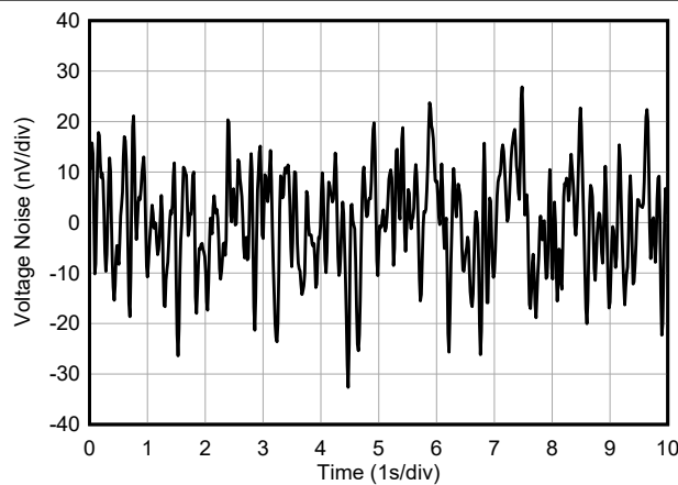
7-27. 0.1-Hz to 10-Hz RTI Voltage Noise
