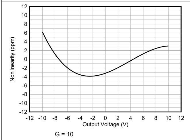
7-35. Gain Nonlinearity, G = 10
