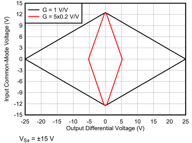
8-6. Input Common-Mode Voltage vs Output Voltage, Unity-Gains
