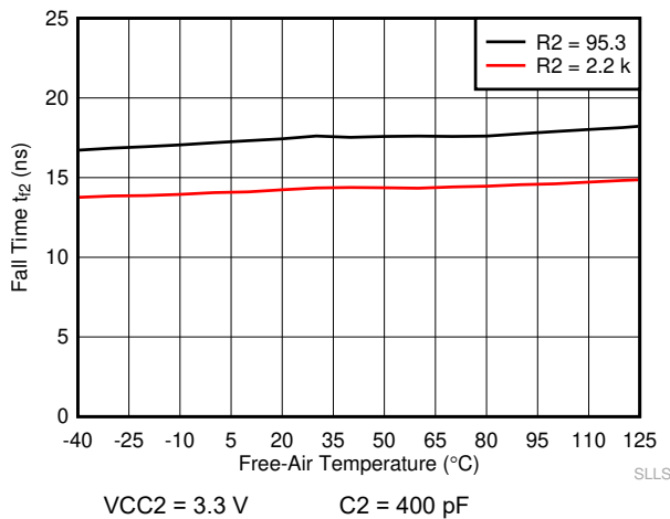
Figure 6-11. Side 2: Output Fall Time vs Free-Air Temperature
