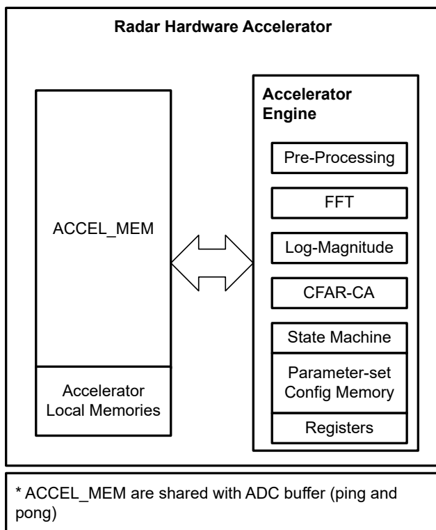
8-6. HWA 1.2 Functional Block Diagram
