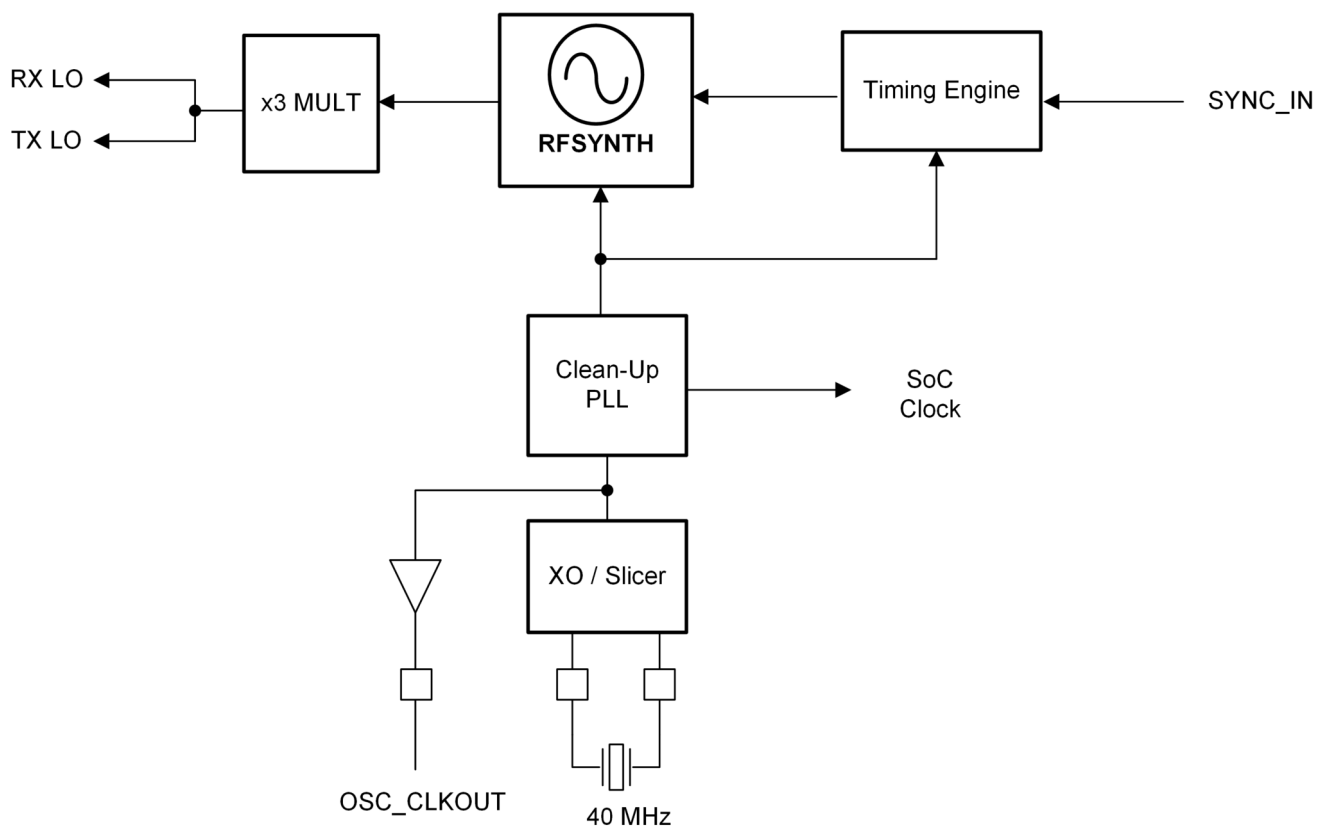
Figure 8-2. Clock Subsystem
