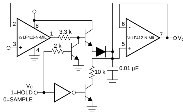
☒ 29. Single-Supply Sample and Hold
