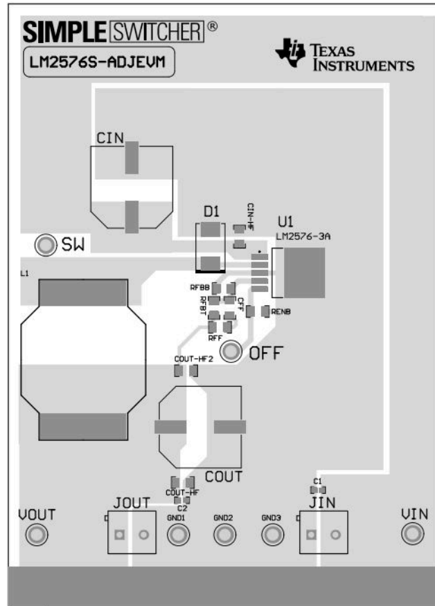
8-11. LM2576xx Layout Example
