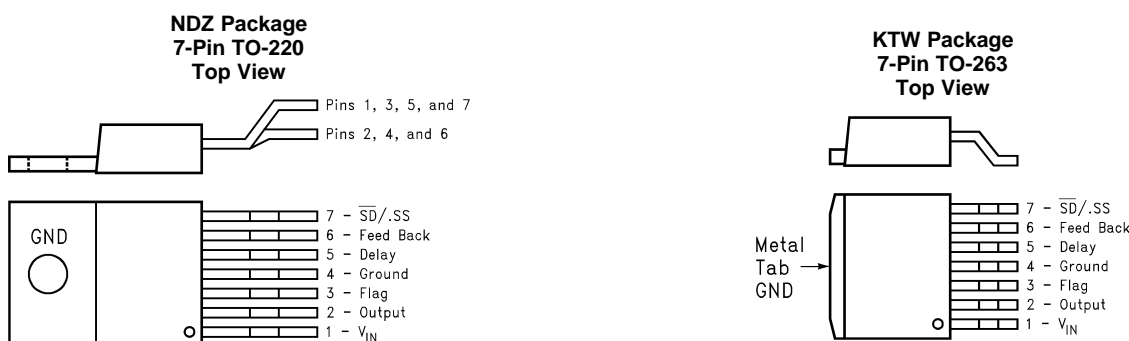
Pin Functions (1)
