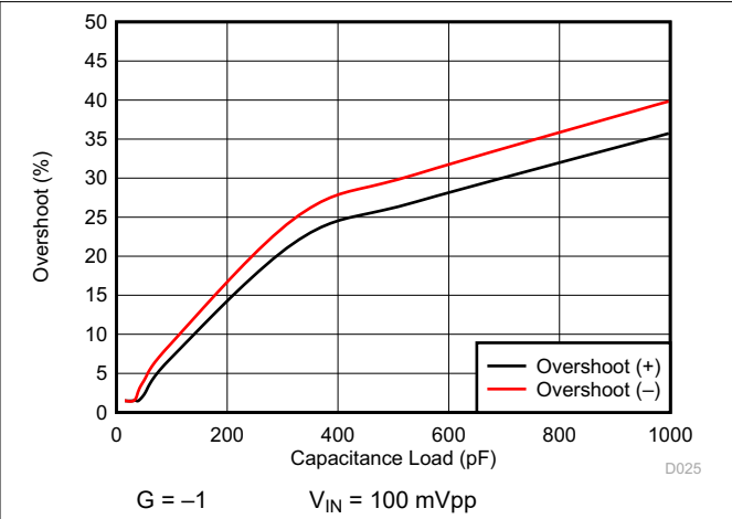
6-19. Small Signal Overshoot vs Capacitive Load
