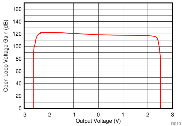
6-4. Open-Loop Gain vs Output Voltage
