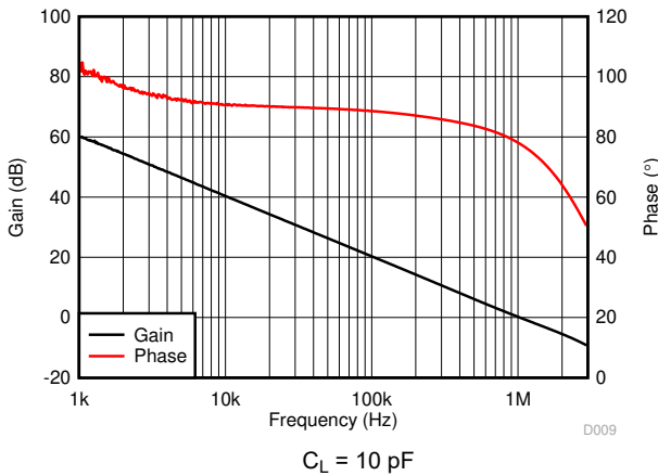
6-3. Open-Loop Gain and Phase vs Frequency
