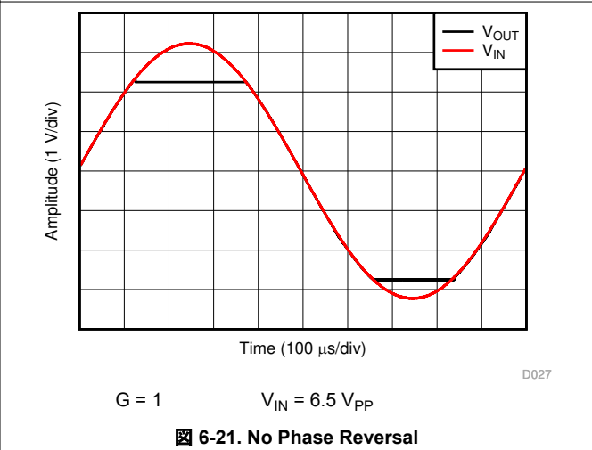
Figure 6-21. No Phase Reversal
