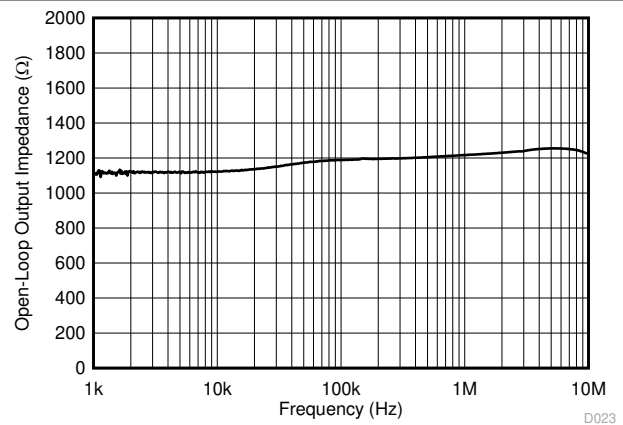
6-17. Open-Loop Output Impedance vs Frequency
