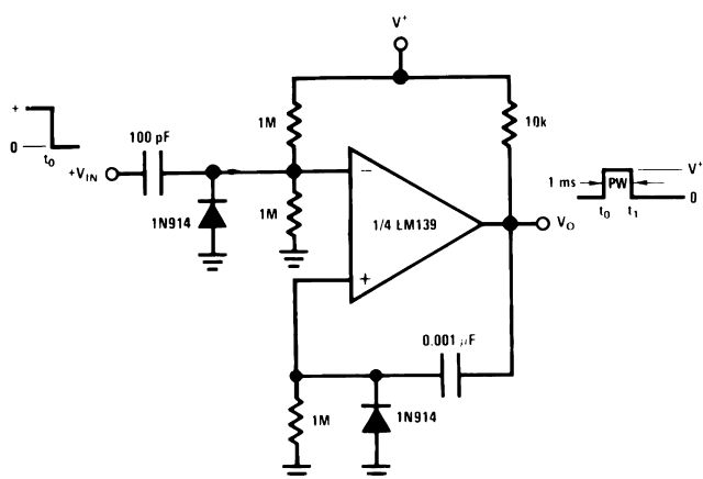
Figure 12. One-Shot Multivibrator ( V_+ = 15\text{ V}_{\text{DC}} )
