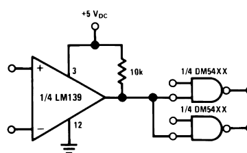
Figure 9. Driving TTL ( V_+ = 5\text{ V}_{\text{DC}} )
