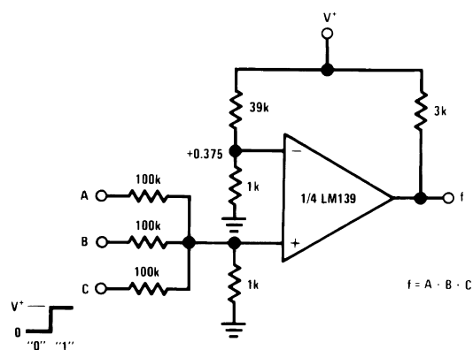
Figure 10. AND Gate ( V_+ = 5\text{ V}_{\text{DC}} )
