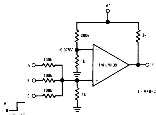
Figure 11. OR Gate ( V_+ = 5\text{ V}_{\text{DC}} )
