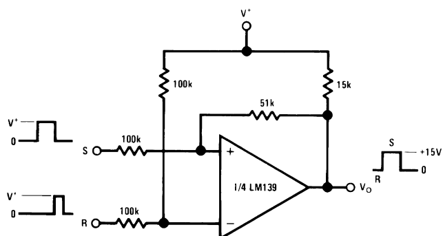
Figure 13. Bi-Stable Multivibrator ( V_{+} = 15\text{ V}_{\text{DC}} )
