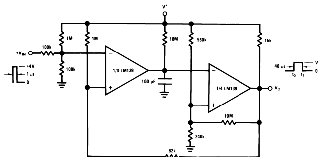
Figure 14. One-Shot Multivibrator With Input Lockout ( V_{+} = 15 V_{DC} )
