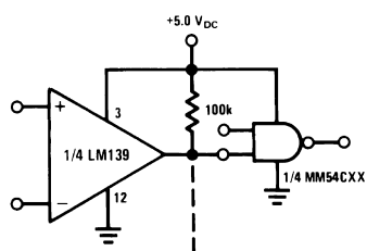
Figure 8. Driving CMOS ( V_+ = 5\text{ V}_{\text{DC}} )
