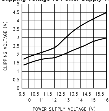
Figure 59. R_L = 8\Omega , BTL operation, f_{IN} = 1\text{kHz} at (from top to bottom at 12V): positive signal swing, negative signal swing
