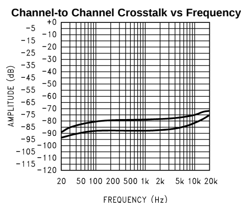
Figure 44. V_{DD} = 9.6V , R_L = 8\Omega , P_{OUT} = 1W , SE operation, at (from top to bottom at 1kHz): V_{INB} driven, V_{OUTA} measured; V_{INA} driven, V_{OUTB} measured
