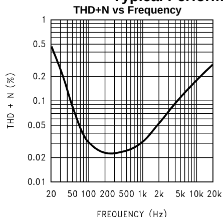
Figure 11. V_{DD} = 12V , R_L = 4\Omega , SE operation, both channels driven and loaded (average shown), P_{OUT} = 1W , A_V = 1
