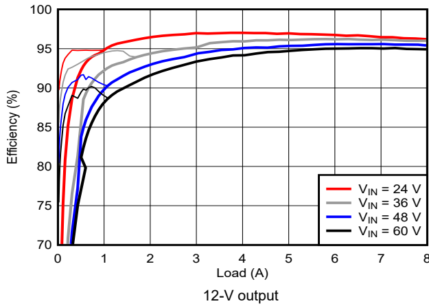
9-19. Efficiency vs. I_{OUT}
