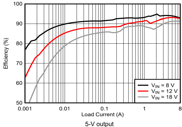
9-7. Efficiency vs I_{OUT} , Log Scale
