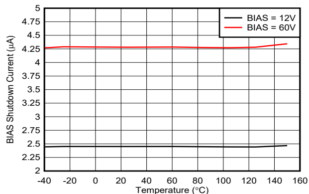
FIG 8-2. BIAS Shutdown Current vs Temperature
