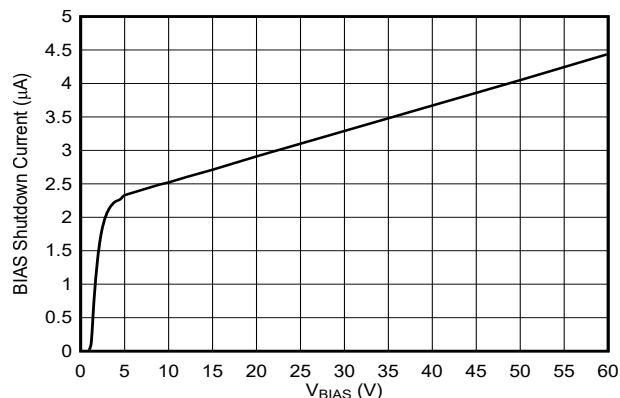
FIG 8-1. BIAS Shutdown Current vs V_{BIAS}
