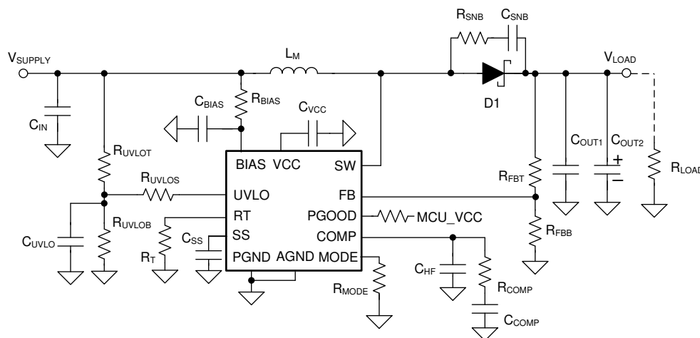
10-1. Typical Boost Converter Circuit with Optional Components
