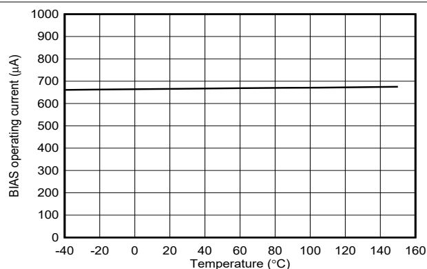
FIG 8-3. BIAS Operating Current vs Temperature
