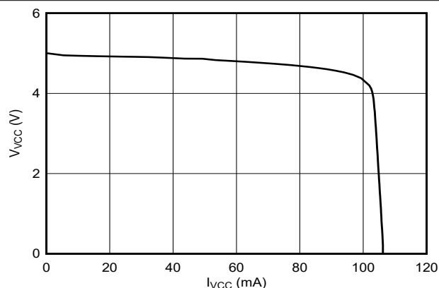
FIG 8-5. V_{VCC} vs I_{VCC}
