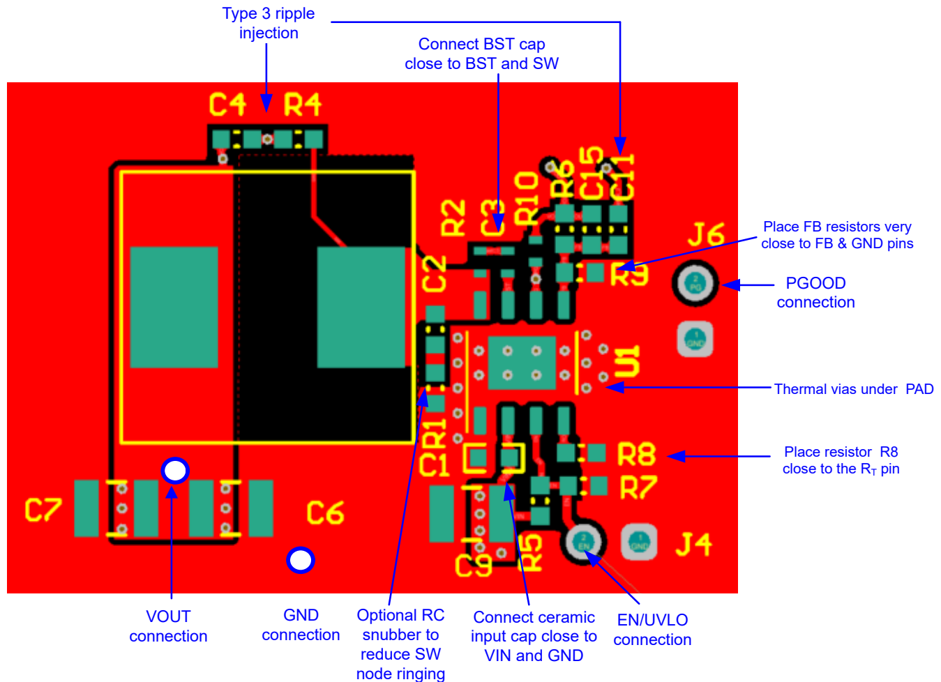
☒ 8-41. LM516x PCB Layout Example for DDA package
