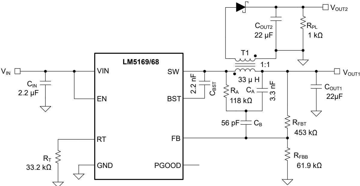
図 8-1. Example Fly-Buck™ Converter Application Circuit
