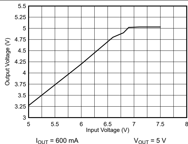
9-31. Drop-Out Response
