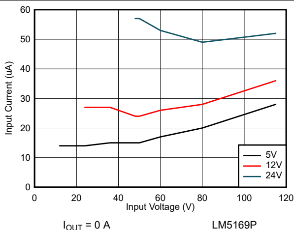
9-30. No-Load Input Supply Current
