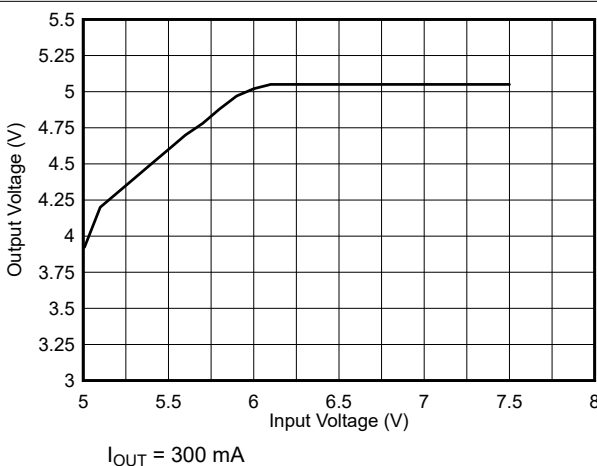
9-32. Drop-Out Response
