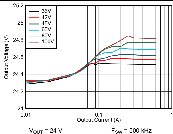
FIG 9-20. Line and Load Regulation: V_{OUT} = 24\text{ V}
