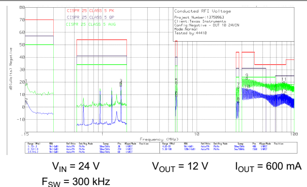
9-37. Conducted EMI (Negative Rail)
