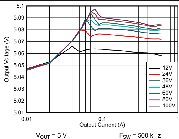
FIG 9-18. Line and Load Regulation: V_{OUT} = 5\text{ V}
