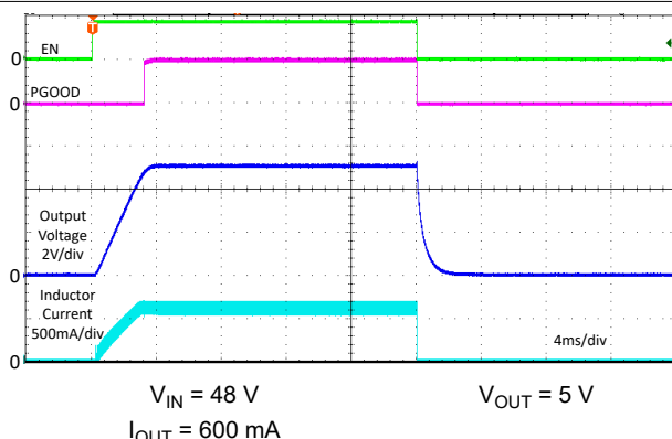
9-29. Typical Start-up Waveforms
