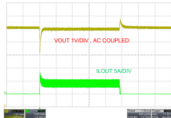
Figure 9-11. Load Transient Response, V_{SUPPLY} = 48V , PFM, 0A to 4A
