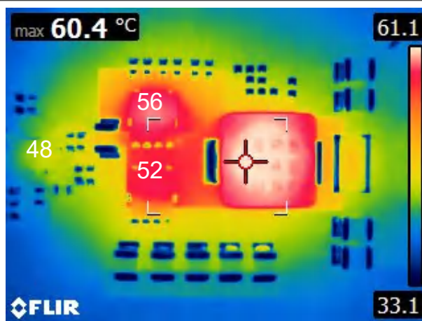
Figure 9-13. V_{SUPPLY} = 48V , I_{LOAD} = 8A , T_A = 25^{\circ}C , No Airflow
