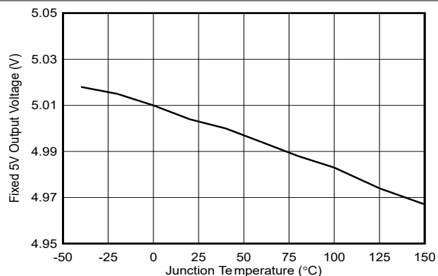
Figure 6-7. Fixed Output Voltage vs Temperature, V_{OUT} = 5V
