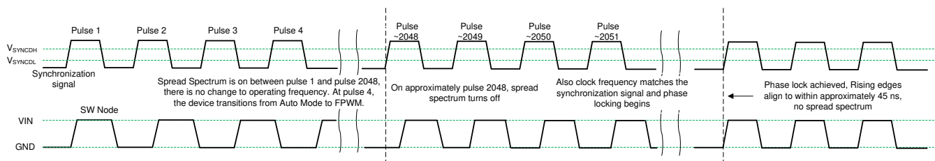
FIG 8-4. Synchronization Process
