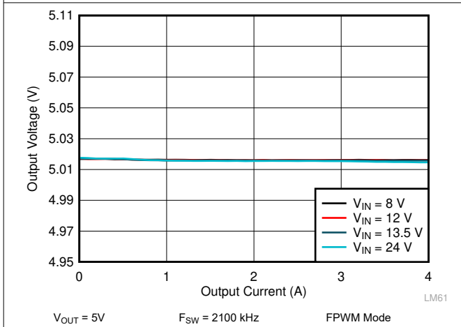
图 9-15. LM61440 Load and Line Regulation
