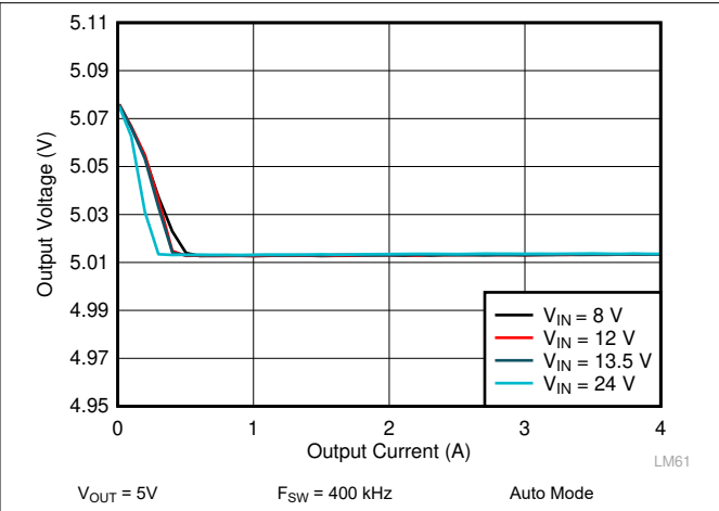
图 9-12. LM61440 Load and Line Regulation
