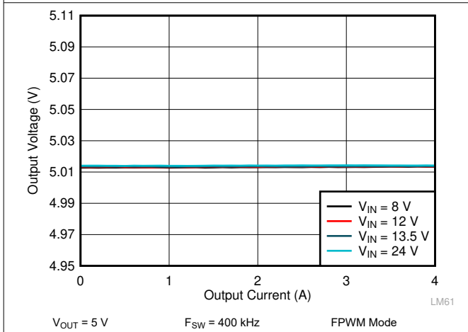
图 9-13. LM61440 Load and Line Regulation
