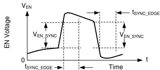
FIG 8-3. Typical SYNC/EN Waveform
