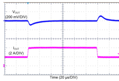
9-30. LM61440 Load Transient
