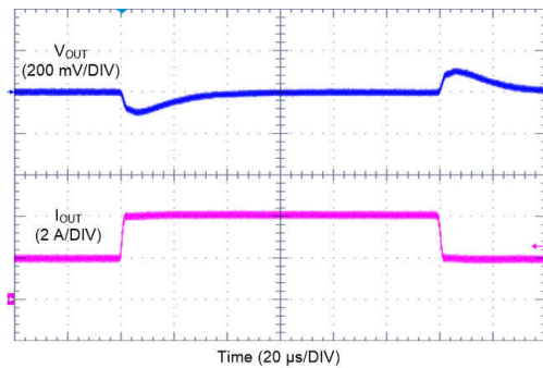
9-32. LM61440 Load Transient
