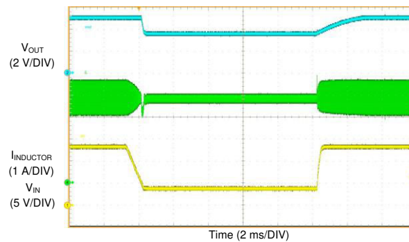
8-9. Recovery From Dropout
