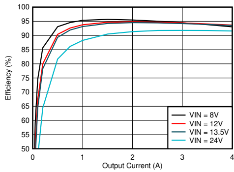
图 9-5. LM61440 Efficiency
