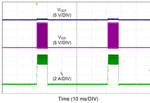
9-29. LM61440 Short Circuit Performance
