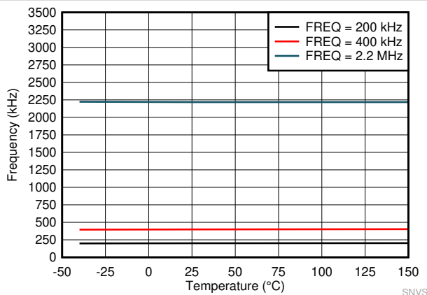
8-5. Switching Frequency Set by RT Resistor
