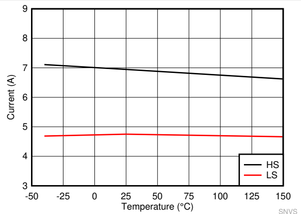
8-4. LM61440-Q1 High-side and Low-side Current Limits
