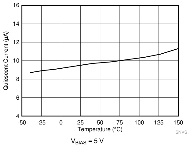
8-1. Non-Switching Input Supply Current
