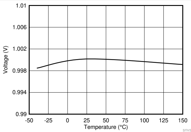
8-3. Feedback Voltage
