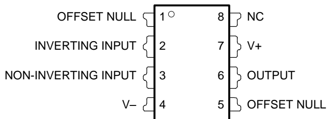
P Package 8-Pin PDIP Top View
