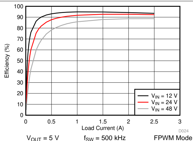
Figure 36. LM76002 Efficiency
