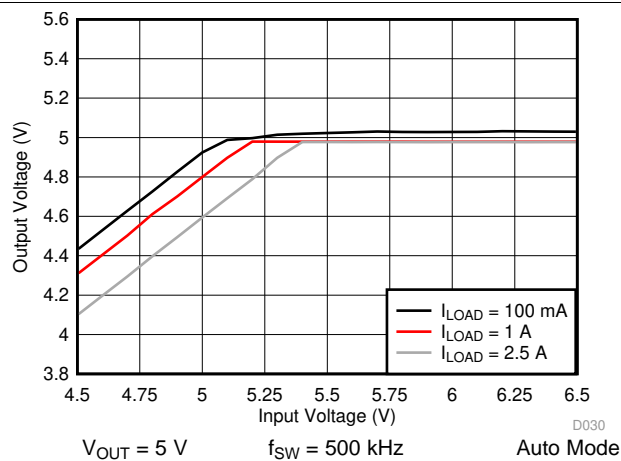
图 55. LM76002 Dropout Curve
