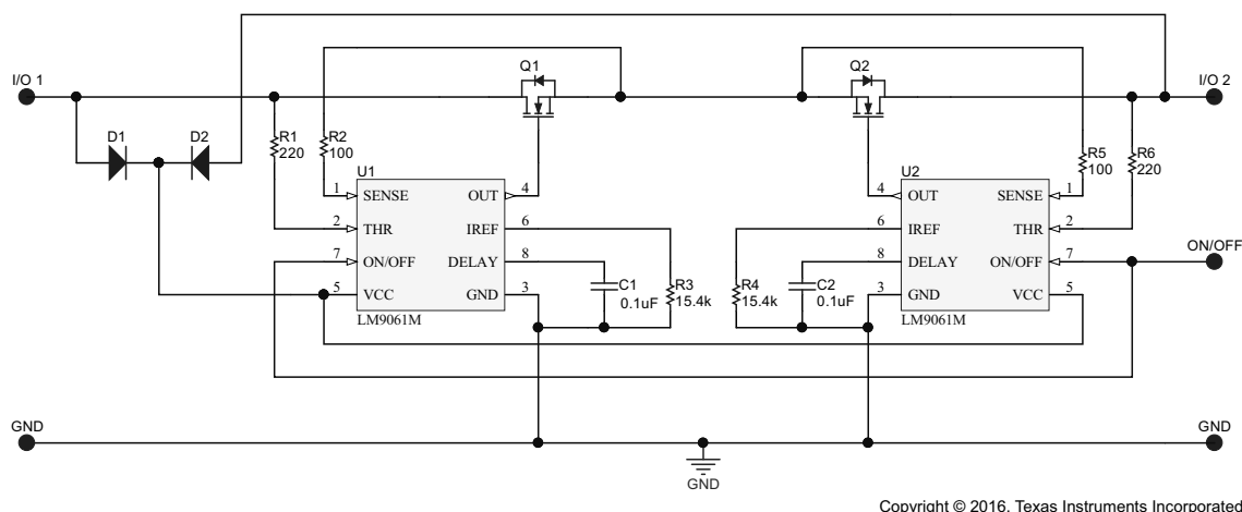
Figure 24. Bidirectional Switch Including Reverse OCP
