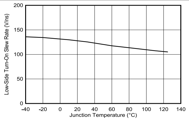
Fig 5-10. Low-Side Turn-On Slew Rate vs Junction Temperature
