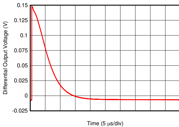
6-25. Turn-Off Time
