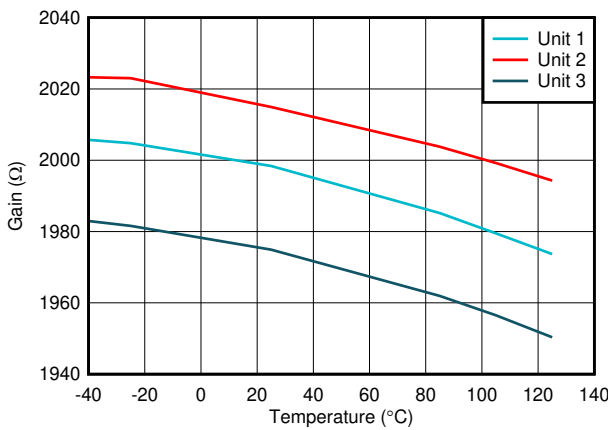
Gain = 2 kΩ
