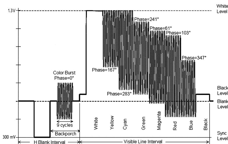
Figure 51. Input Video Signal After DC Restore Clamp
