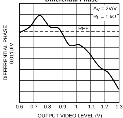
Differential Phase
