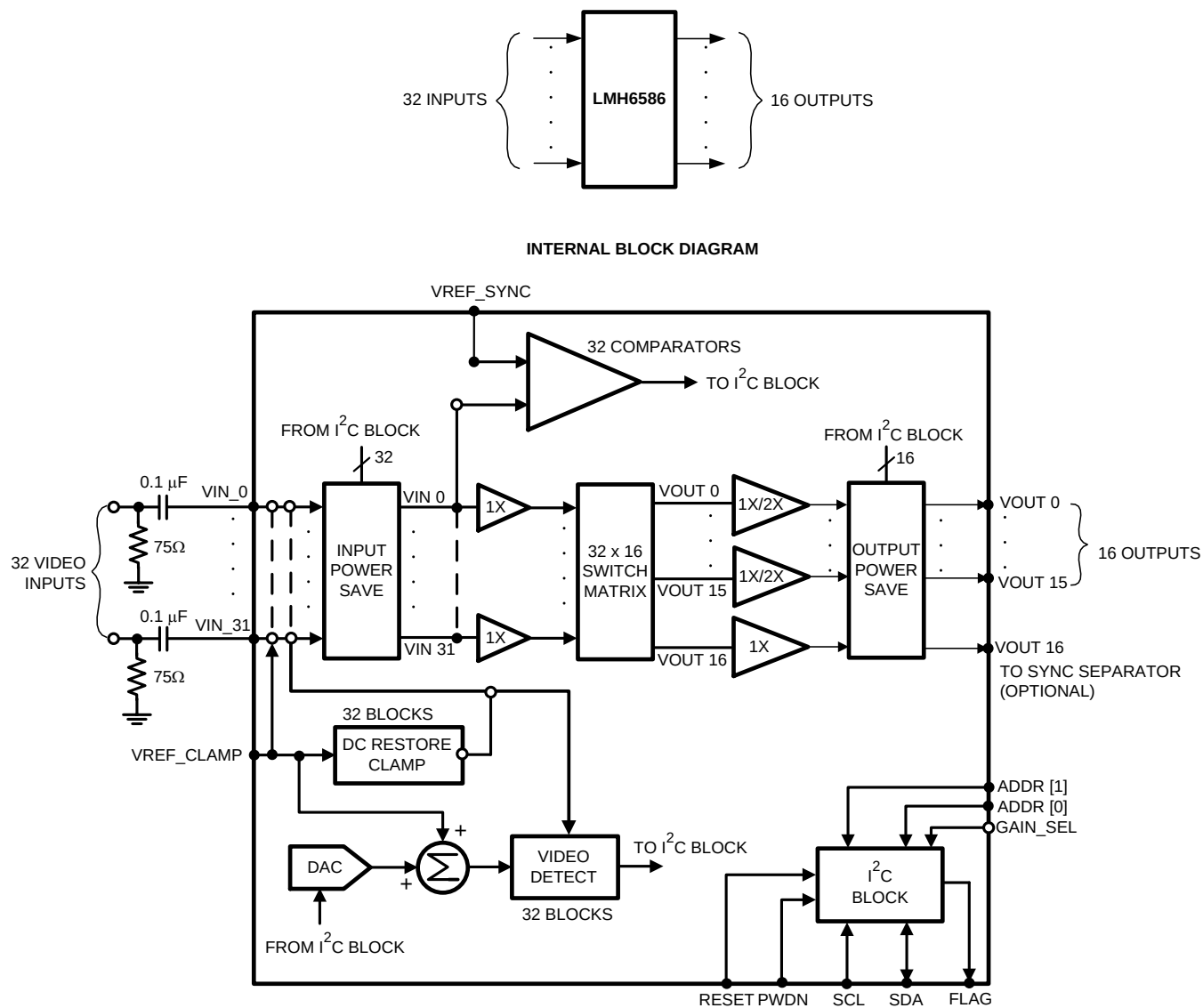
Figure 1. Functional Diagram
