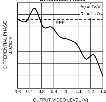
Differential Phase
