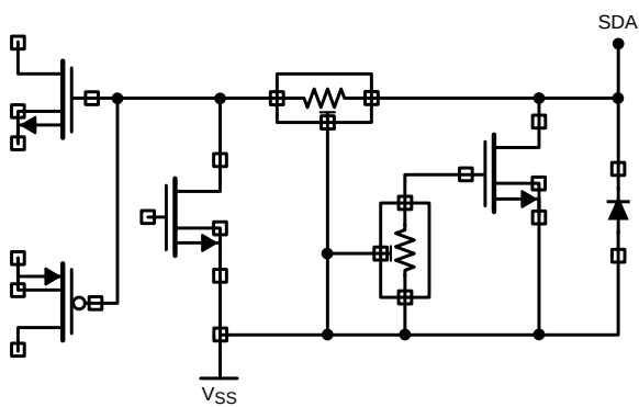
I²C DATA CIRCUIT DIAGRAM
