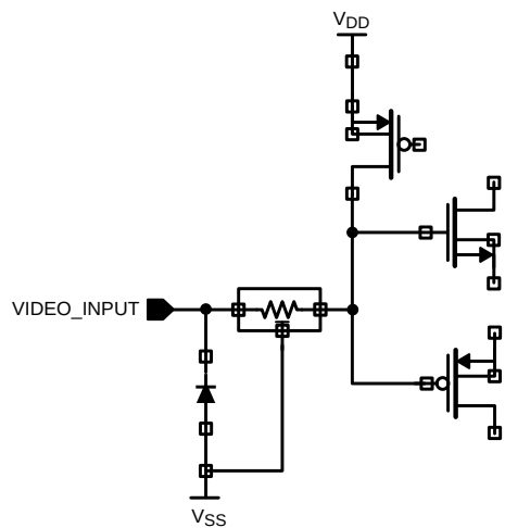
VIDEO INPUT CIRCUIT DIAGRAM
