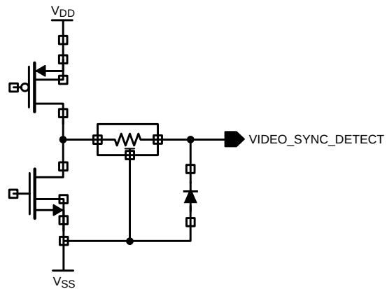
VIDEO SYNC DETECT CIRCUIT DIAGRAM
