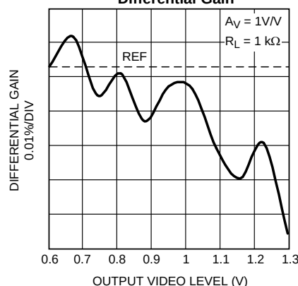
Differential Gain
