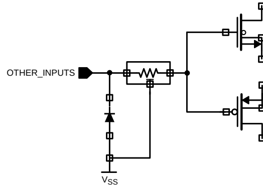
OTHER INPUT CIRCUIT DIAGRAM
