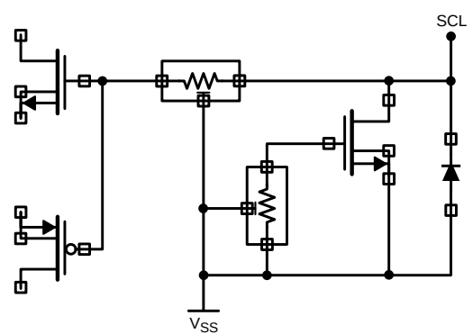
I²C CLOCK CIRCUIT DIAGRAM
