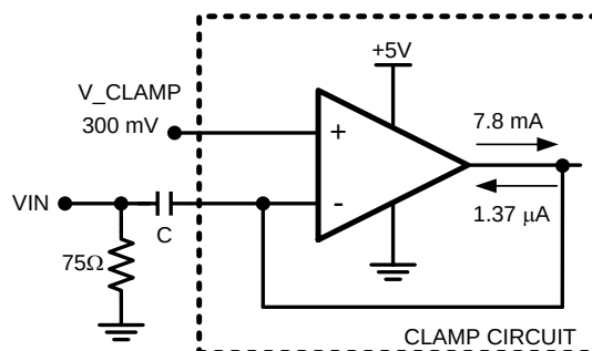
Figure 52. Clamp Circuit
