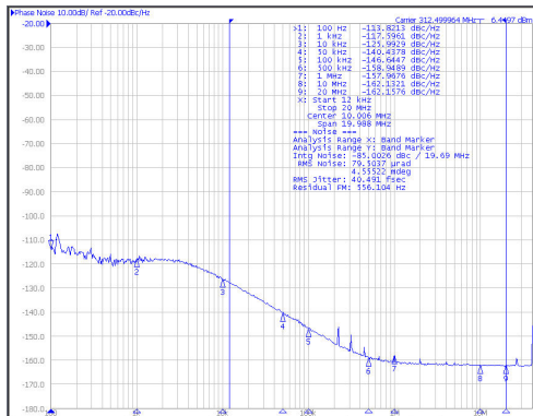
图 6-8. 312.5MHz HSDS Output From BAW APLL
