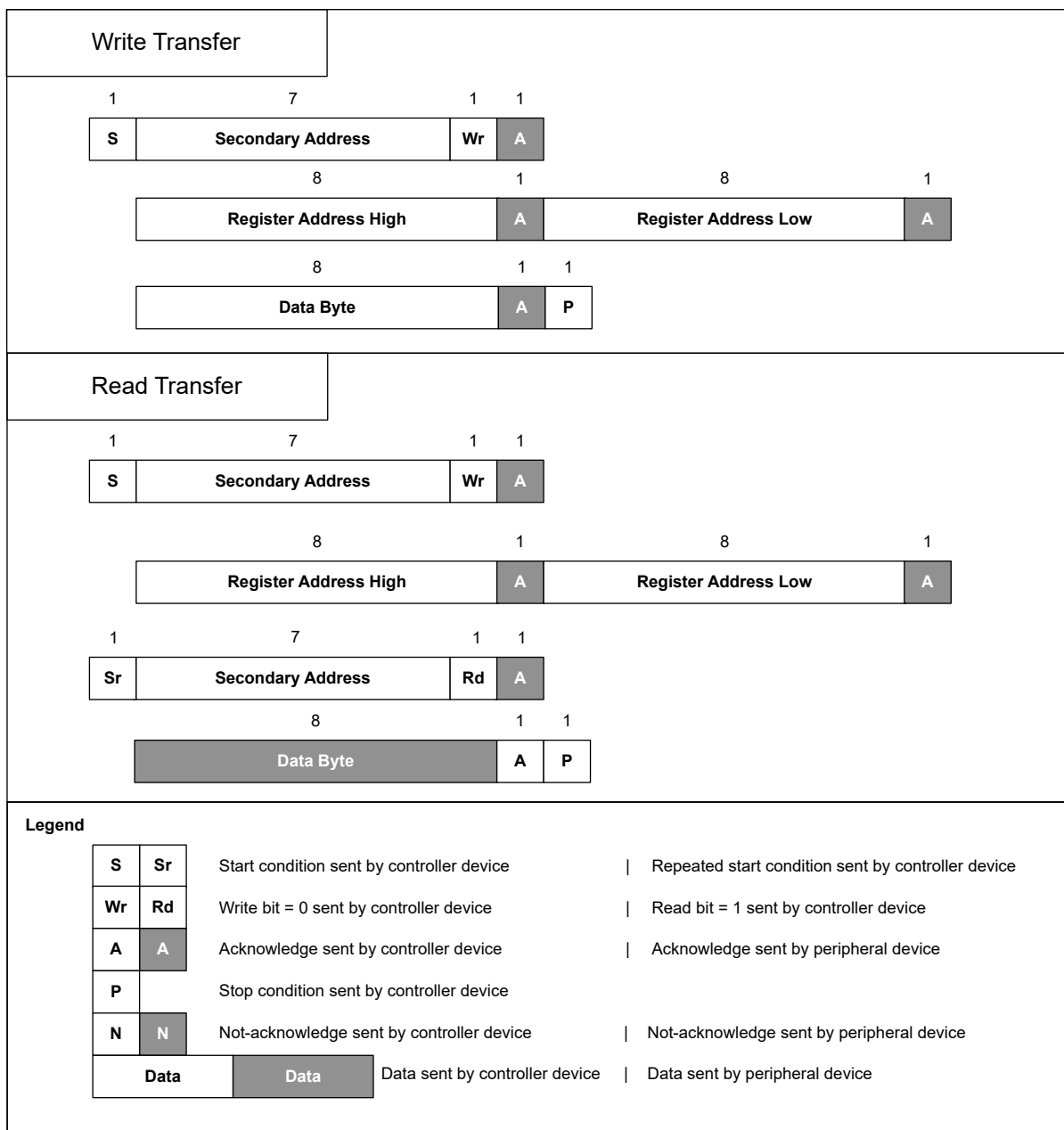
図 8-45. I 2 C Byte Write and Read Transfers
