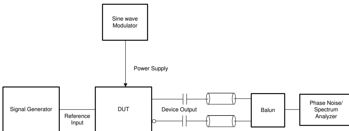
図 7-8. HCSL Output Phase Domain Test Configuration
