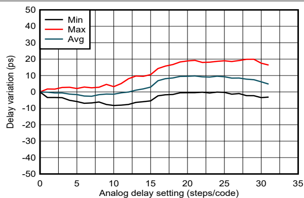
図 6-22. SYSREF/1PPS Delay Linearity vs. Analog Delay Code 3
