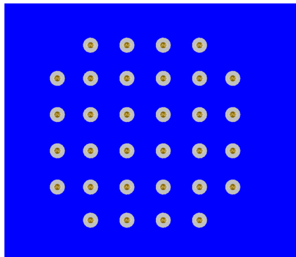
図 9-6. PCB Layout Example for LMK5B33414, Bottom Layer
