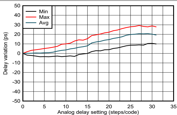
図 6-21. SYSREF/1PPS Delay Linearity vs. Analog Delay Code 2
