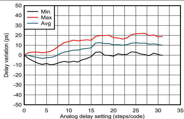
図 6-24. SYSREF/1PPS Delay Linearity vs. Analog Delay Code 5
