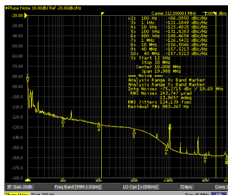
図 6-12. 312.5MHz HSDS Output From APPL2
